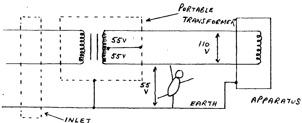
v) Isolating transformer with secondaries tapped to earth
