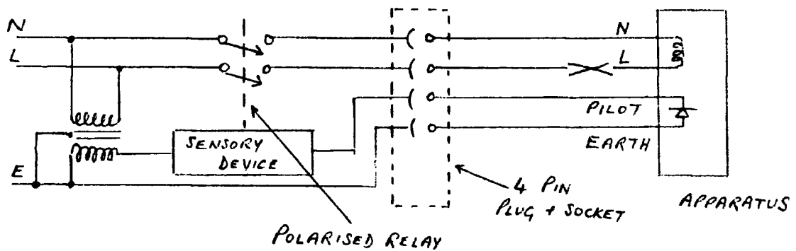
iii) Circulating-current earth monitoring
