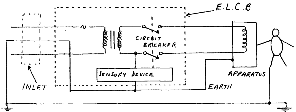
i) Voltage-operated, isolation type
