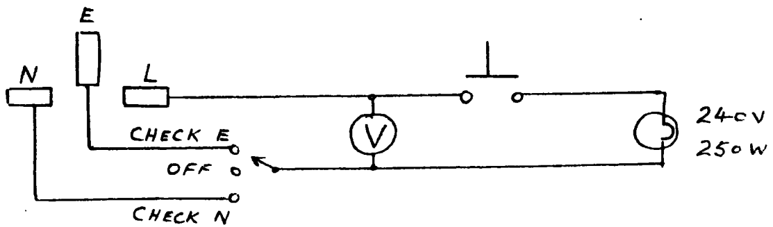
Diagram 8.1 : Test circuit for Mains Socket (8.3.3)
