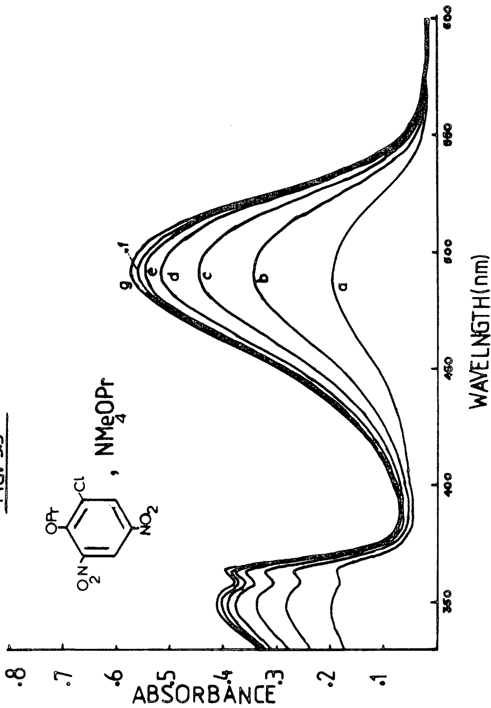
FIGURE 3.5 Visible spectra of 1-propoxy-2,4-dinitro-6-chlorobenzene ( 4 \times 10^{-5} M) with tetramethylammonium propoxide in propan-1-ol at 25^\circ . The change with time is a \rightarrow e . [BASE] = 1 \times 10^{-2} M.
