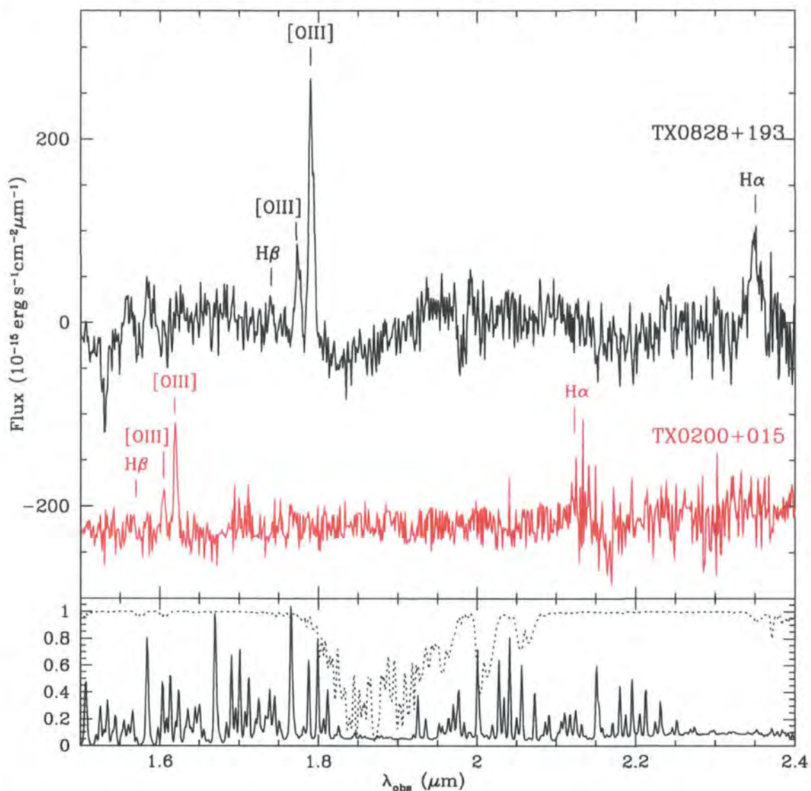
Figure 8.1: Collapsed spectra of both radio galaxies in our sample from the UIST IFU observations. TX0200+015 is offset in flux scale for clarity. We mark the positions of the strongest emission features. We also show a (scaled) sky spectrum (bottom pannel), as well as the Mauna Kea atmospheric transmission (dashed line).
