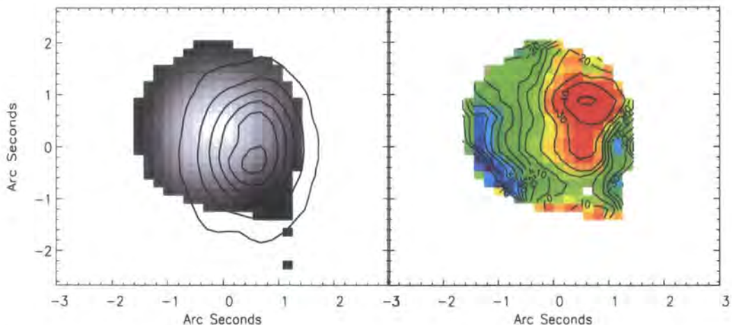
Figure 2.6: Left: The UV continuum intensity (colour scale) with the continuum from the older stellar population overlaid as contours. Right: Two dimensional velocity field of the galaxy derived from the [OII] emission line. The galaxy shows a shear across the galaxy with peak-to-peak velocity difference of 100 \pm 20 \text{ km s}^{-1} .
