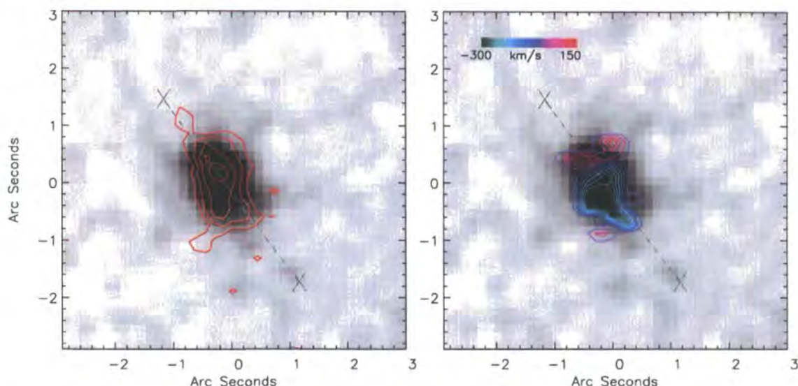
Figure 8.2: Left: The ISAAC K' image of TX0200+015 ( z=2.23 ) with the [OIII] \lambda 5007 emission line intensity overlaid as contours. Right: The ISAAC K' image of TX0200+015 with the velocity field derived from the [OIII] \lambda 5007 emission line overlaid. The dashed line shows the orientation of the radio lobes and the crosses mark their location (Carilli et al., 1997). It is clear that the velocity field follows the direction of the radio jet
