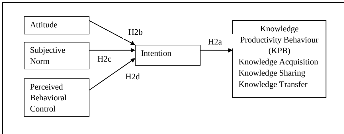
Figure 4.33 Hypotheses H2a-e
