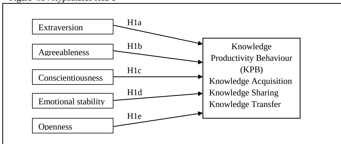
Figure 4.14 Hypotheses H1a-e
