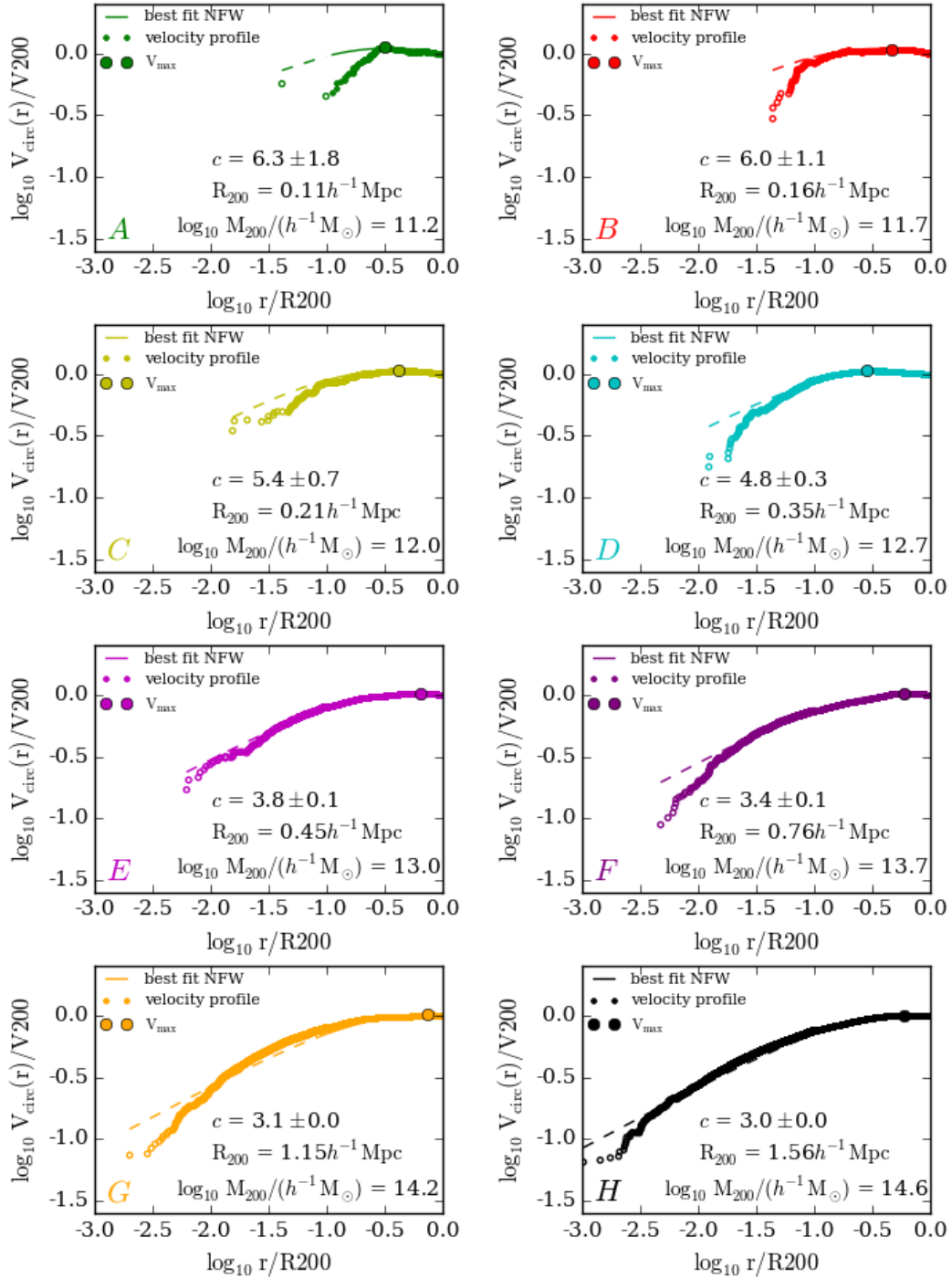
Figure 6.8: Circular velocity profiles for the example haloes given in Fig. 6.4. The large circle in each panel shows the maximum circular velocity in the halo ( V_{\max} ). The solid curves show the expected circular velocity profile from the halo concentration as found in §6.4.
