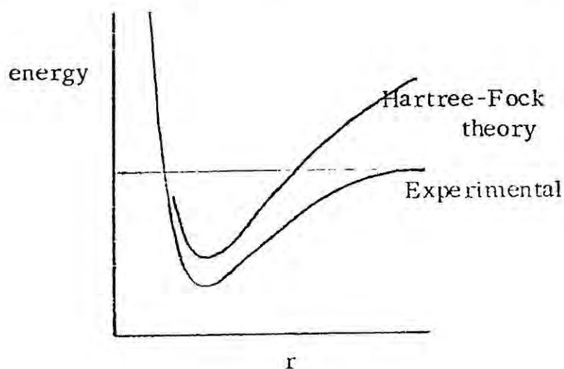
Fig 1.2 Behaviour of Hartree Fock energy and experimental energy as functions of internuclear distance
