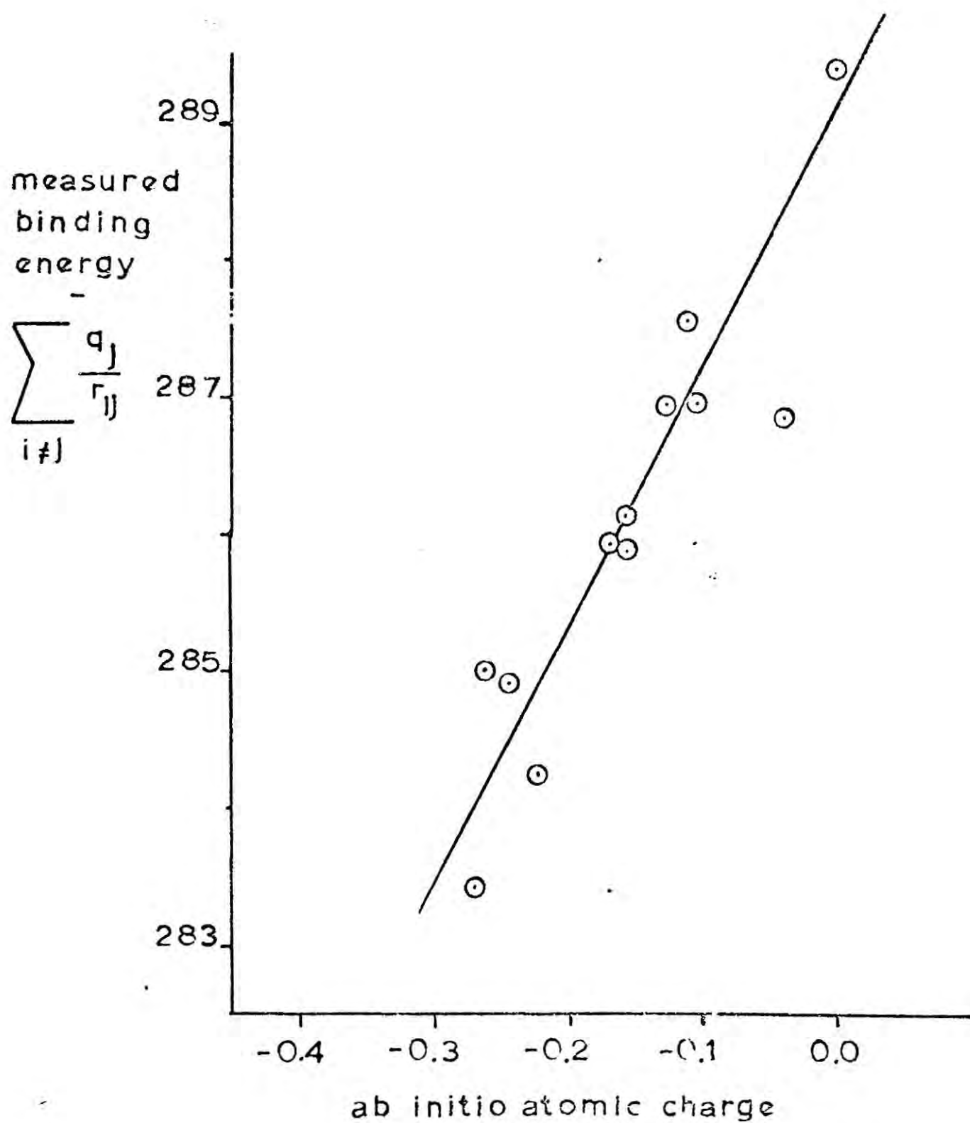
Fig. 4.2(a). Measured C_{1s} binding energies corrected for Madelung potentials against ab initio atomic charge.
