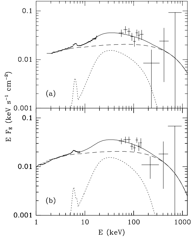
Figure 4.2: The average continuum spectrum of unobscured (type 1) AGN from Ginga/OSSE (top panel) and EXOSAT/OSSE (bottom panel) with 2\sigma upper limits. The roll-over at high energies is clearly present (from Gondek et al. 2006).
