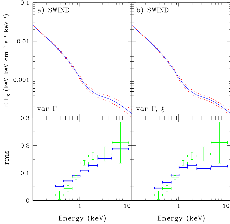
Figure 9.8: As for fig. 9.4 but for a smeared absorption model for the soft excess. (a) shows the rms produced by pivoting the steep spectrum about the peak in seed photon flux at 5kT_{\text{seed}} \sim 0.15 keV without changing the ionization of the absorber. Similarly to fig. 9.6, this linear rise in rms as a function of energy does not match the sharper rise around 0.7 keV seen in the rapid variability. (b) shows that this low energy rise can be matched if the ionization responds to the changes in illumination as this enhances the variability over 0.7–2 keV where the absorption dominates. However, this also predicts that the variability should drop above 2 keV, which is not seen in the data.
