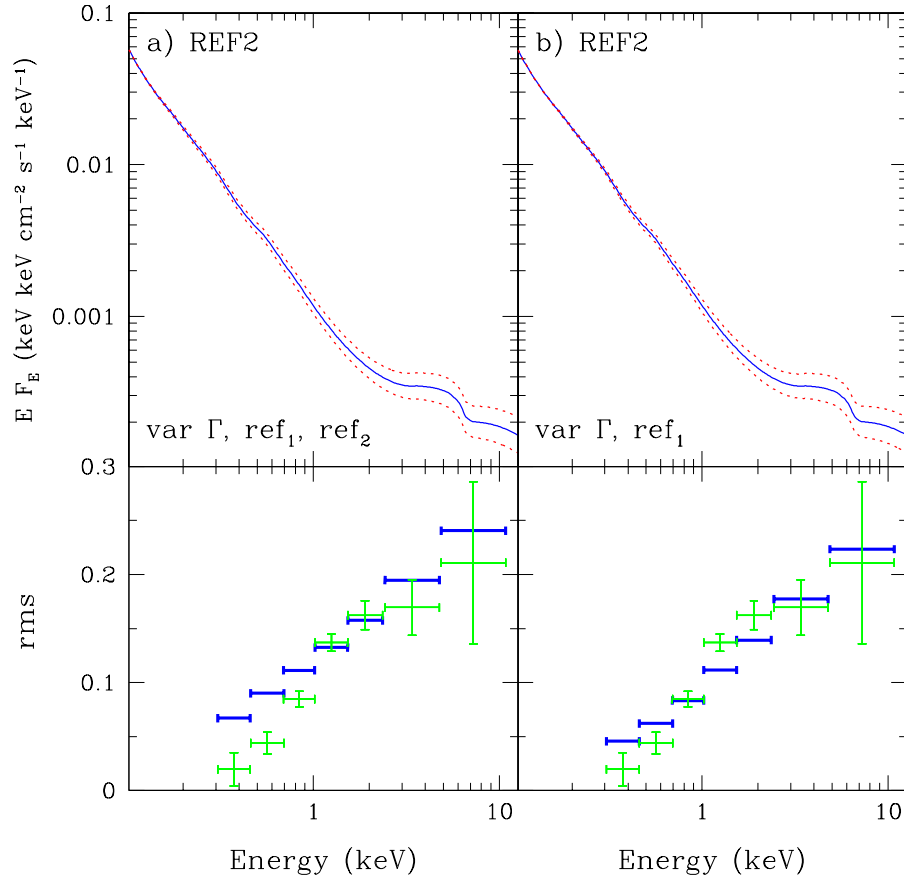
Figure 9.6: As for fig. 9.4 but for the double reflection model for the soft excess. (a) shows the rms produced by pivoting the steep spectrum about the peak in seed photon flux at 5kT_{\text{seed}} \sim 0.15 keV when both reflectors respond to this illumination. This gives a linear rise in rms as a function of energy, which does not match the sharper rise around 0.7 keV seen in the rapid variability. (b) shows that this can be roughly matched if the ionized reflector which contributes mainly at low energies remains constant while the more neutral reflector responds to the spectral pivoting.
