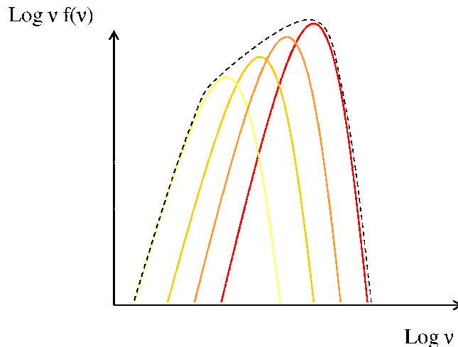
Figure 1.1: The multi-colour disc blackbody, formed from the black-body emission of many annuli with the hottest being those closer to the compact object.
