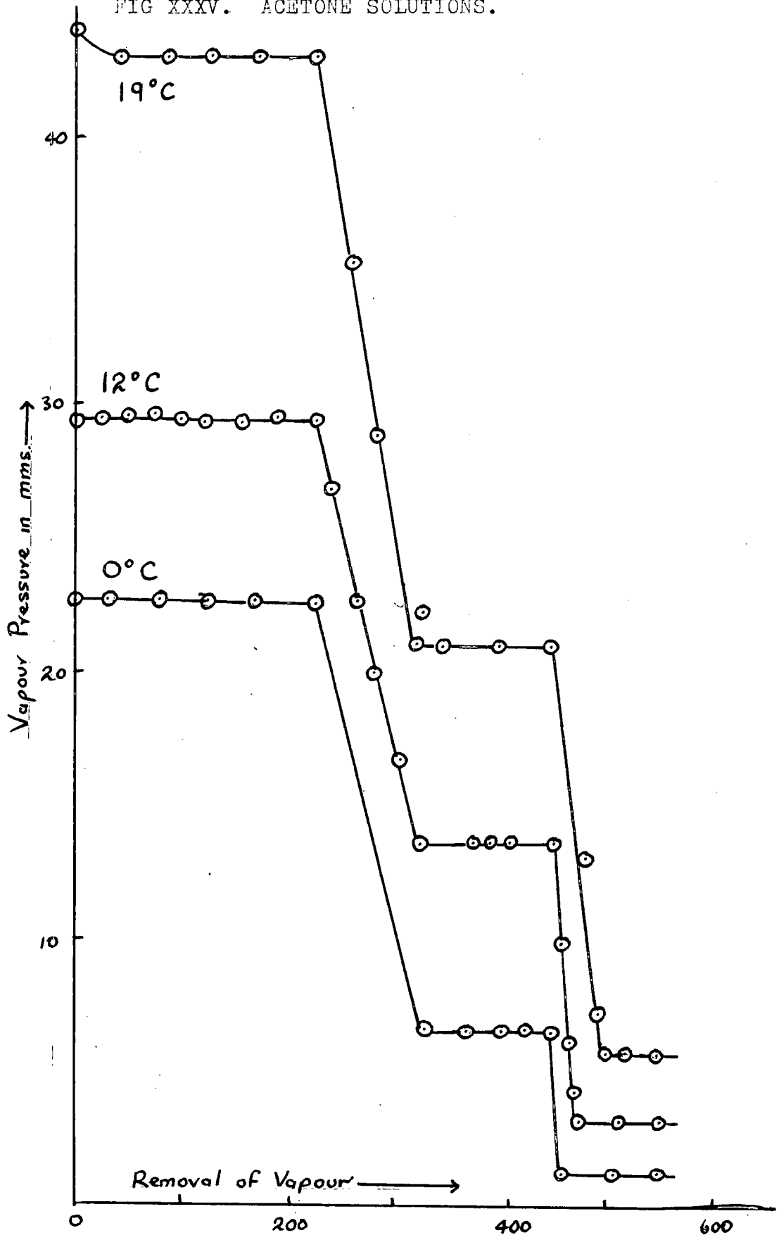
FIG XXXV. ACETONE SOLUTIONS.
