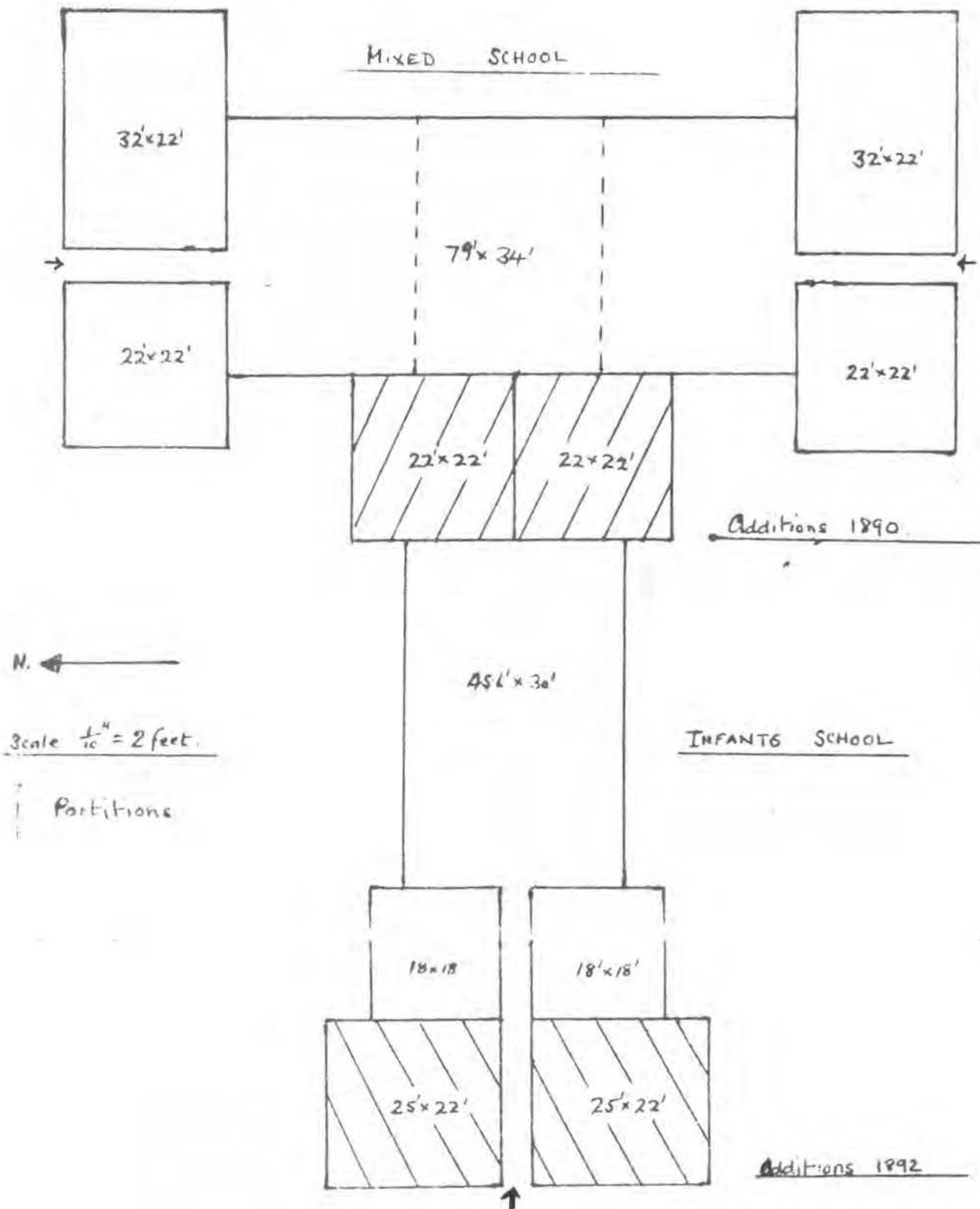
HIGH FELLING BOARD SCHOOLS : PLAN OF ROOMS
