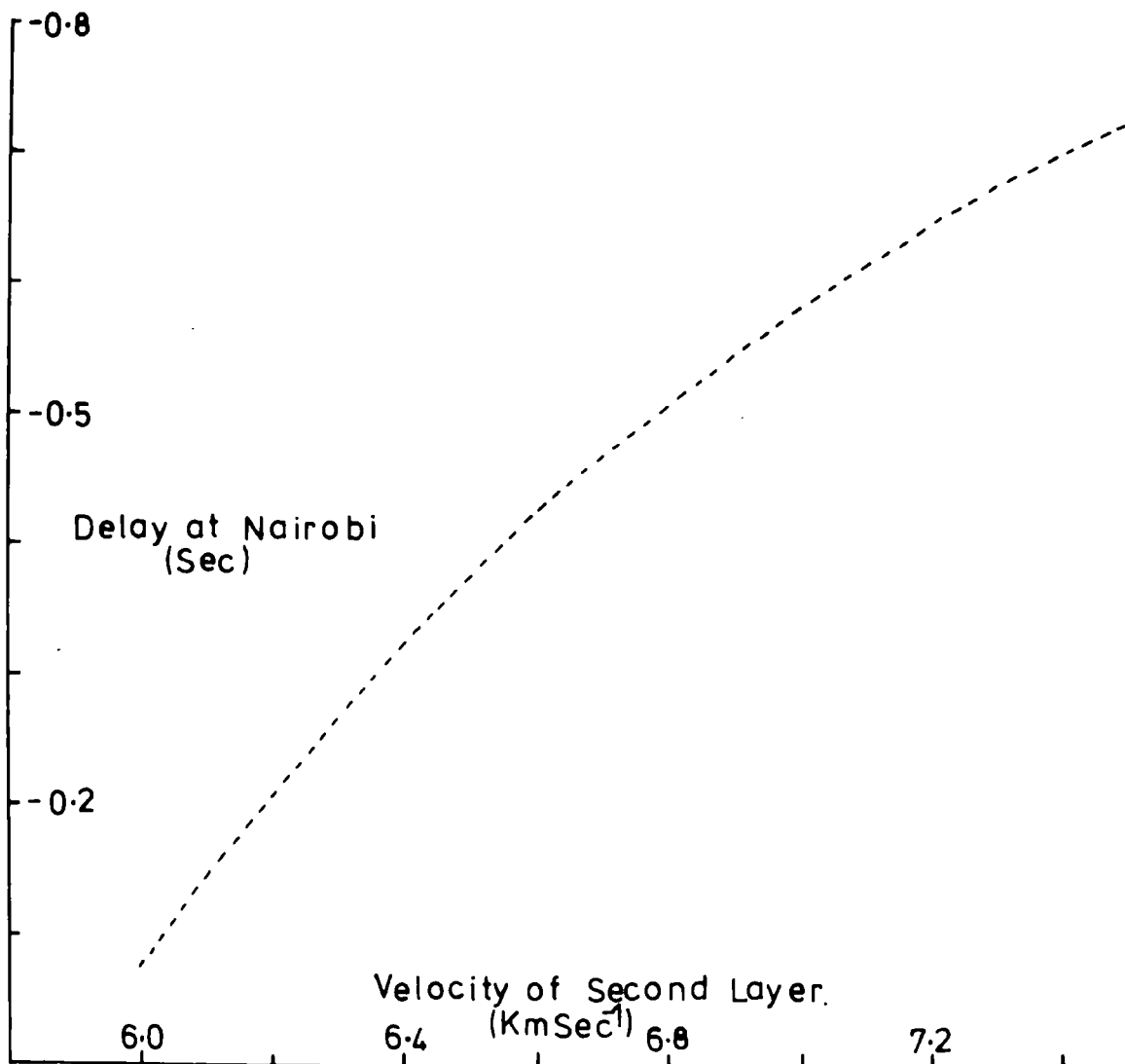
Delay at Nairobi on Events from the Siria Fault Assuming Two Layer Crust in the Gregory Rift.
