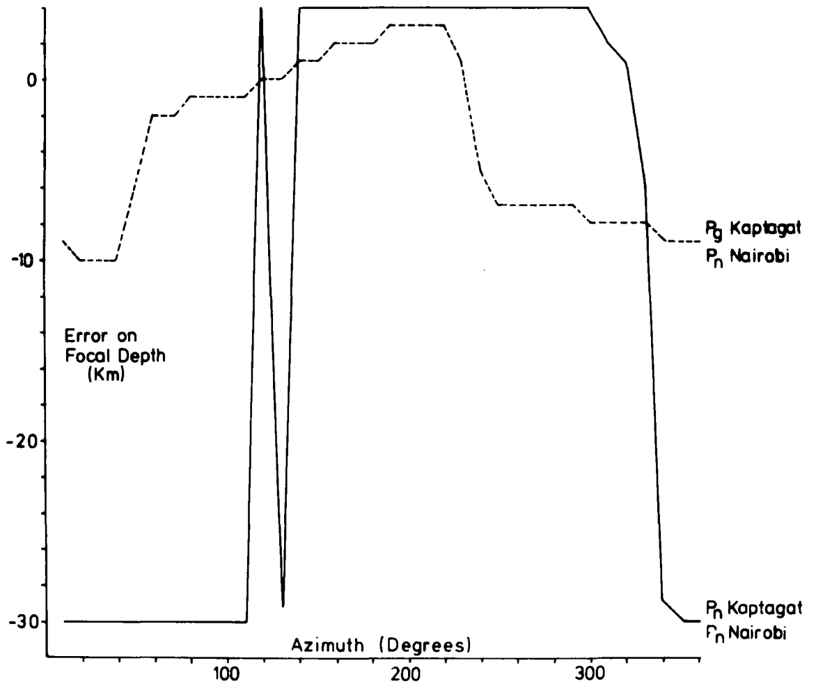
Error on Focal Depth due to an Error of 0.5 Seconds on the Travel Time to Nairobi
