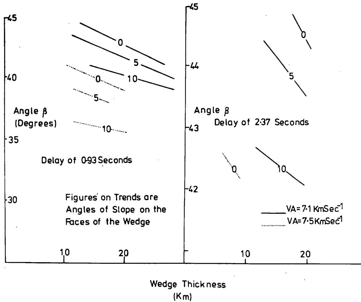
Delay on Moho Arrivals Assuming a Two Layer Model for the Gregory Rift
