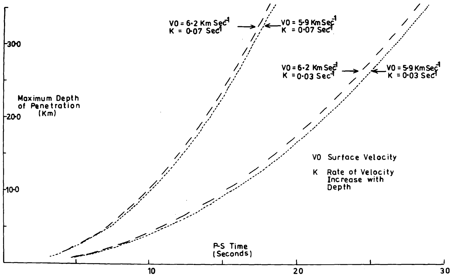
P-S Time for a Surface to Surface Travel Path Through a Velocity Increase with Depth
