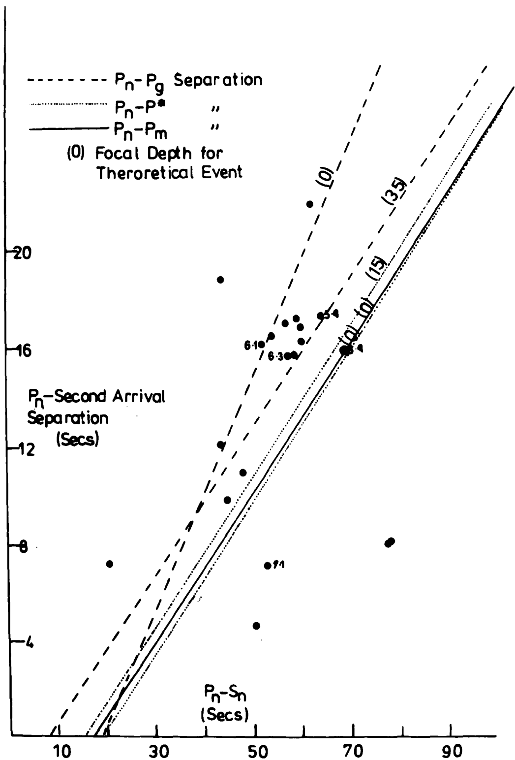
Theoretical Separation of P_n and Second P Arrivals Against P_n - S_n Fig 3:18
