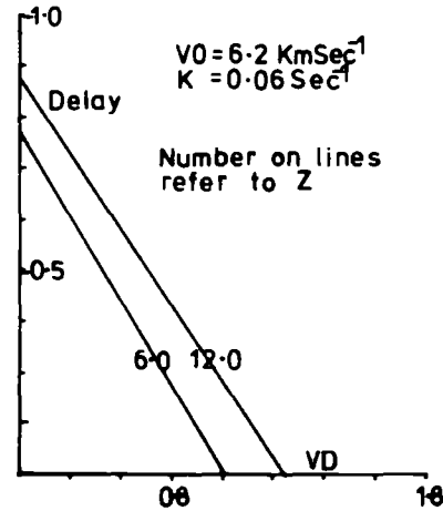
Delay at Nairobi on Events from the Siria Assuming the Model Above
