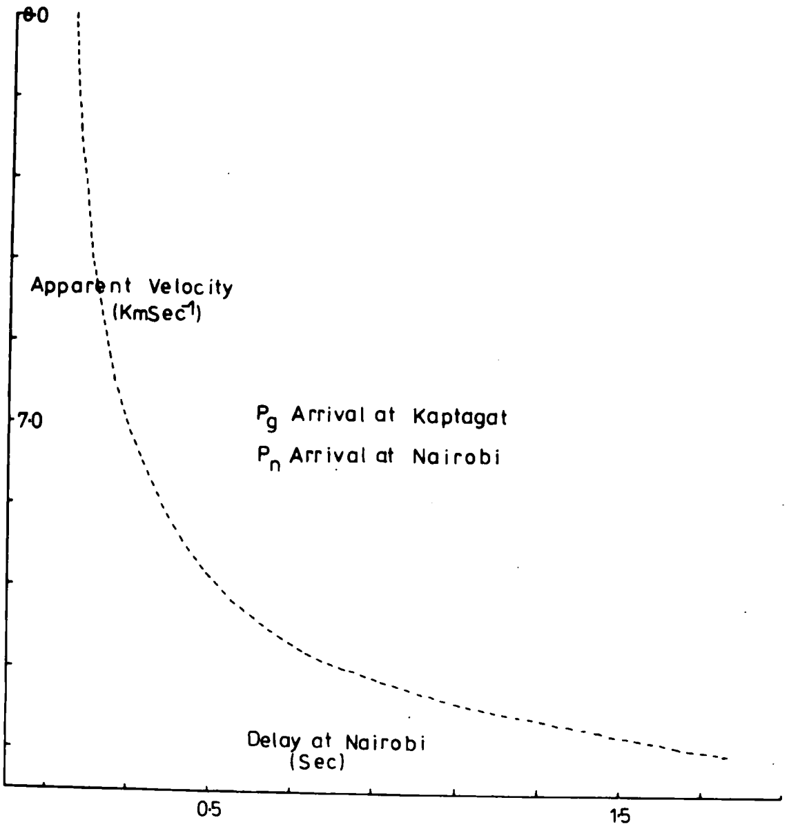
Delay at Nairobi due to an Error of 0.1 KmSec -1 on the First Crustal Layer.
