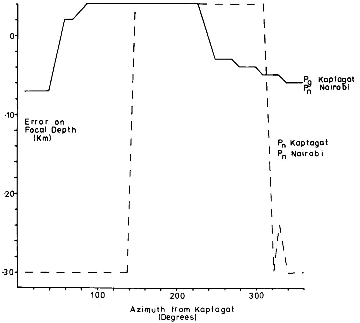
Error on Focal Depth due to Error on the Measured Azimuth.
