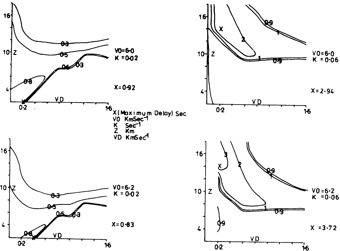
Delay at Nairobi as a Function of the Velocity Drop, VD, at a Discontinuity at Depth Z for Constant Velocity Increase, K, and Initial Velocity V_0 .
