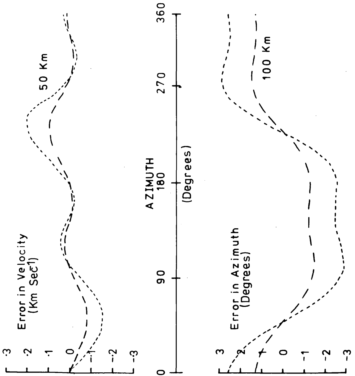
Error on Azimuth and Velocity Due to Assuming a Plane Wavefront
