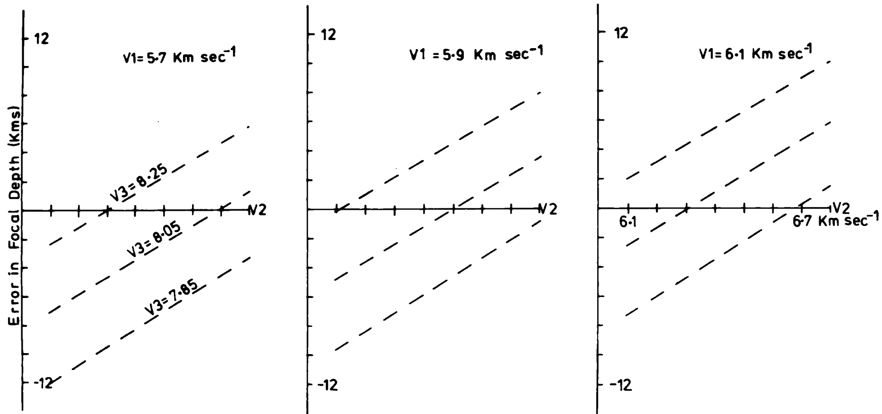
Variation of the Error on the Focal Depth Due to Variation of the P-Velocity of the Three Layers Forming the Crustal Model
