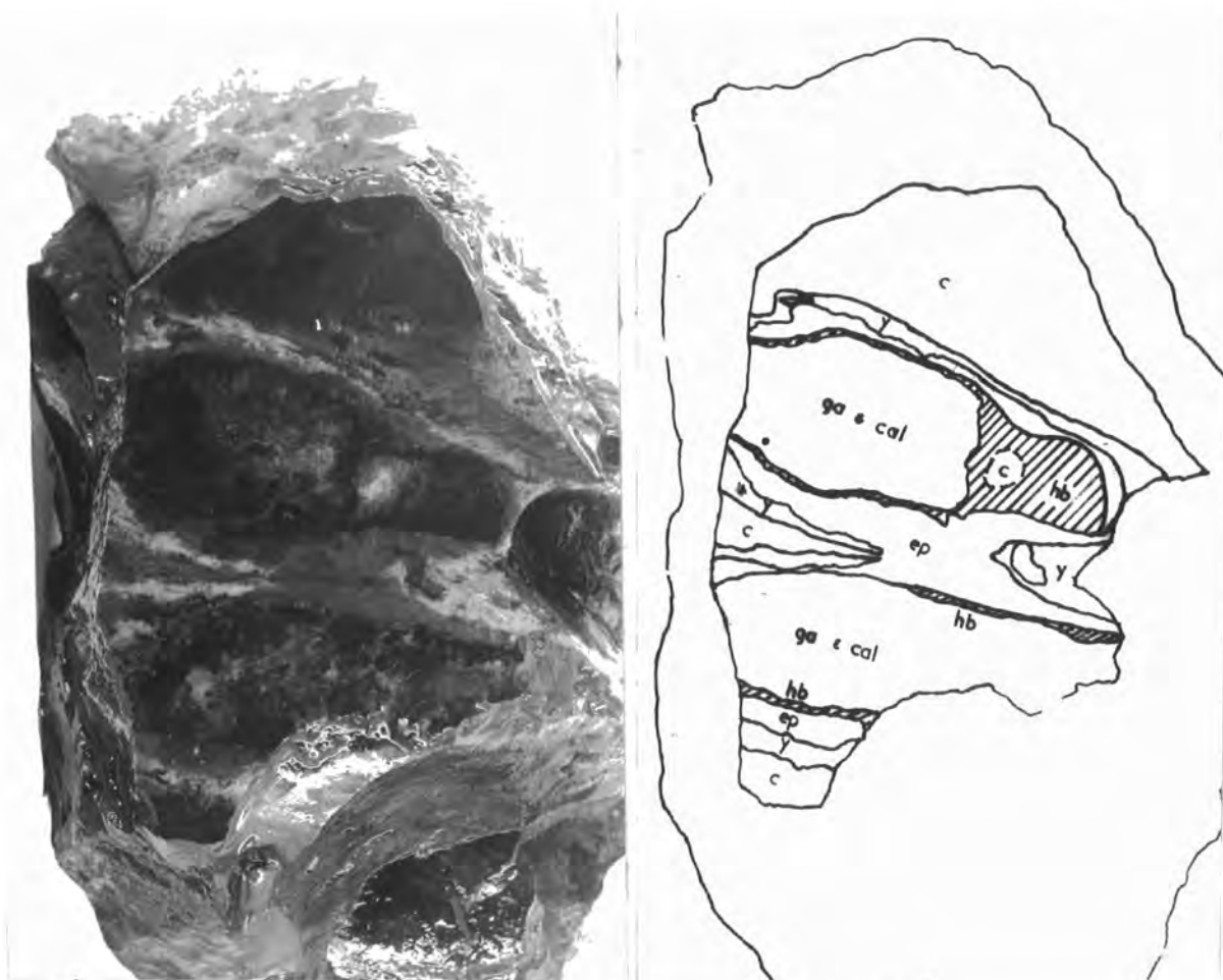
Fig.21.(R.F.31.) Irregular replacement patches. c = country rock, y = reaction zone, hb = hornblende, ep = epidote, ga = garnet, cal = calcite.
