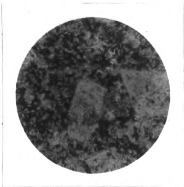
Fig.7.(R.J.26.) Metamorphosed porphyritic andesite. Great Grain Gill, Eskdale. Felspar phenocrysts sericitised. Ground mass impregnated with haematite.(x 35).
