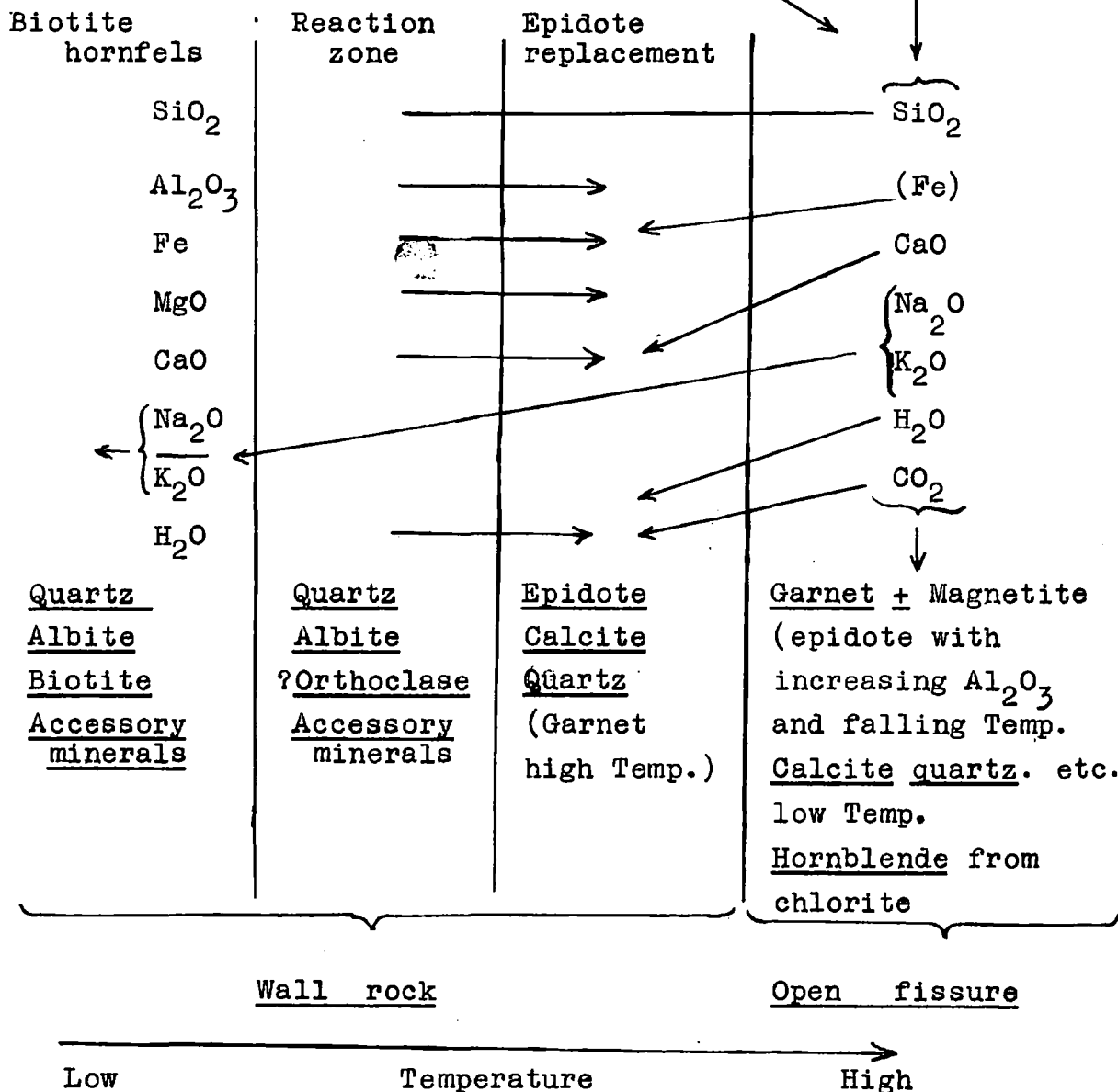
Schematic representation of the petrogenesis of a garnet bearing vein.
