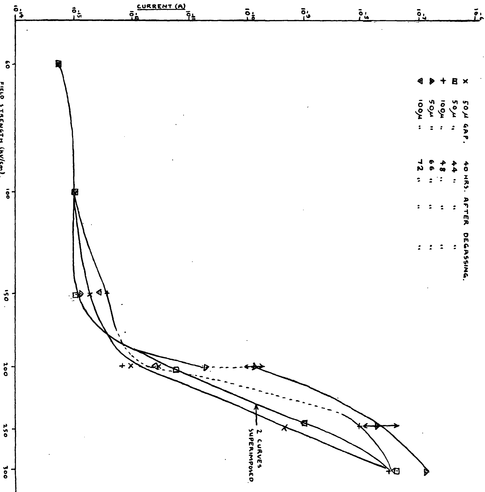
FIG. 47. THE (I,V) CHARACTERISTIC FOR PURE n-HEXANE
