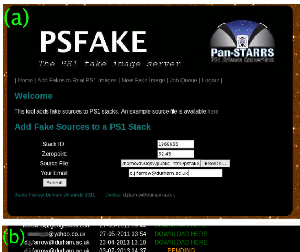
Figure 2.4: Screenshots from the synthetic image server. Panel (a) shows the page where the user submits requests, panel (b) shows the queue page where the user can download the finished images.
