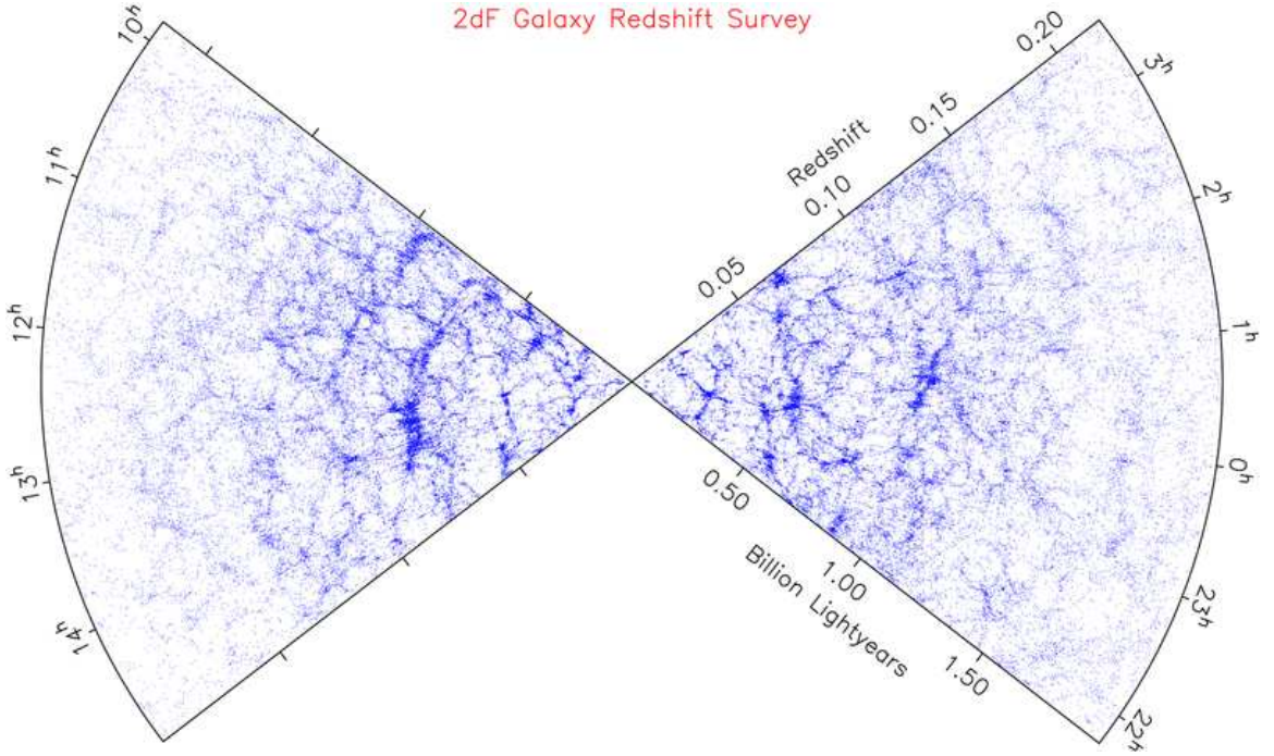
Figure 1.2: The positions of galaxies in 2dFRGS. Large scale structure is apparent. The figure is from http://www2.aao.gov.au/2dFRGS/ , accessed 04/05/13.
