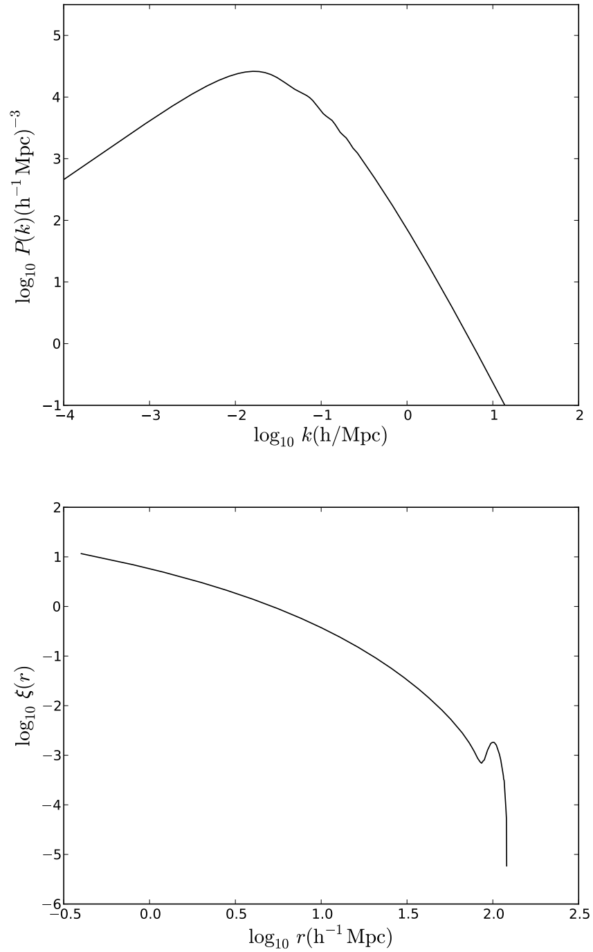
Figure 1.5: Top : A model power spectrum, from CAMB (Lewis & Bridle (2002)). Bottom : The correlation function computed by Fourier transforming the power spectrum. The baryonic acoustic peak can clearly be seen.
