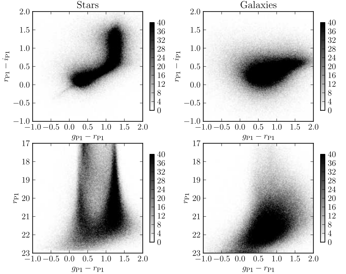
Figure 3.10: Colour-colour and colour-magnitude diagrams, using Kron magnitudes, of SAS2 objects falling on the star side and galaxy side of our chosen star/galaxy separator (section 3.3.1). The greyscale bar gives the number of objects in each colour-magnitude bin. We see the characteristic stellar features highlighted in Finlator et al (2000), such as the upturn in the colour-colour diagram. In support of our classification we see no evidence of these features in the galaxy sample.
