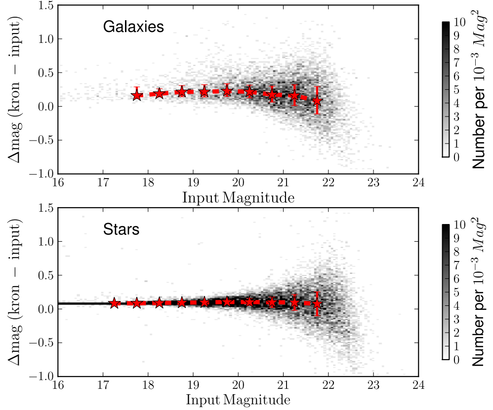
Figure 2.5: The input magnitude versus the recovered magnitude for galaxies (above) and stars (below), for synthetic objects placed on synthetic detrended exposures. The red stars mark the median values, the error bars mark the upper and lower quartiles.
