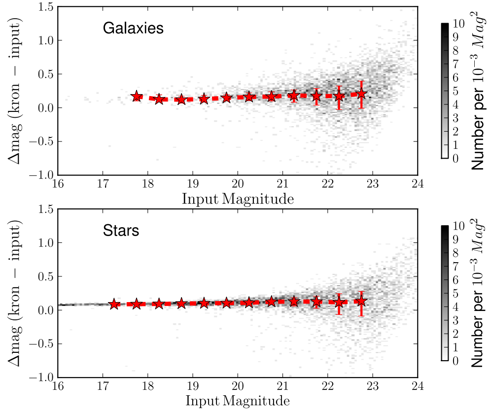
Figure 2.9: The input magnitude versus the recovered Kron magnitude for galaxies (above) and stars (below), for synthetic objects placed on real warps and then stacked. The red stars mark the median values, the error bars mark the upper and lower quartiles.
