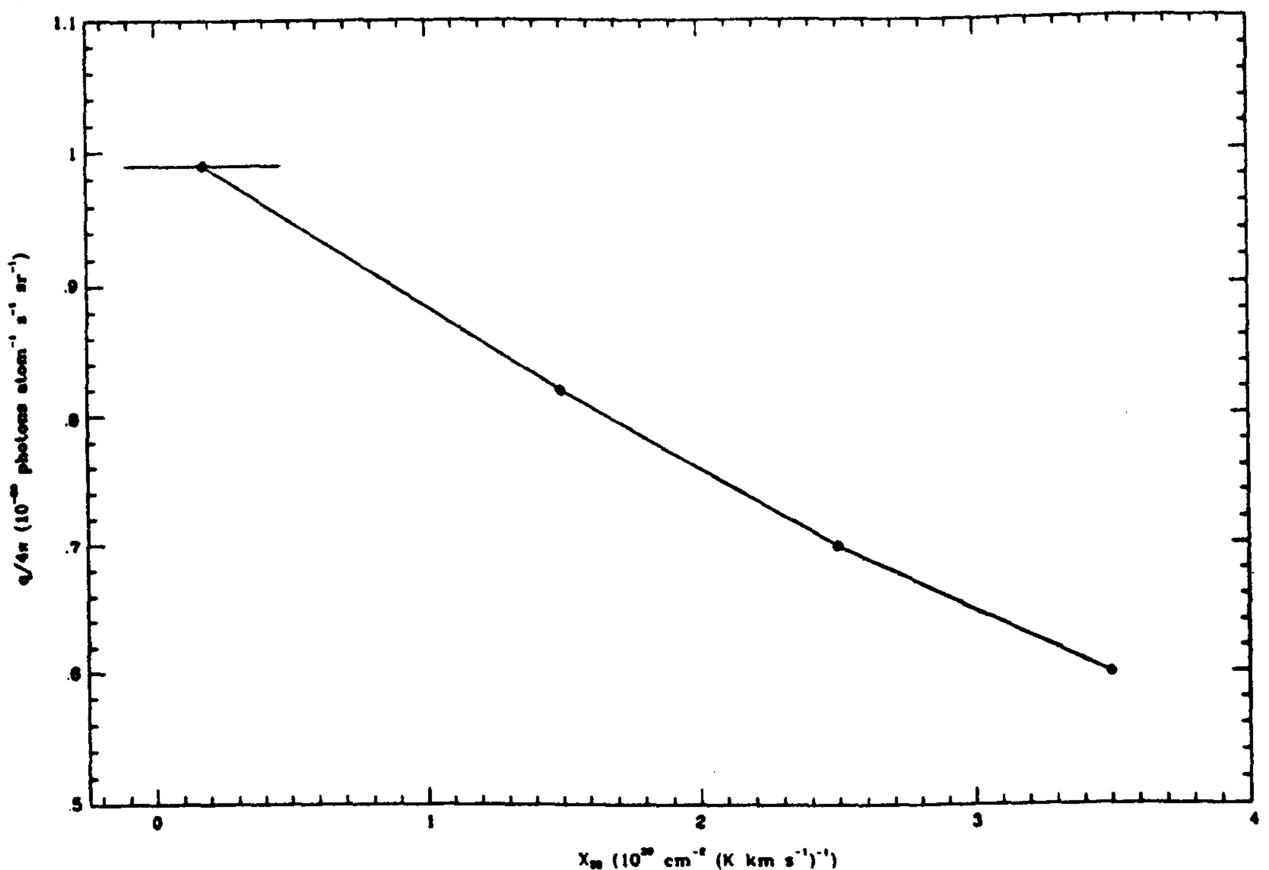
Fig 3.13 q(\text{HI})/4\pi for 300–5000 MeV derived using a 1-parameter fit to the \gamma -ray and gas data in region E for X_{20} = 1.5, 2.5 and 3.5 . The best fit 95% confidence interval for X_{20} is indicated.
