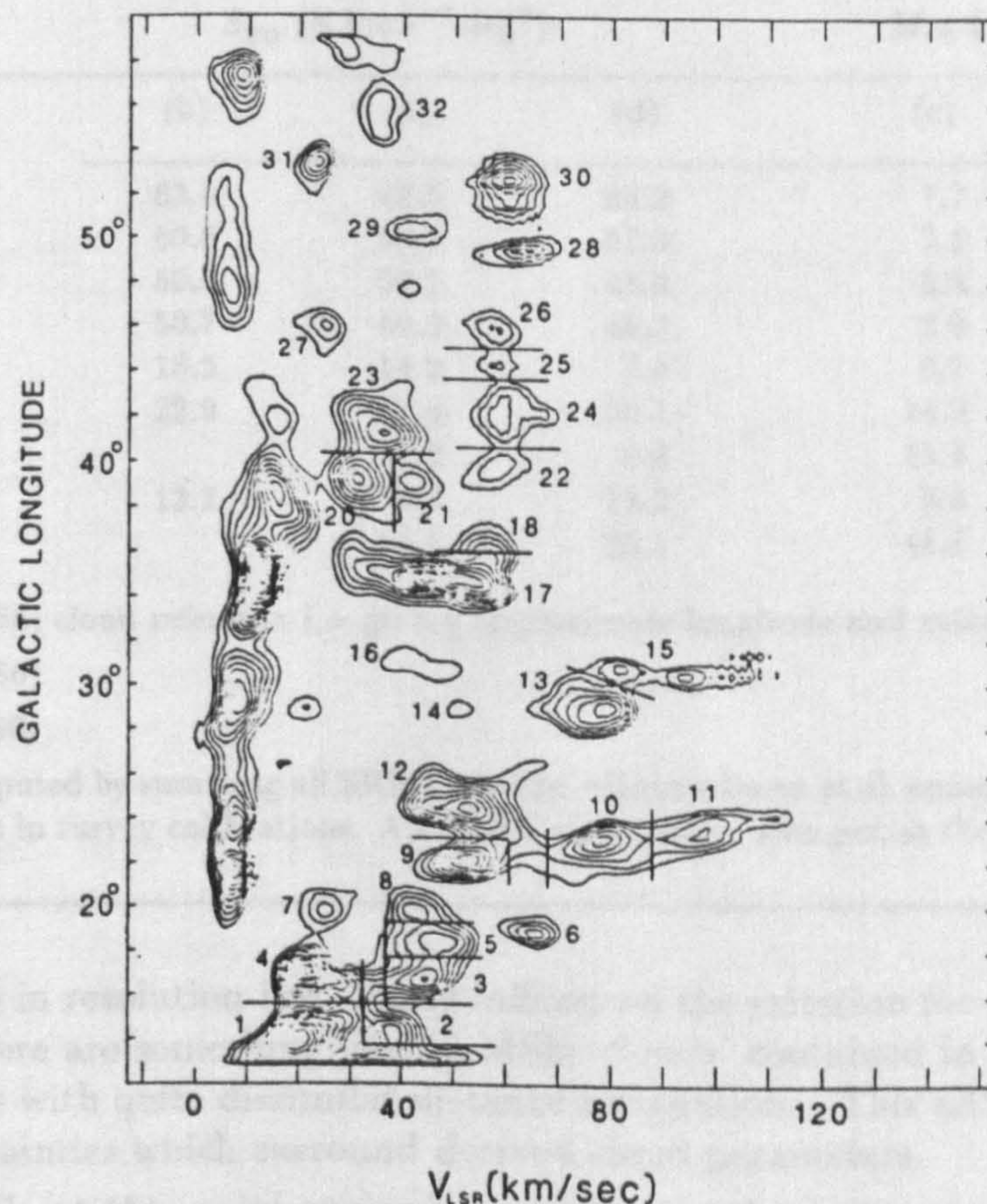
Fig 5.2 l-v map resulting from the Dame et al. (1986) technique of subtracting a model background from the observed l-v map. The model background (see Dame 1984) was scaled so that 75% of the total emission in the observed map was removed. Contour intervals are 0.25 K deg.
