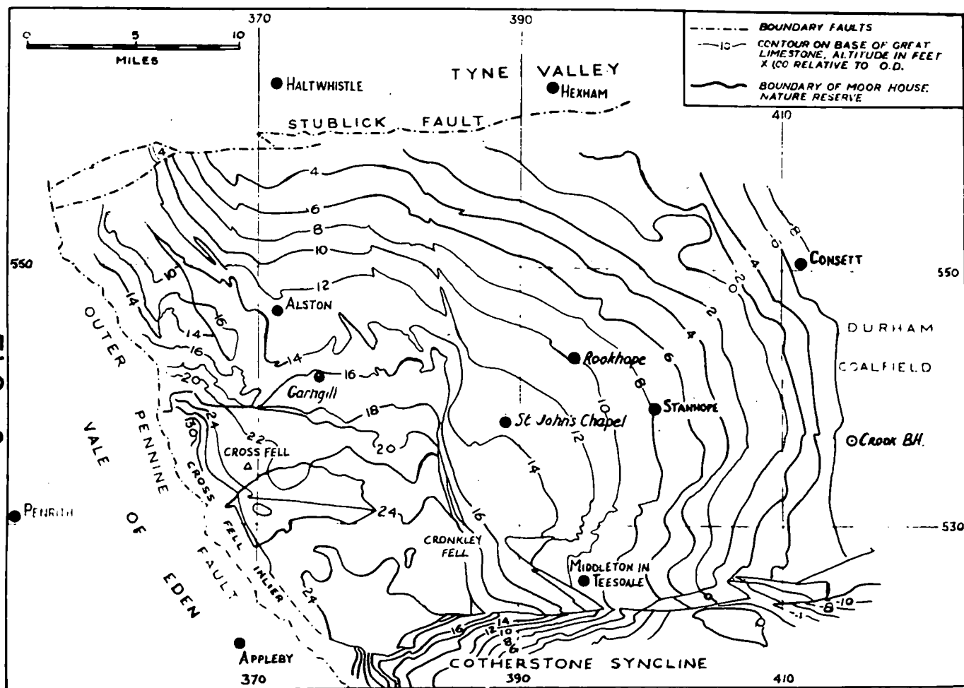
Structure of the Alston Block illustrated by structure-contours on the base of the Great Limestone; heights in hundreds of feet above ordnance datum. Based on Dunham (1959)
