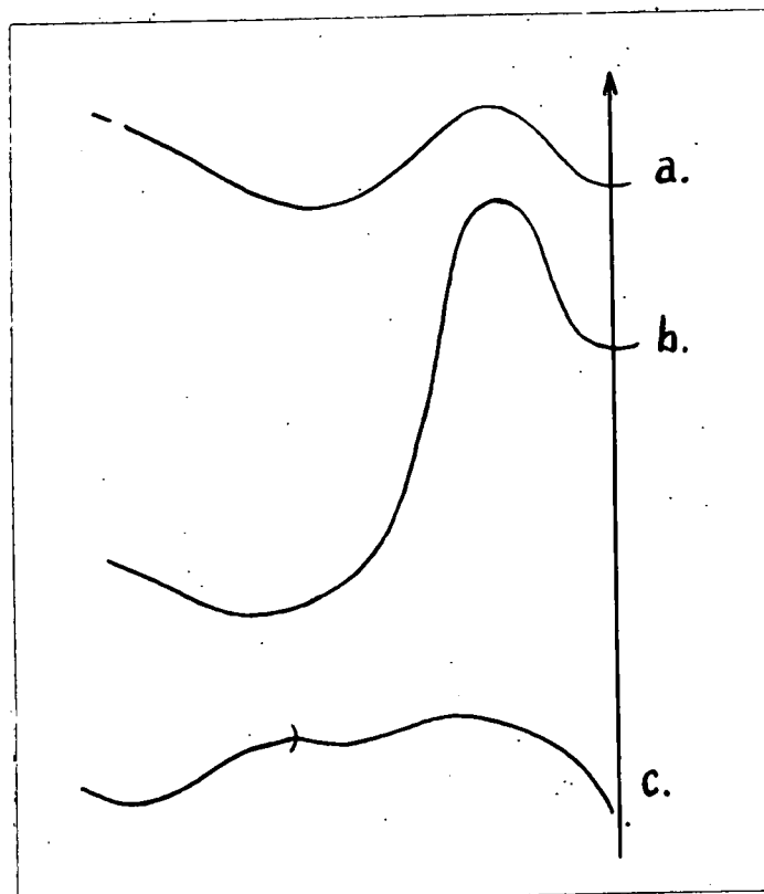
Text fig. 25. Maenioceras terebratum (G. & F. Sandberger). a. Growth lines at c.3mm diameter based on D.802 from Pentonwarra Point, Trevone. b. Growth lines at 6.8mm diameter based on GS.22077 from Trevone. c. Suture based on GS.1609 from Portquin. All Terebratum Zone, Givetian. All X 20.
