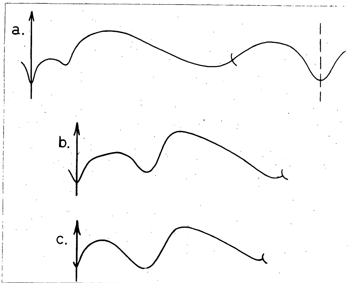
Text fig. 58. Tornoceras (Aulatornoceras) auris auris (Quenstedt). a. Suture at 1.9mm diameter based on D.1107 from Büdesheim, X 50. b, Suture at 6mm diameter based on BM.cl8445 from Saltern Cove, X 25. c. Suture at 12mm diameter based on D.1080 from Büdesheim, X 12\frac{1}{2} .
