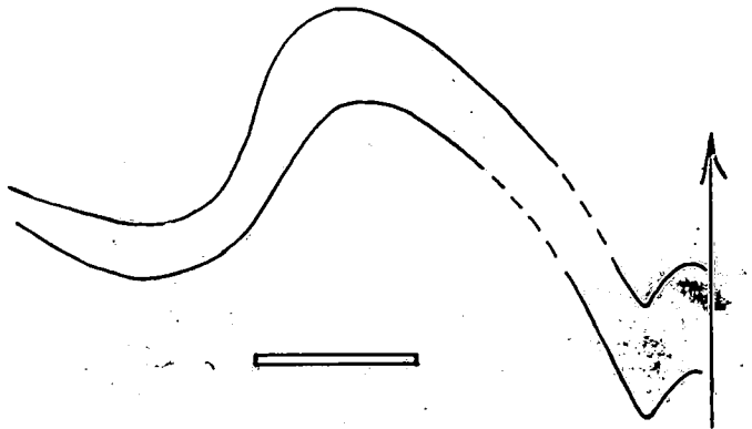
Text fig. 44. Manticoceras sp. indet. Suture of a specimen from Galampton Point, due NNE of Warren House, four miles south of Paignton, South Devon. Frasnian, ? Cordatum Zone. Based on D.401, X 20.
