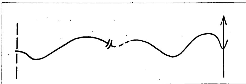
Text fig. 22. Wedekindella psittacinus (Whidborne) . Suture of the syntype BM.c9010 from Wolborough Quarry, South Devon at 20mm diameter. Molarium Zone, Givetian. c. X 6.
