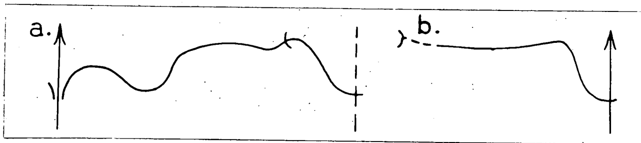
Text fig. 57. Tornoceras ( Protornoceras ) sp. nov. a, Suture and b, growth lines. Both based on D.810 from Pentonwarra Point, Trevone, North Cornwall, X 12½. Terebratum Zone, Givetian.
