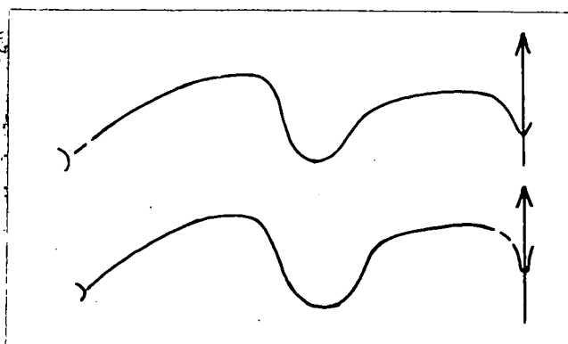
Text fig. 51. Tornoceras ( Tornoceras ) simplex var. ovata Frech. Above, suture based on SM.H1526, Below, suture based on BM.cl8461. Both from Saltern Cove, Devon. Holzapfeli Zone, Frasnian. Both X 12½.
