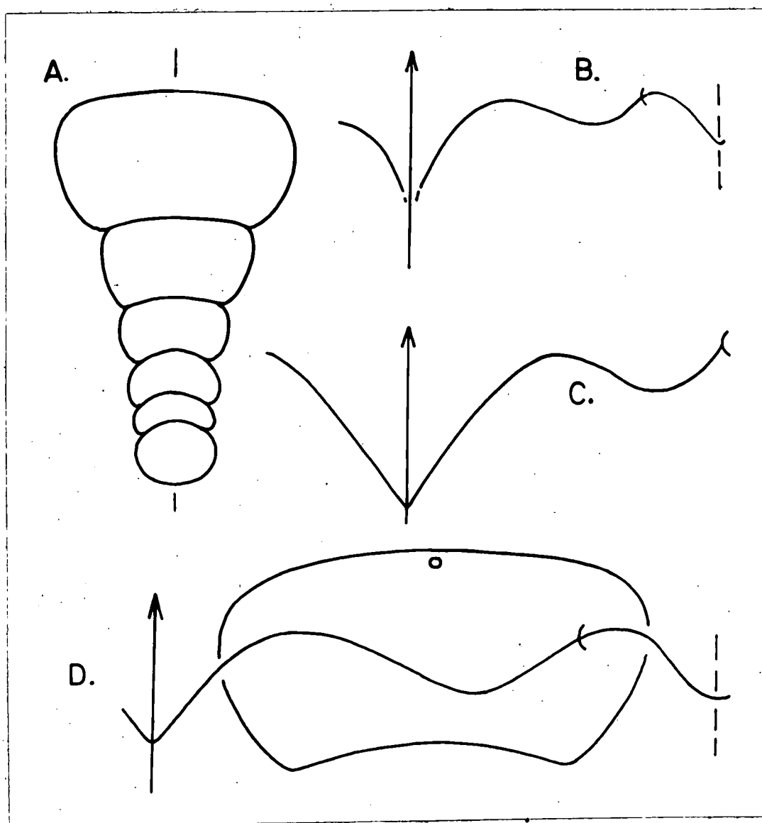
Text fig. 14. Archoceras varicosum (Drevermann). A. reconstructed cross-section of the inner whorls based on D.233, X 20. B. Suture at 6mm diameter of D.233, X 20. C. Suture at 8mm diameter of D.208, X 20. D. Whorl section and suture of D.241 X 40.
