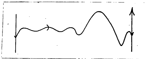
Text fig. 47. Koenenites sp. nov. Suture based on GS.95230 from a quarry NW of St. John Baptist Chapel, Staverton Wood, South Devon, collected by Dr. G.V. Middleton. Frasnian Lunulicosta Zone. X 10.
