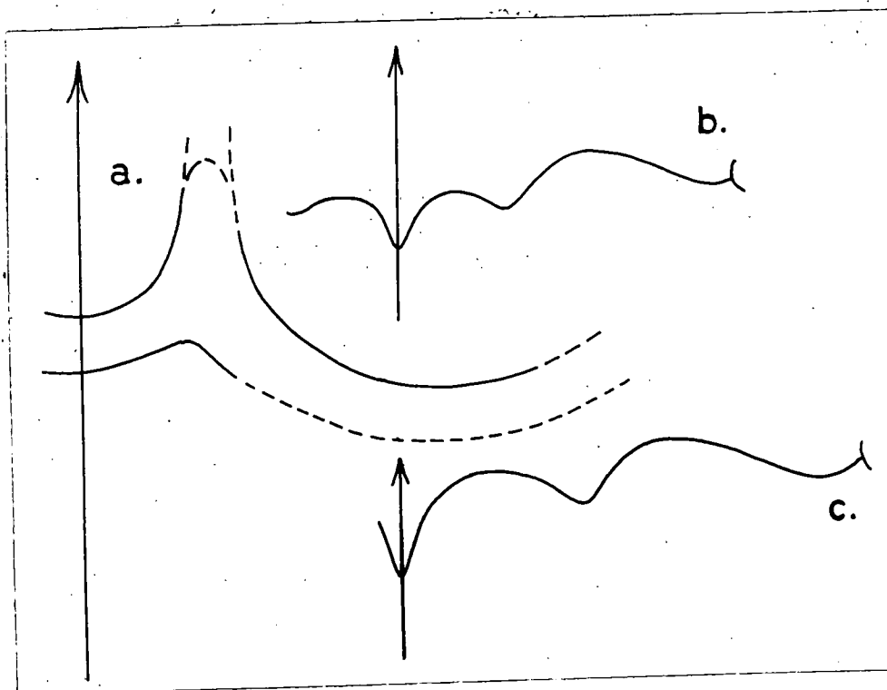
Text fig. 60. Tornoceras ( Aulatonoceras ) paucistriatum var. nov. a, Constriction at 6mm diameter. b, Suture at 4mm diameter, both based on D.246 from Saltern Cove. c, Suture based on SM. H1525 from Saltern Cove. All X 20. Holzapfeli Zone, Frasnian.
