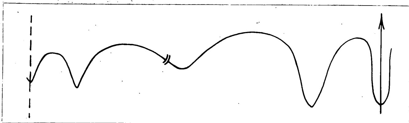
Text fig. 66. Imitoceras sulcatum (Münster). Suture at 14.5mm diameter based on GS.57362, dorsal suture from four septae previous. Specimen from a mine leat 680 yards north-west of Marytavy Church, Devon. X 8.
