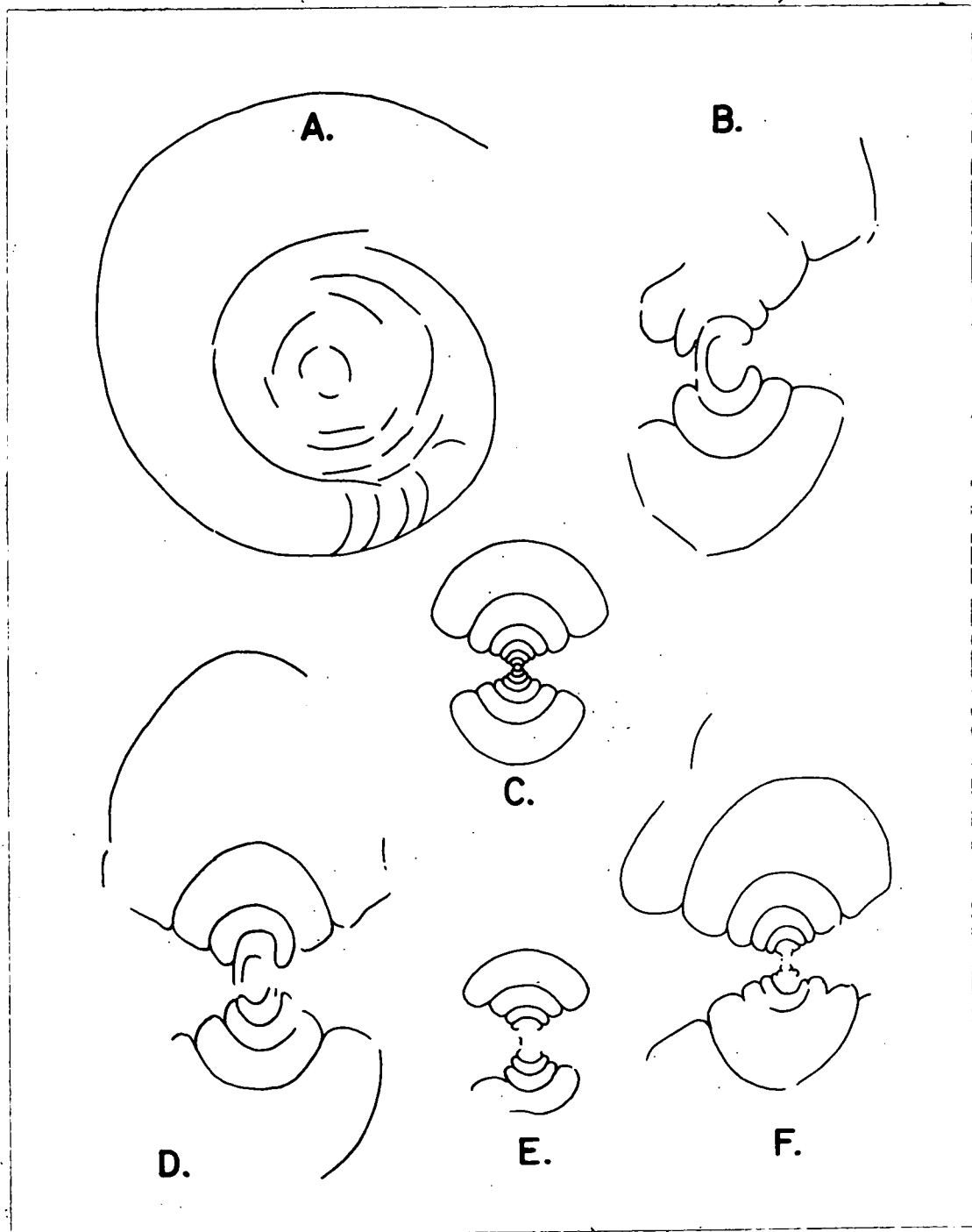
Text fig. 12. ? Anarcestes ( Anarcestes ) lateseptatus (Beyrich) var. plebeius (Barrande). A. TM.72/9, B. TM.68/9, C. BM.c 30396, D. TM.69/9, E. TM.78/9, F. 74/9. All from the lower part of the Calceola Shales at Mudstone Bay, Brixham, Devon. Couvinian, ? Lateseptatus Zone. All natural size.
