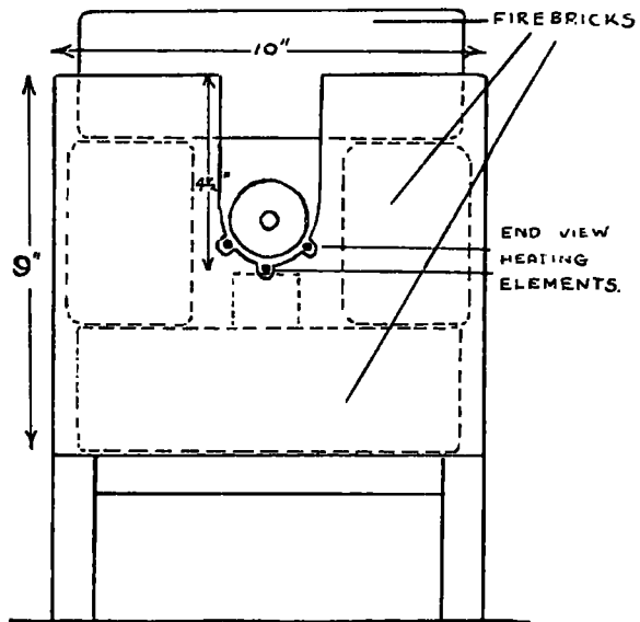
END VIEW OF OVEN
