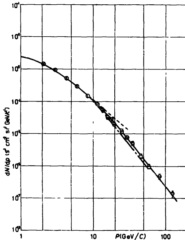
The differential \mu -meson momentum spectrum. Key: ● This experiment, cloud chambers; ○ This experiment, Geiger counters; ---- Rossi (1) ; — Owen and Wilson (1) ; - - - Caro et al. (2) .
