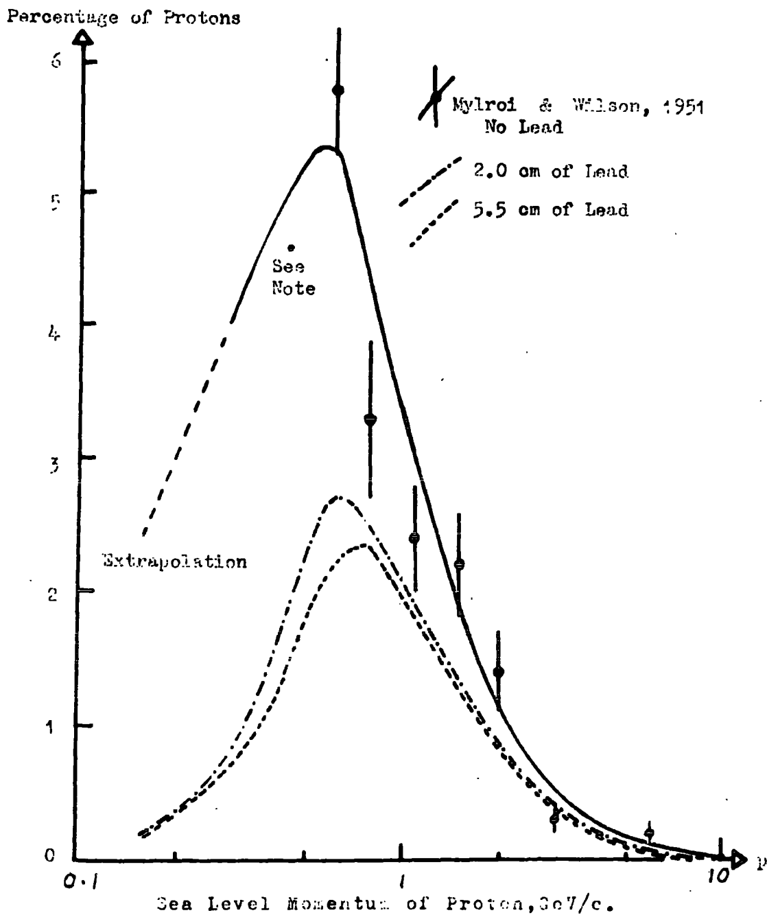
FIG.4.6.3. The Proton Spectrum of Myroli and Wilson (1951) used in correcting for proton intensity. Modified after Sternheimer, (1959). Note : this point is originally due to Rochester and Bound, 1940, but is plotted as corrected by York, 1952.
