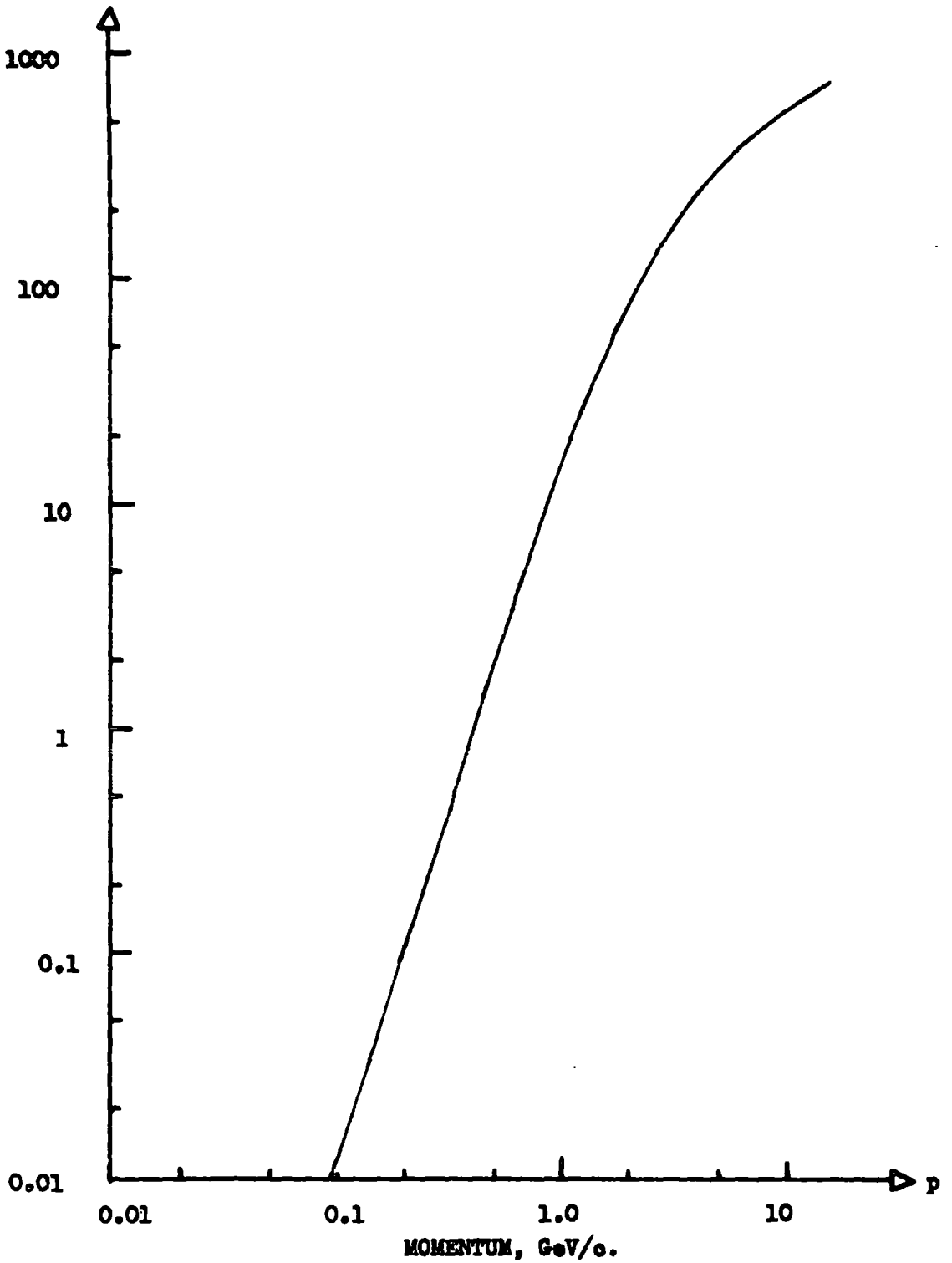
FIG. 4.6.1. Range momentum relationship for Protons in Lead, from the work of STERNHEIMER, 1959.
