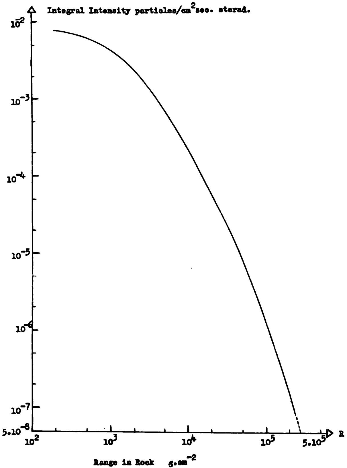
FIG. 9. 3. 1 Integral Range Spectrum of Muons at Sea-Level.
