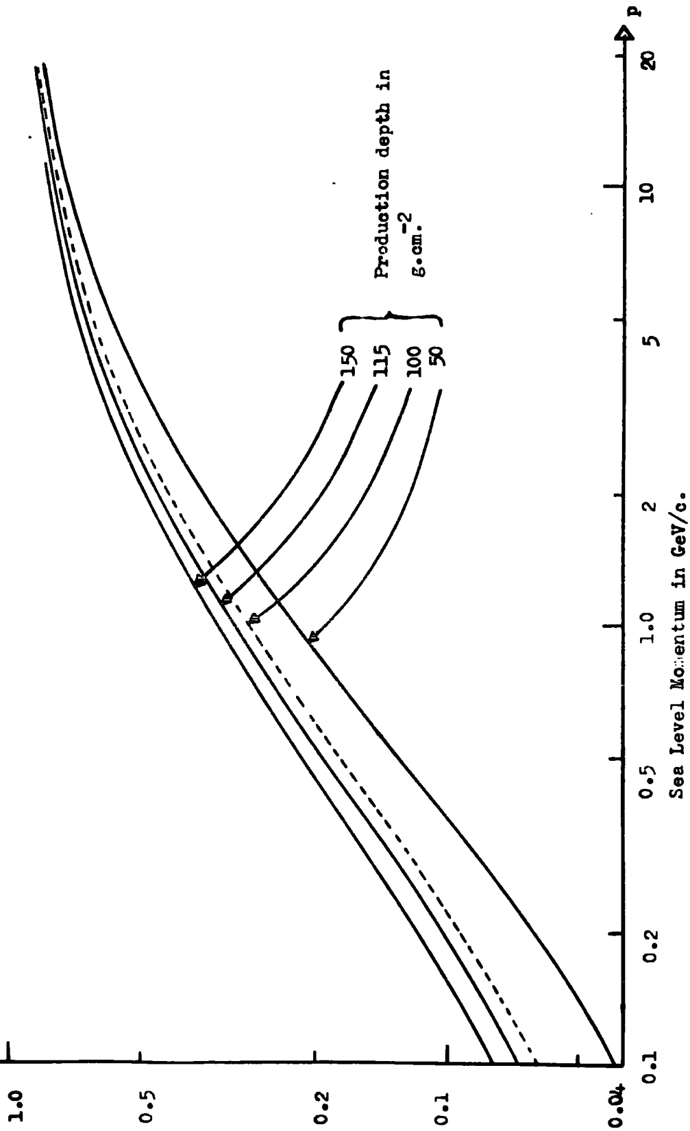
FIG.7.1.1.1. Survival Probability as a function of Sea Level Momentum, for a series of production depths.
