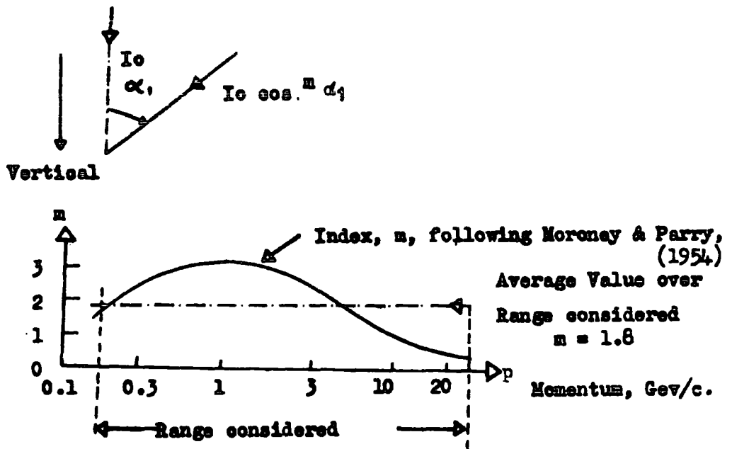
FIG. 3. 8. 7. Expansion of Flux - Model
