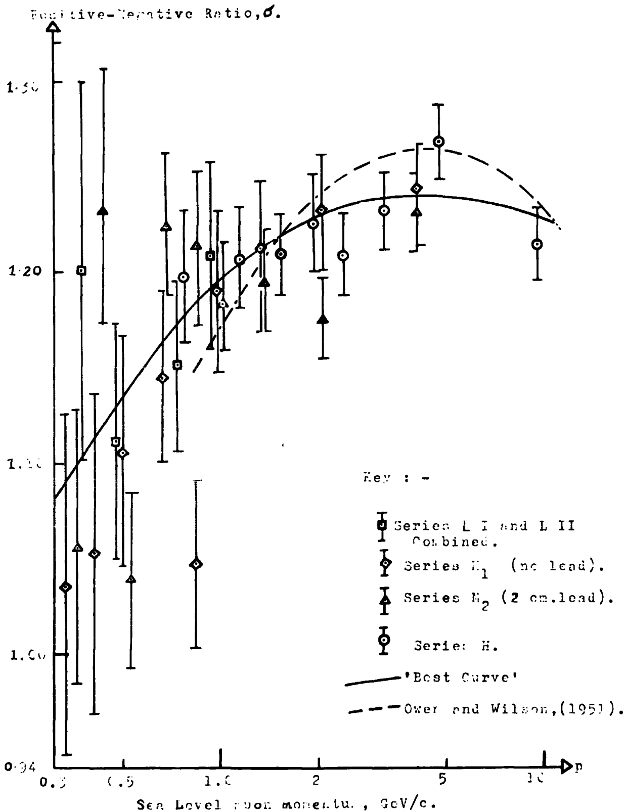
FIG. 3.1.2. Experimental Observations of the Positive-Negative Ratio of Muons at Sea level, corrected for momentum loss and Proton Component.
