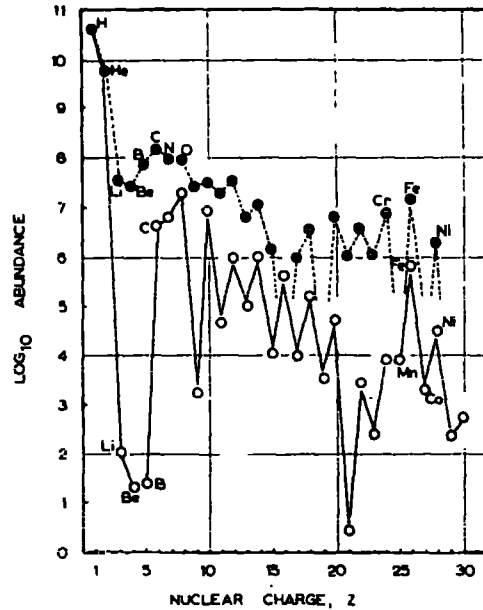
Relative abundances of different elements in the primary cosmic radiation and in the general matter of the universe. Results for cosmic radiation are shown by full circles; for the general matter of the universe, open circles, the two distributions being normalized to hydrogen and helium. The crucial points of difference are the appreciable abundance of lithium, beryllium and boron, and the over-abundance of nickel, iron and other neighbouring elements, in cosmic radiation.
