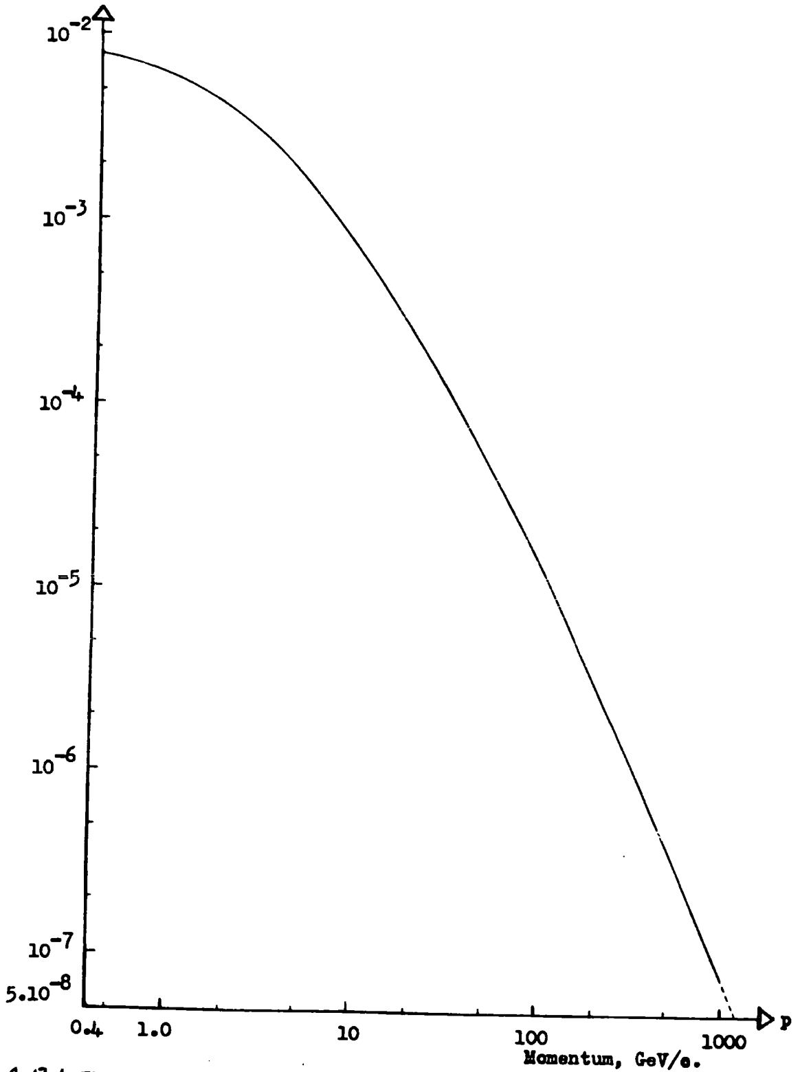
FIG. 4. (3.1) The Integral Momentum Spectrum of Muons at Sea-Level.
