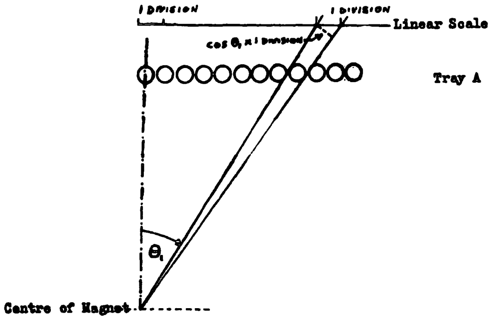
FIG. 3. 8. 7. Expansion of Flux - Model
