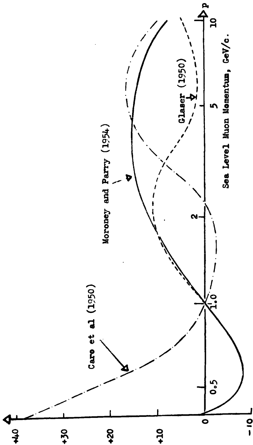
FIG. 6.4.1. Comparison between the Durham Sea Level Spectrum and the curves of FIG. 6.3.1. Normalised to Rossi's 1 GeV/c intensity.
