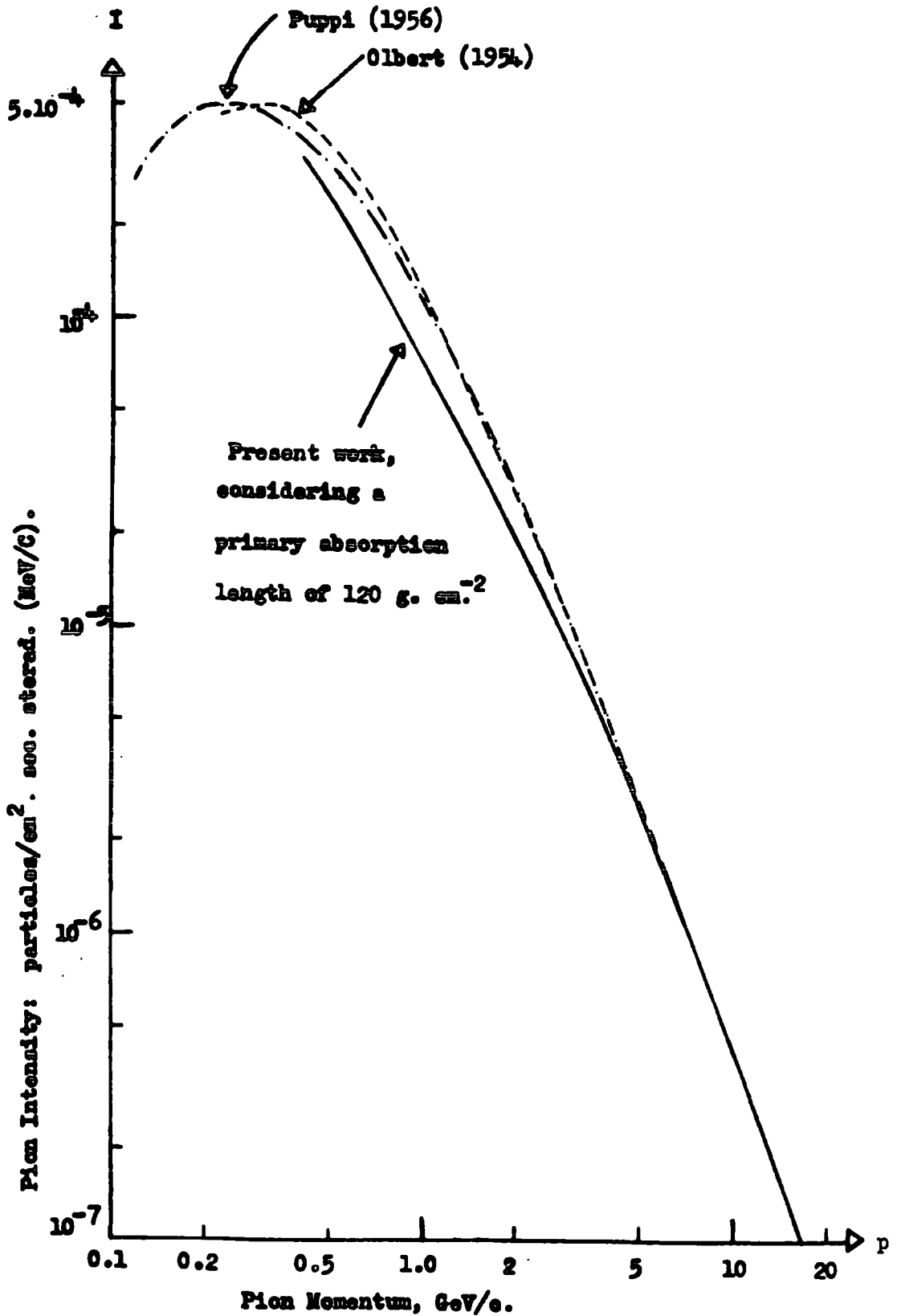
FIG. 7.2.5. The Generation Spectra of Pions in the Atmosphere, considering extended production of pions.
