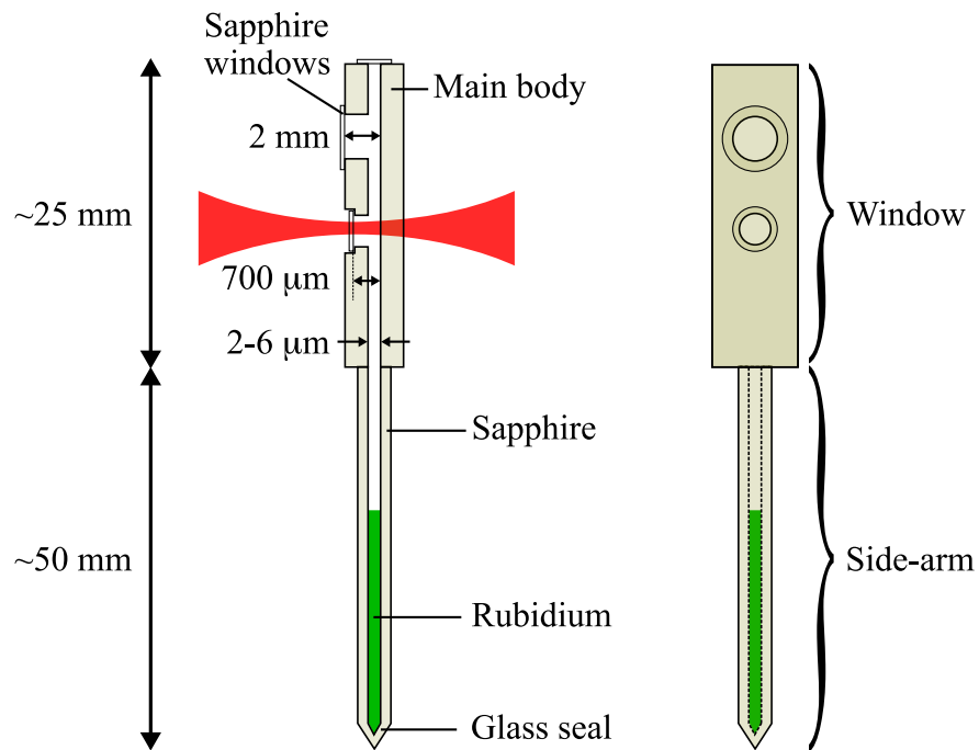
Figure 5.4: The multi-region cell. Side view (left) and front view (right). The cell has three regions of varying thickness, 2 mm, 700\ \mu\text{m} and 2\text{--}6\ \mu\text{m} . Two thermocouples are placed adjacent to the thin cell. The first measures the temperature of the ‘window’ region and the other the ‘side-arm’.
