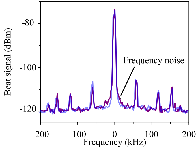
Figure 6.10: Power spectrum showing broader frequency features in the presence of no current feedback, purple, and with feedback, translucent blue. The sidebands at harmonics of 62 kHz are suspected to be due to electric field noise.
