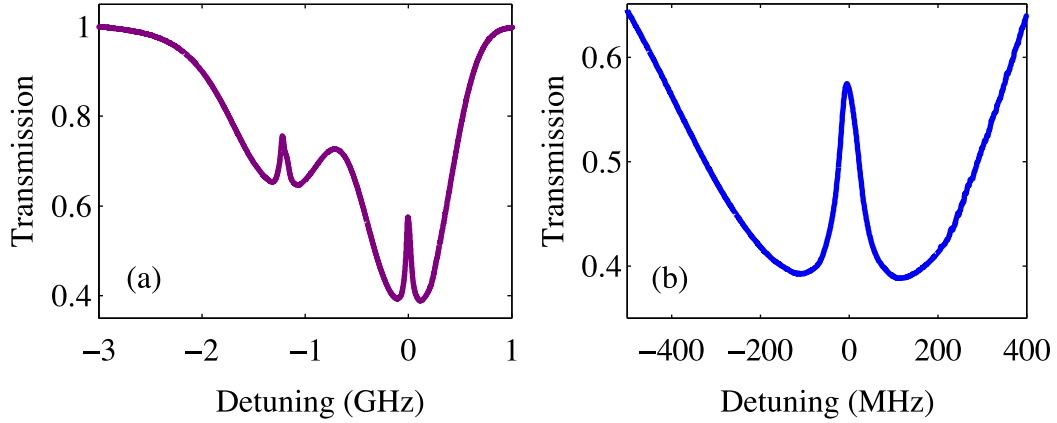
Figure 5.13: Ladder EIT in the micron cell. 56 mW coupling power in the 776 nm laser and a probe power of 1 \mu W. Window temperature 198 °C and side-arm temperature 135 °C. 5 cm lenses, with input beam sizes of approximately 1 mm ( 1/e^2 radius). Cell length is around 2.5 \mu m. Probe detuning is relative to the 5S_{1/2}(F = 3) \rightarrow 5P_{3/2}(F' = 4) transition in ^{85}\text{Rb} .
