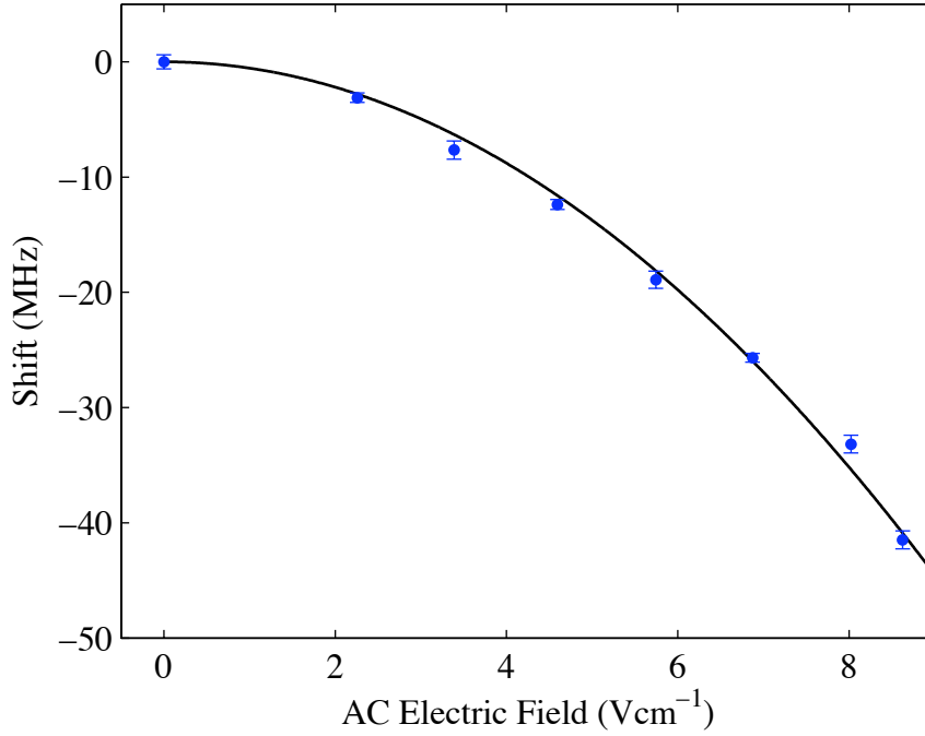
Figure 7.4: Stark shift of the 32S_{1/2} state as a function of applied ac electric field. The solid line gives the theoretical fit using the plate separation as a free parameter.
