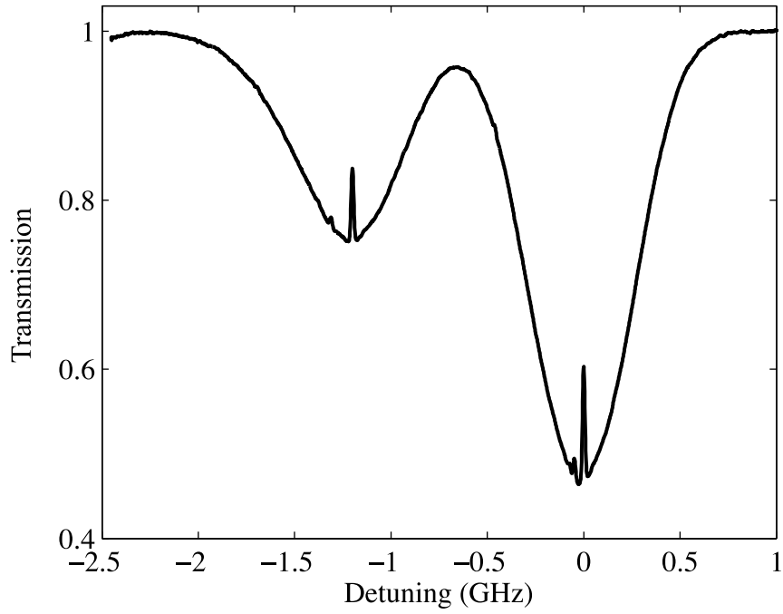
Figure 4.3: Rydberg EIT spectrum corresponding to the case of a probe laser around the D 2 transition in ^{87}\text{Rb} and ^{85}\text{Rb} . The coupling beam is resonant with the 27\text{D}_{5/2} state and has a power of 80 mW, while the probe beam has less than 1\text{ }\mu\text{W} .
