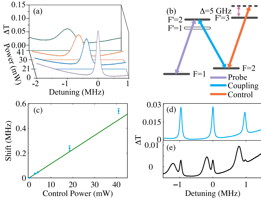
Figure 3.8: (a) Change in transmission as a function of detuning from the 5^2\text{S}_{1/2}(F = 1) \rightarrow 5^2\text{P}_{3/2}(F' = 2) level. (b) Level scheme for the N -system with a far off-resonant control field is used to shift the F = 2 ground state. (c) Shift in frequency of EIT peak for various control beam powers. Data points are taken from (a), whilst the solid line is the calculated ac Stark shift. (d) Change in probe transmission as a function of detuning from the F = 1 \rightarrow F' = 2 level, with a small magnetic field of order 1 Gauss to lift the degeneracy in the F = 1 and F = 2 ground states. In (d) three peaks in transmission are seen for no control beam. A control beam with 110 \mu\text{W} , detuned by -5 MHz from the F' = 3 level, is applied to split the peak in (e).
