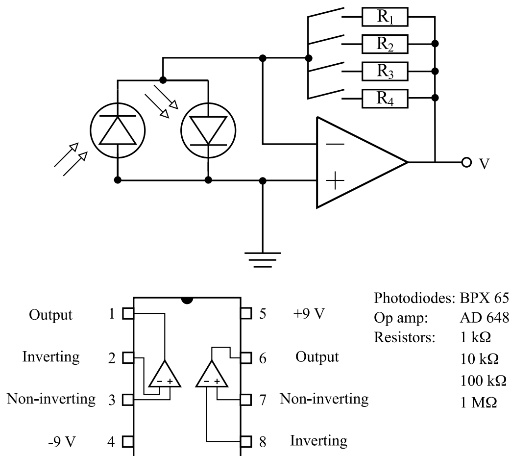
Figure E.1: Circuit diagram used for building a differencing photodiode.
