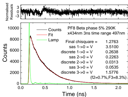
Figure 3-12: Example deconvolution fit to a fluorescence decay profile with the laser scatter profile and the 3-exponential fit using the components listed in the graph.
