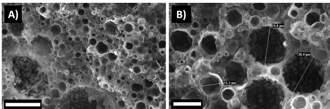
Figure 2:8 – SEM Images of thermally polymerised GMA/EGDMA polyHIPE A) Scale bar 50 \mu\text{m} B) Scale bar 20 \mu\text{m}
