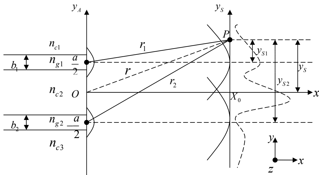
Figure 44 Schematic diagram of fringe formation
