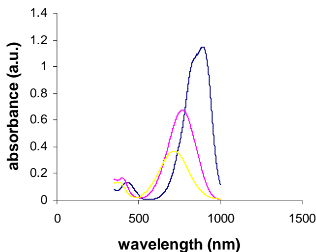
Figure 21 Solvatochromic absorption spectra of C_{18}H_{37}-Q3CNQ in dichloromethane (blue line), acetone (pink line) and acetonitrile (yellow line)
