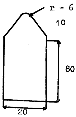
Section X. A Details of Knife Edge Supports
