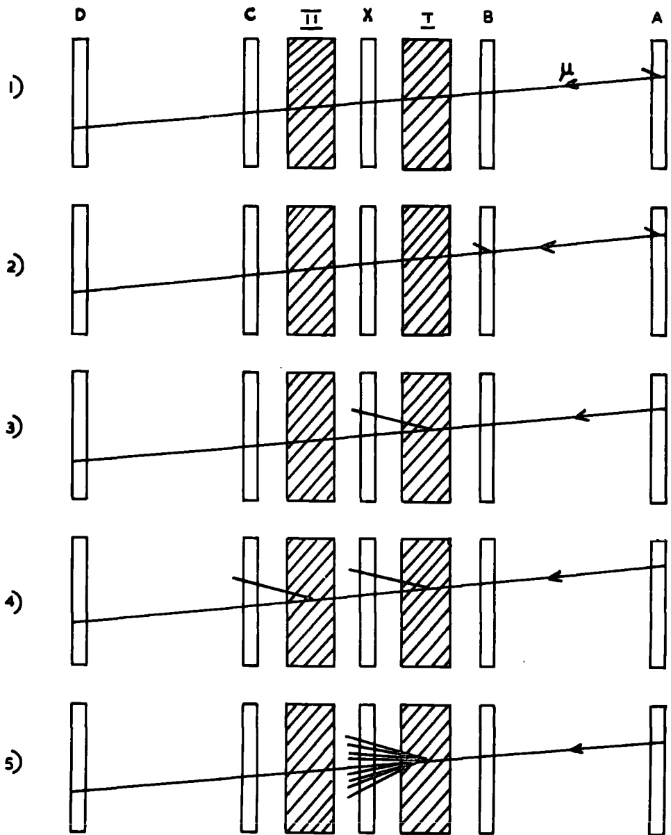
Fig. 6.1 An illustration of the interaction categories.
