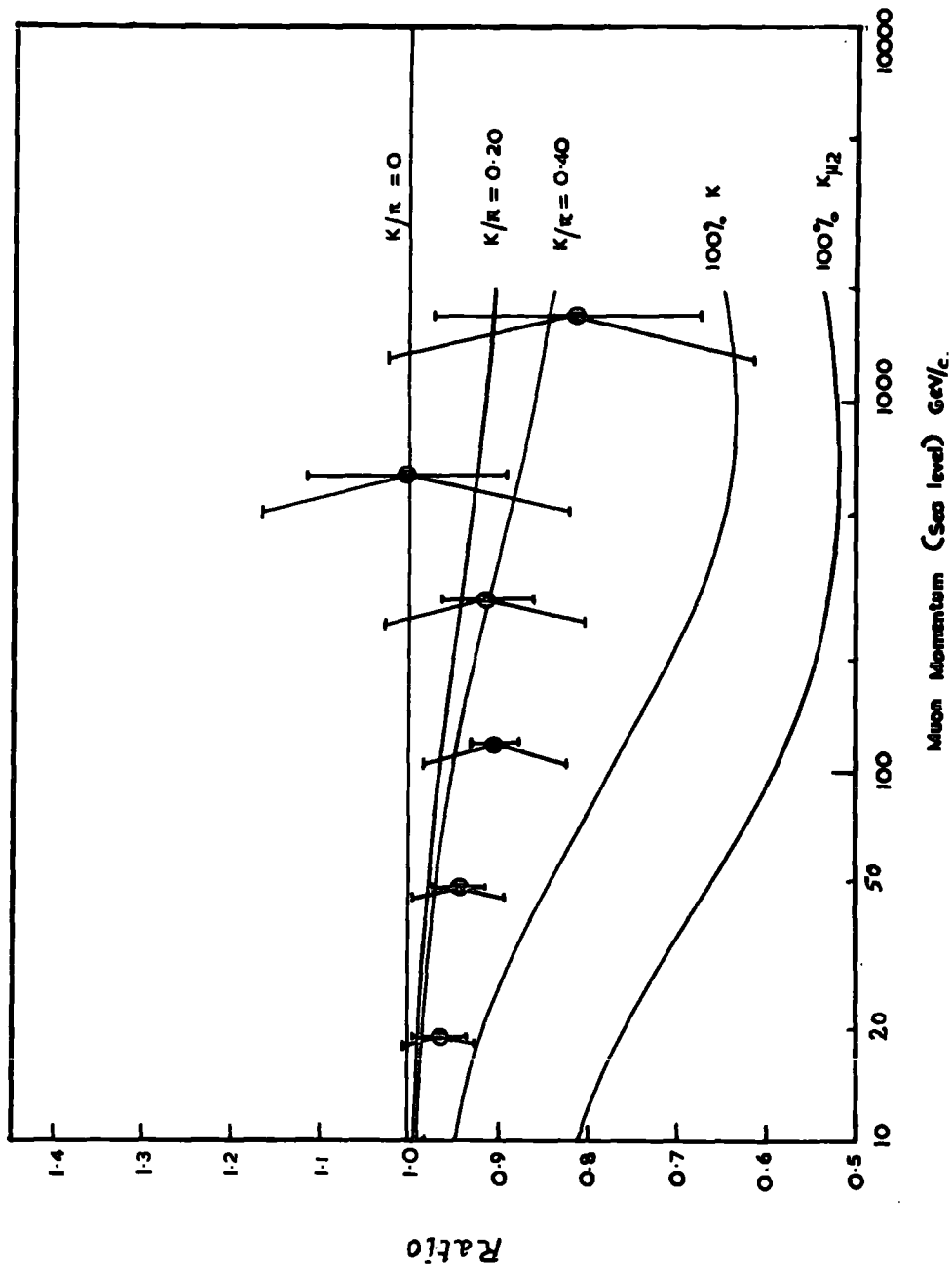
Fig. 4.3 Comparison of measured and predicted intensities with those for pions as the only parents.
