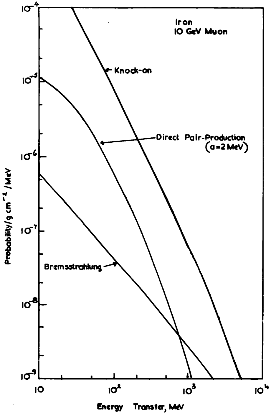
Fig. 6.7 Differential energy transfer curve for 10 GeV muons in iron, after Rogers (1965).
