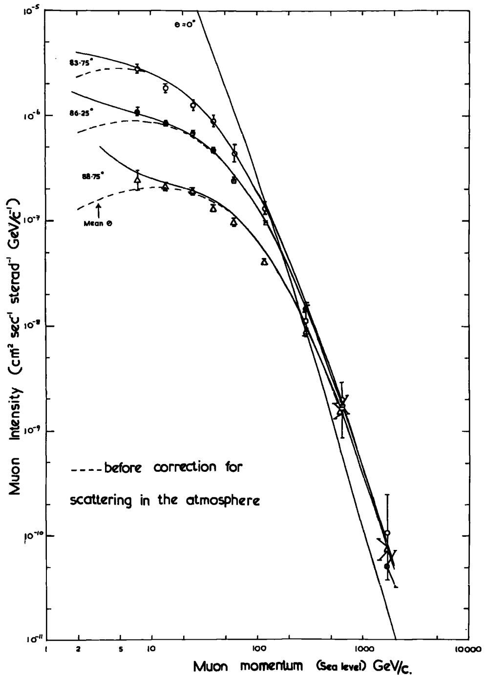
Fig. 4.2 Comparison of the measured momentum spectra at large zenith angles with the predicted ones after Osborne (1966).
