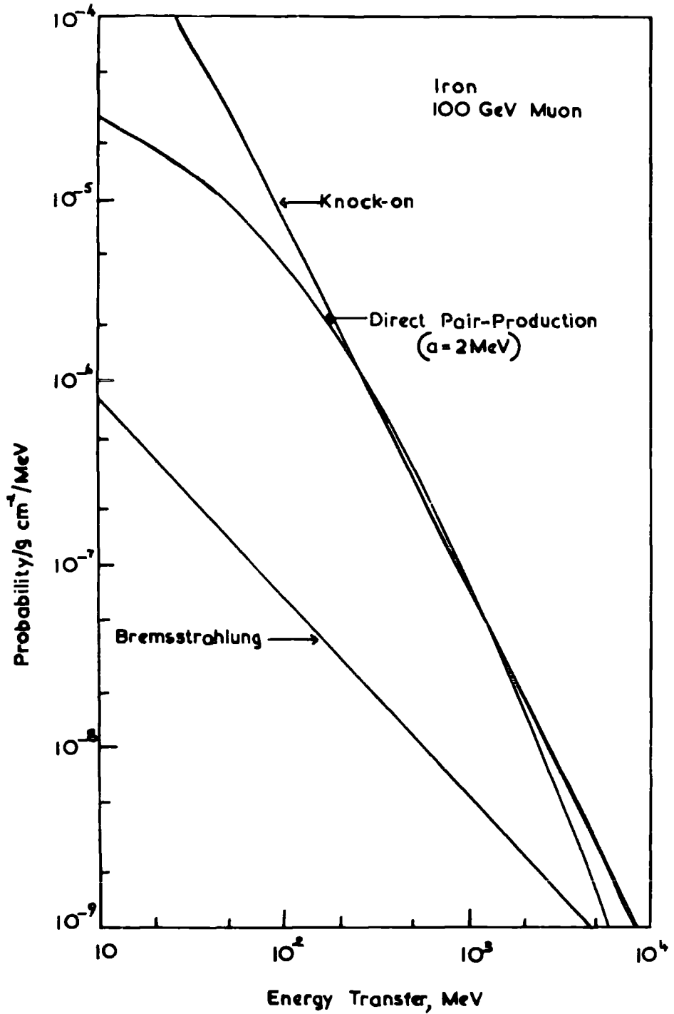
Fig. 6.8 Differential energy transfer curve for 100 GeV muons in iron, after Rogers (1965).
