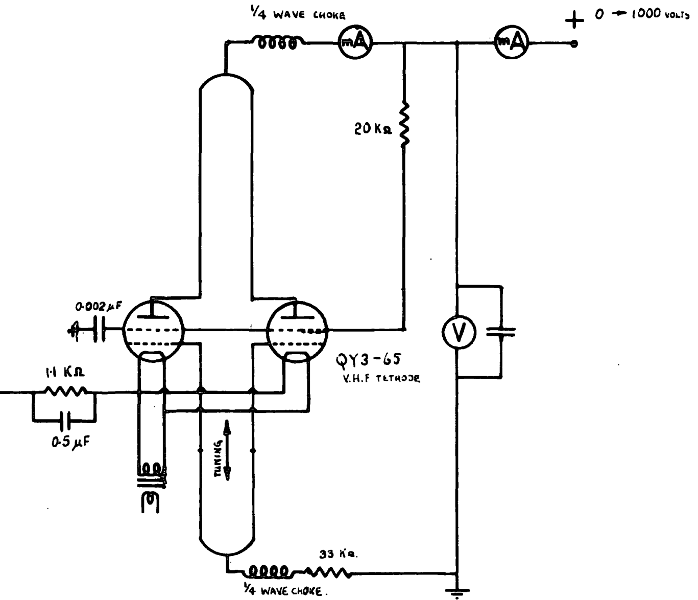
U.H.F. OSCILLATOR CIRCUIT DIAGRAM.
