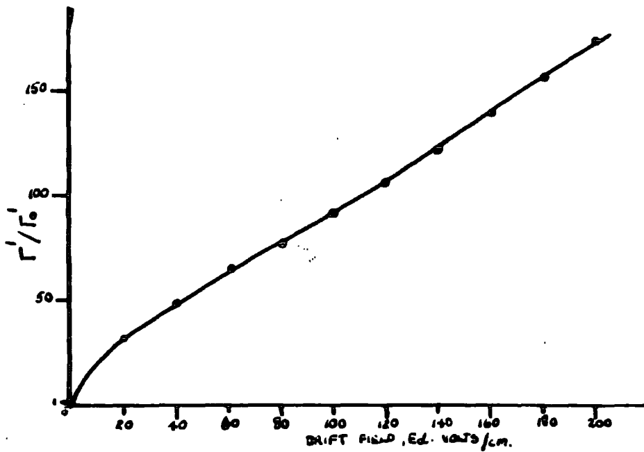
FIG. 12.5 THEORETICAL RATIO OF THE CURRENT TO THE LOW-FIELD ELECTRODE WITH A DIRECT FIELD TO THAT WITHOUT A FIELD AS A FUNCTION OF THE FIELD.
