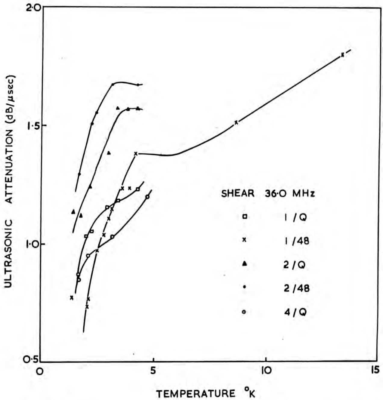
Figure 6.22 Ultrasound attenuation below 4.2^{\circ}\text{K} in samples 1/Q □, 1/48 x, 2/Q ▲, 2/48 • and 4/Q ○ at 36.0 MHz
