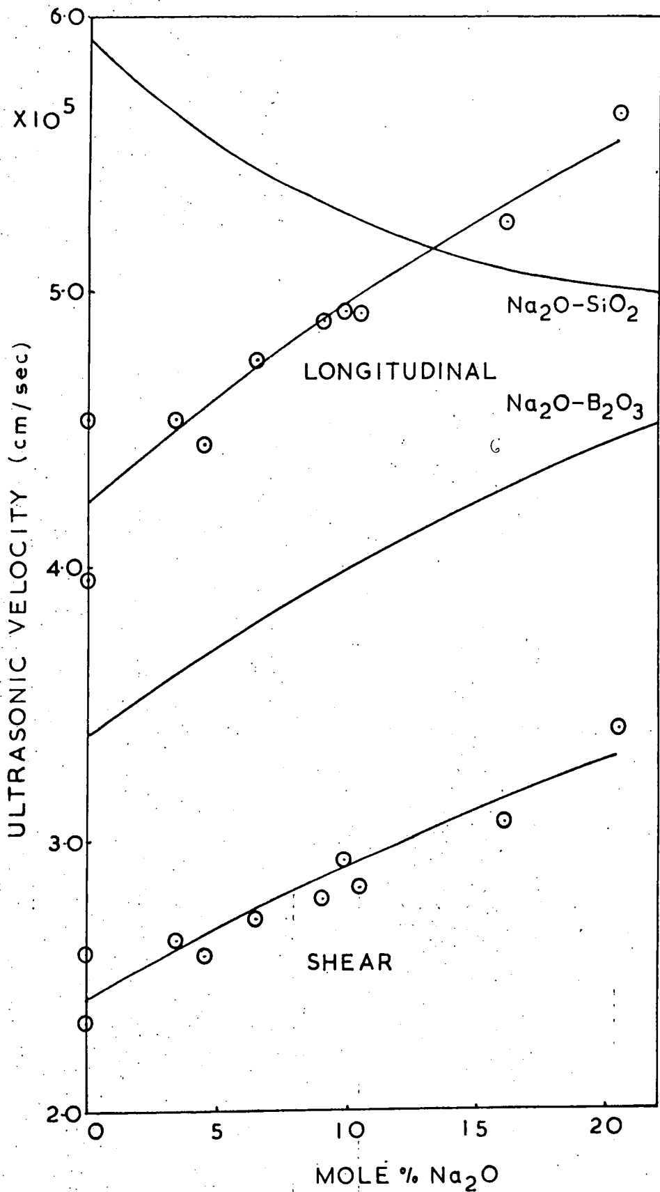
Figure 7.8 Ultrasound velocities for Na 2 O - B 2 O 3 - SiO 2 glasses in comparison with Na 2 O - SiO 2 and Na 2 O - B 2 O 3 glasses.
