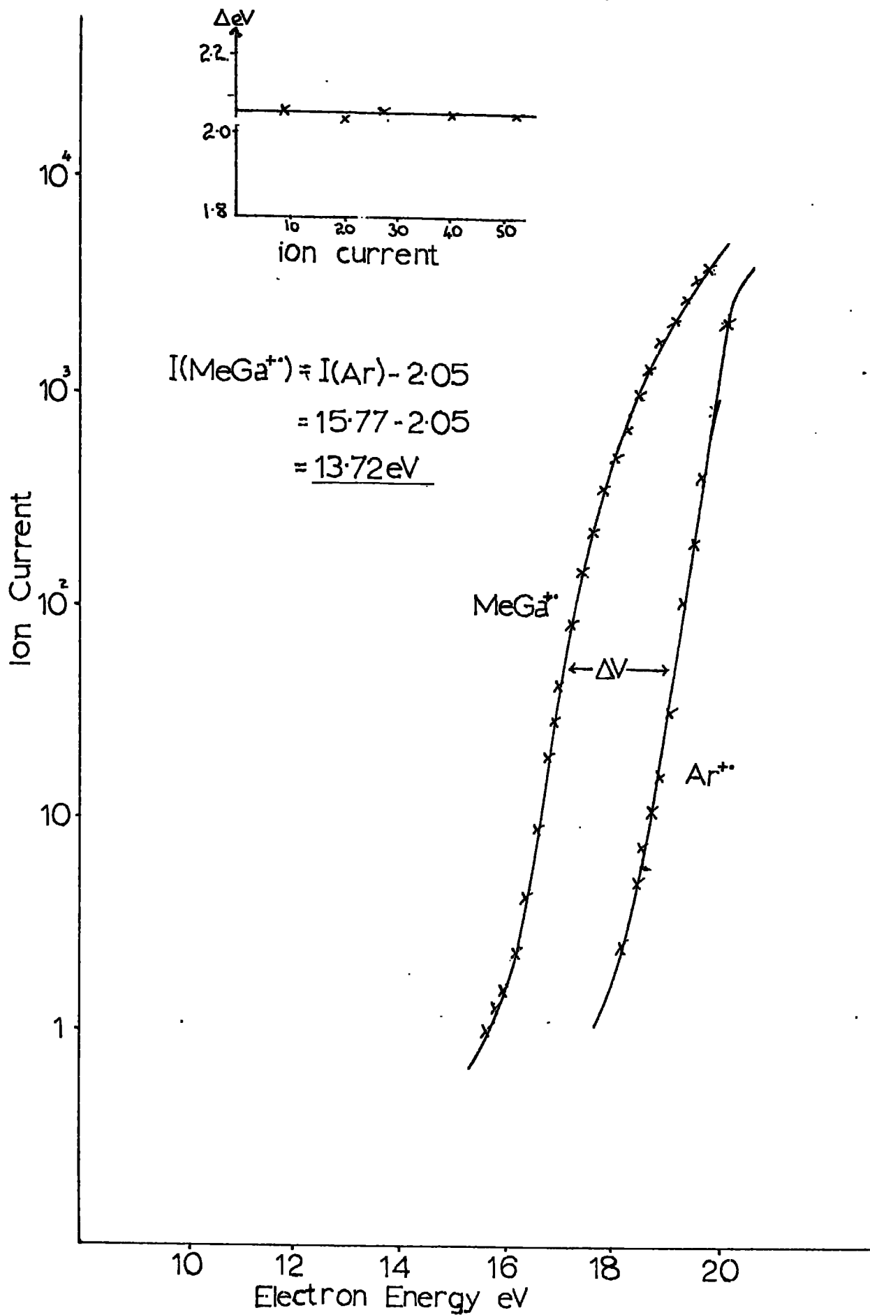
Fig. 14 Ionization Efficiency Curve for MeGa + and Ar +
