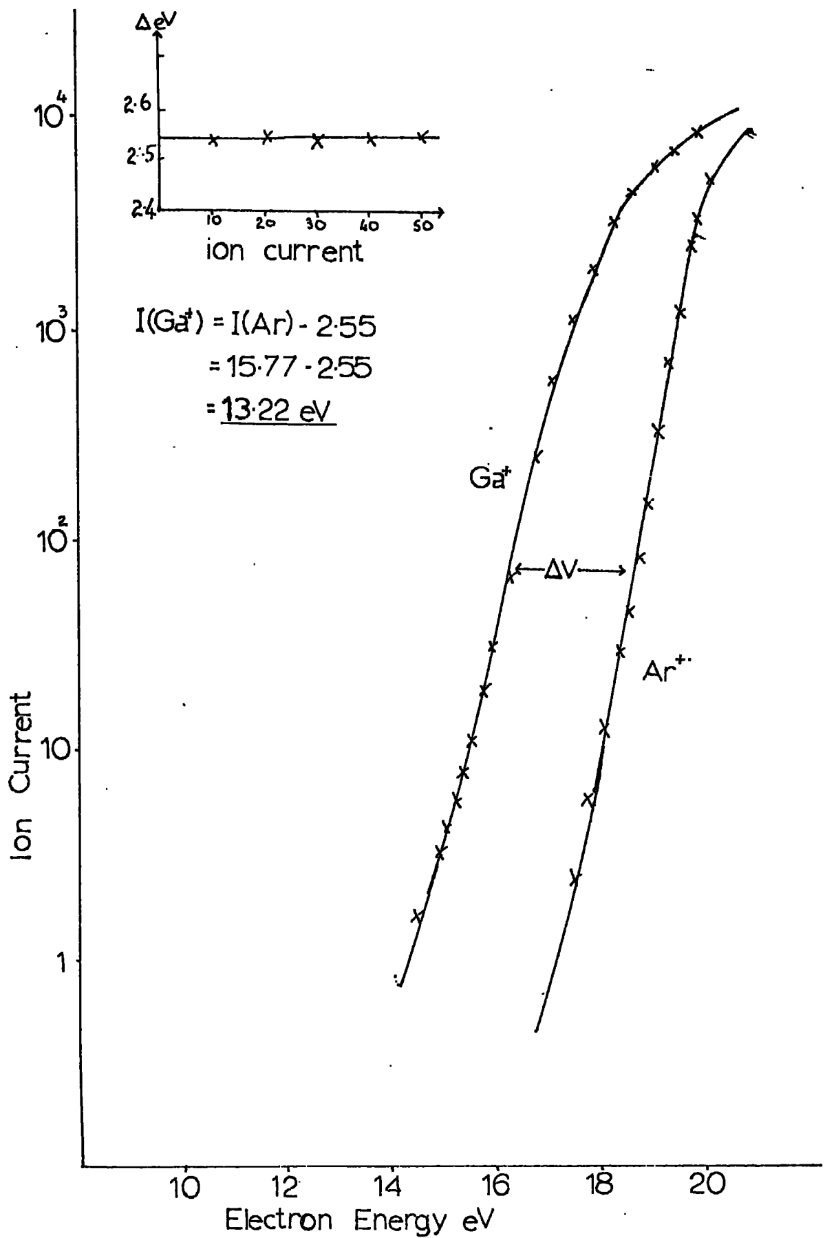
Fig. 15 Ionization Efficiency Curve for Ga + and Ar +
