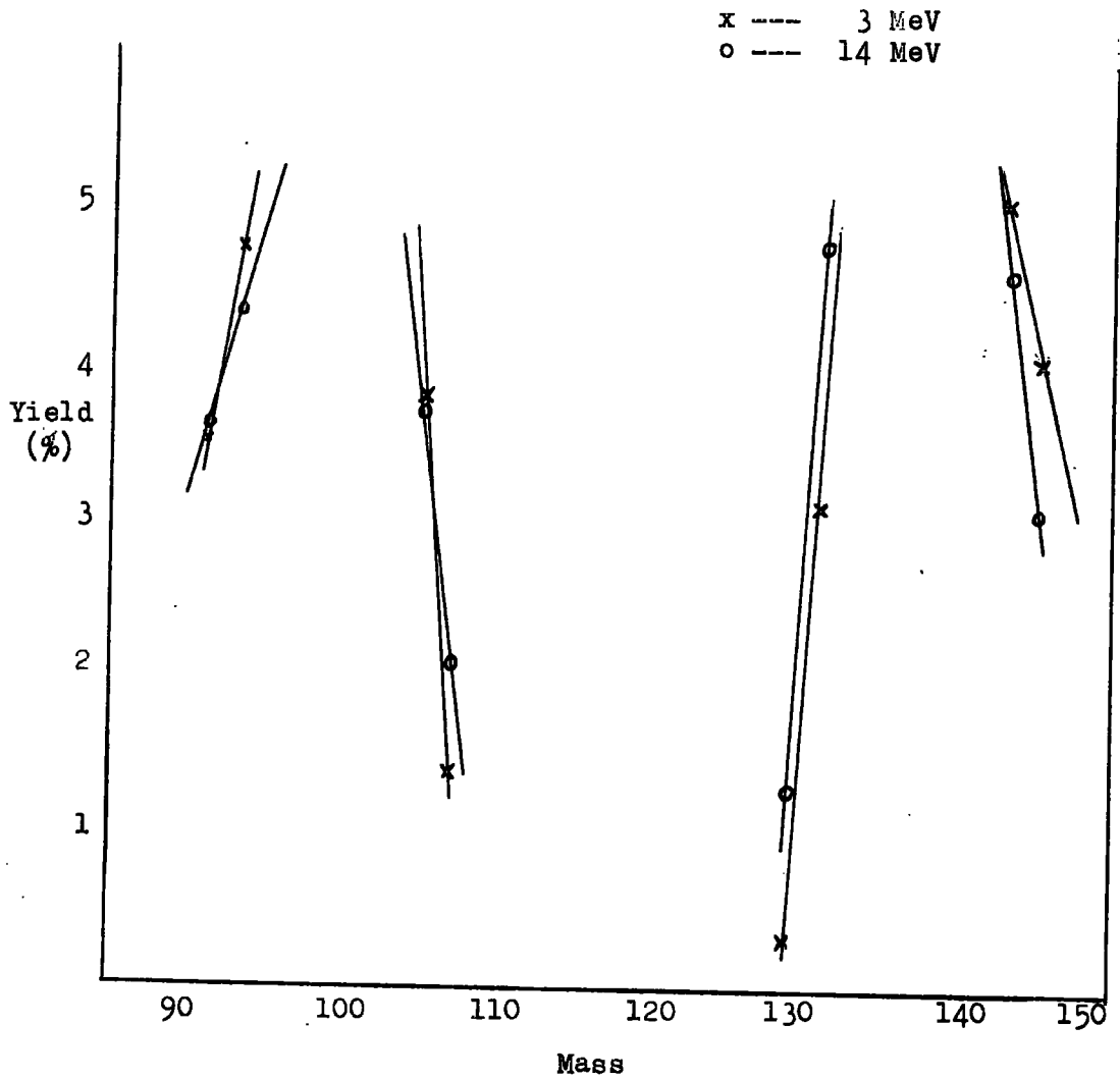
Comparison of Observed Mass-Yields of U^{238} excited by 3 MeV and 14 MeV neutrons.
