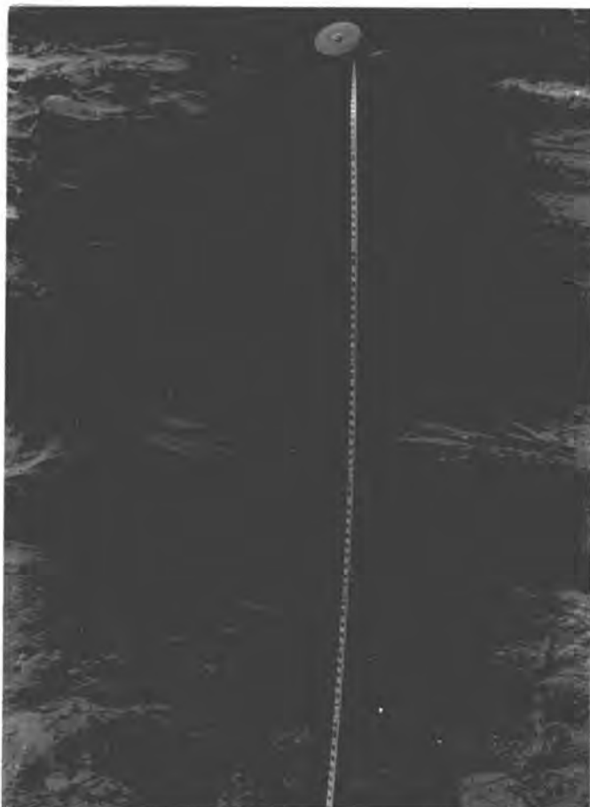
An exposure of a marginal lustrinal facies at Knockshield, East Allen Dale. Four siltier horizons are clearly seen to undulate in the form of giant ripples. When traced into the exposure the ripples showed no constant direction.
