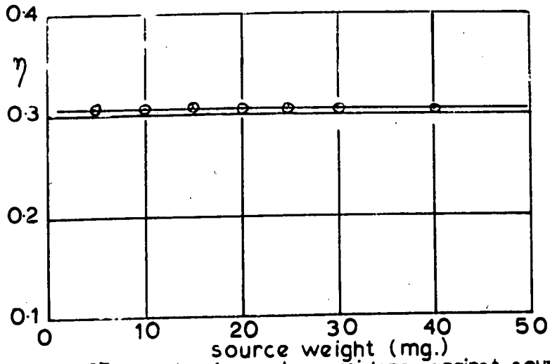
Fig.17 Graph of counter efficiency against source weight for ^{110}\text{Ag}
