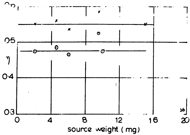
Fig.19 . Counter efficiency against source weight for ^{129}\text{Sb} .
