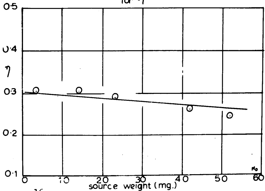
Fig.16 Graph of counter efficiency against source weight for ^{99}\text{Mo} .
