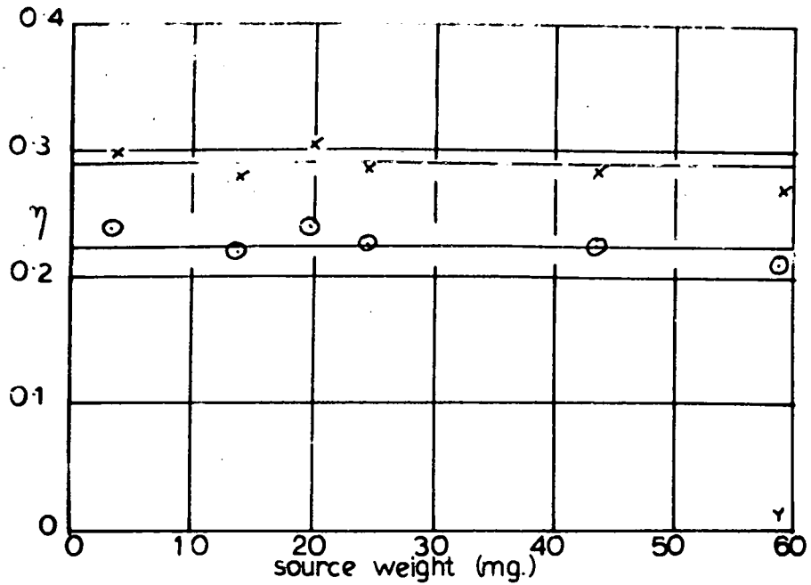
Fig.15 Graph of counter efficiency against source weight for ^{137}\text{Cs}
