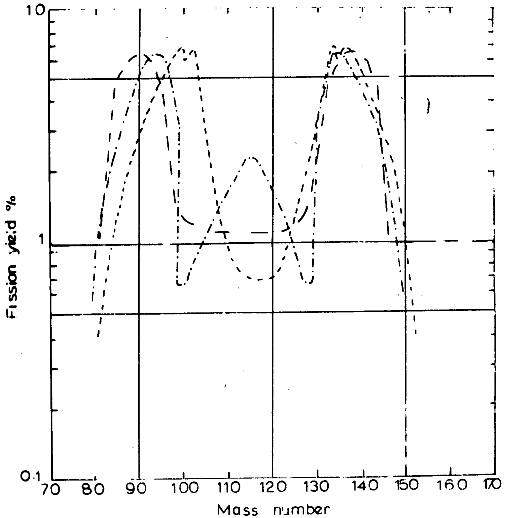
Fig.24. Mass distributions for fission induced by 14 MeV neutrons. ^{232}\text{Tn} (dashed line) ^{238}\text{U} (dash-dot line) ^{239}\text{Pu} (solid line)
