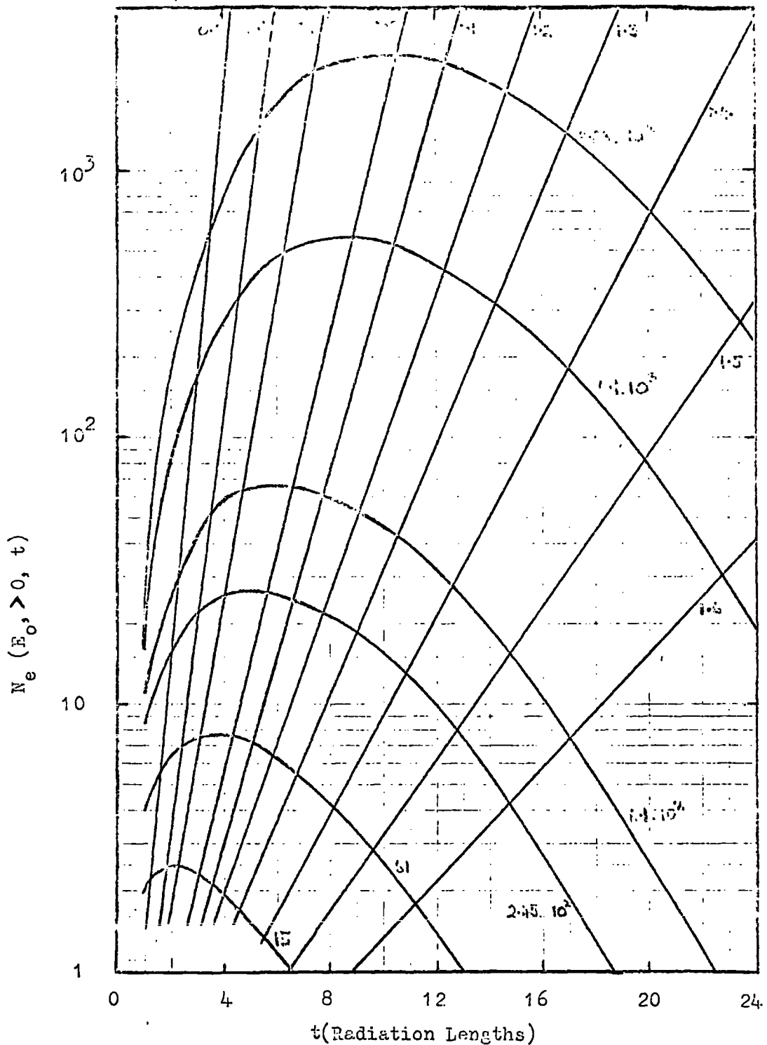
Figure 5.3 Shower development curves giving the total number of electrons as a function of depth for cascades initiated in iron by photons with energy E_0/E_0 = 15, 61, 2.45 \cdot 10^2, 6.1 \cdot 10^2, 6.1 \cdot 10^3, \text{ and } 3.23 \cdot 10^4 , according to Ivanenko et al (1958). The straight lines are loci of constant age parameter s .
