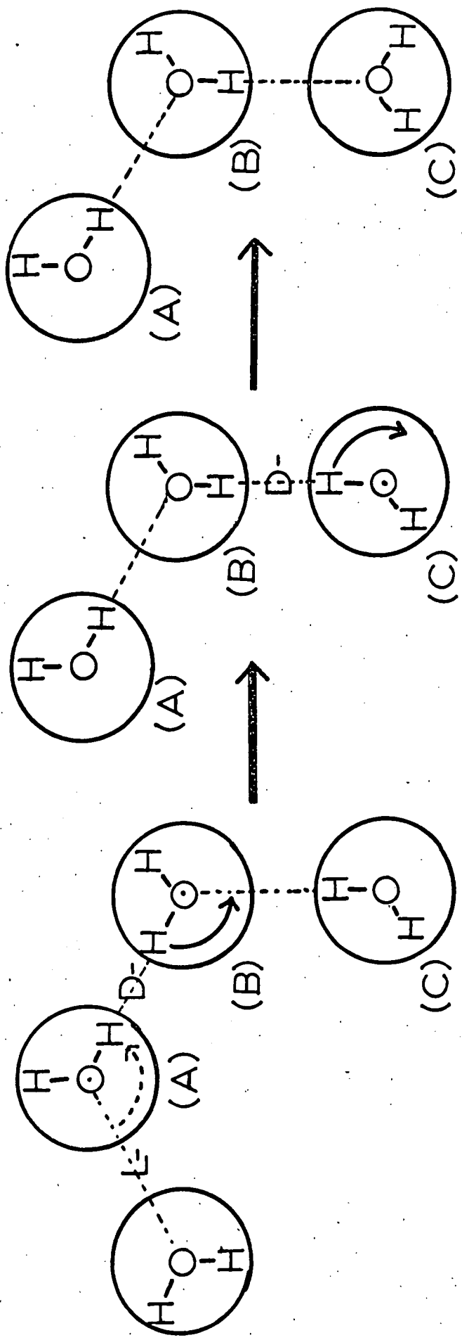
Fig. II.6. the generation & migration of Bjerrum defects in ice.
