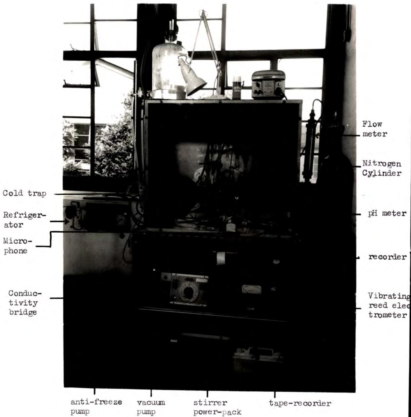
Fig.VII.8. A General View of the Apparatus.
