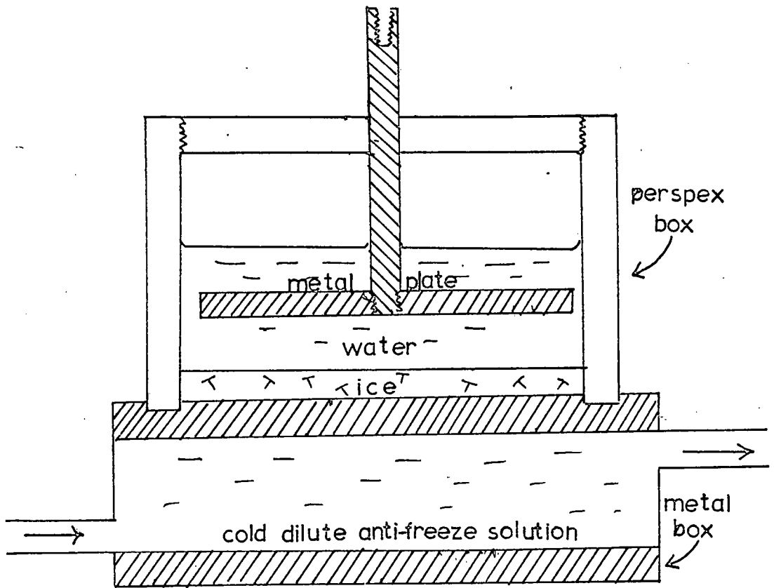
THE BASIC FREEZING CELL.
