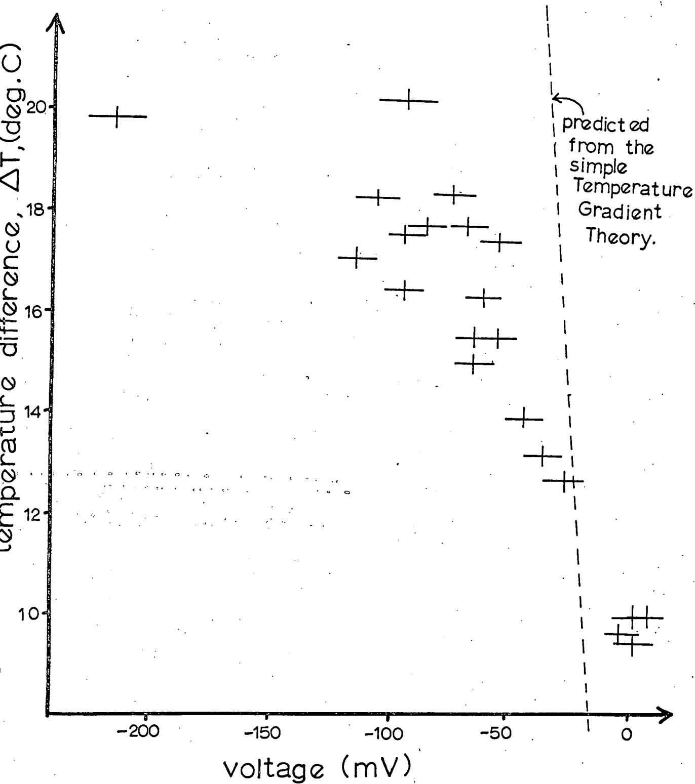
Fig. VI.12. GRAPH OF VOLTAGE AGAINST TEMPERATURE DIFFERENCE BETWEEN OPPOSITE FACES OF THE ICE IN THE FREEZING CELL. THE LIQUID PHASE WAS BEING STIRRED.
