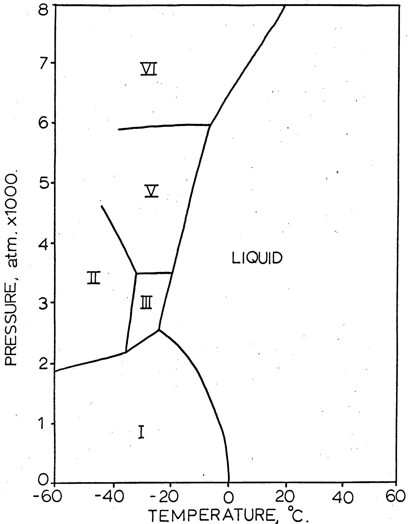
Fig.II.1. the polymorphism of ice.
