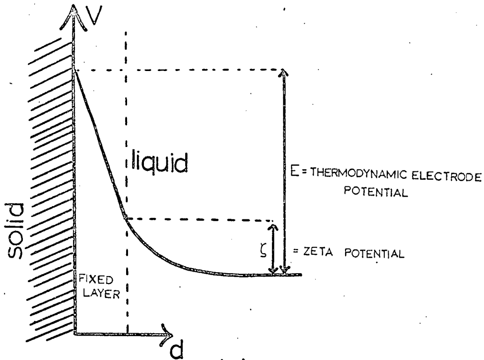
(a) ions of same sign in both layers.
