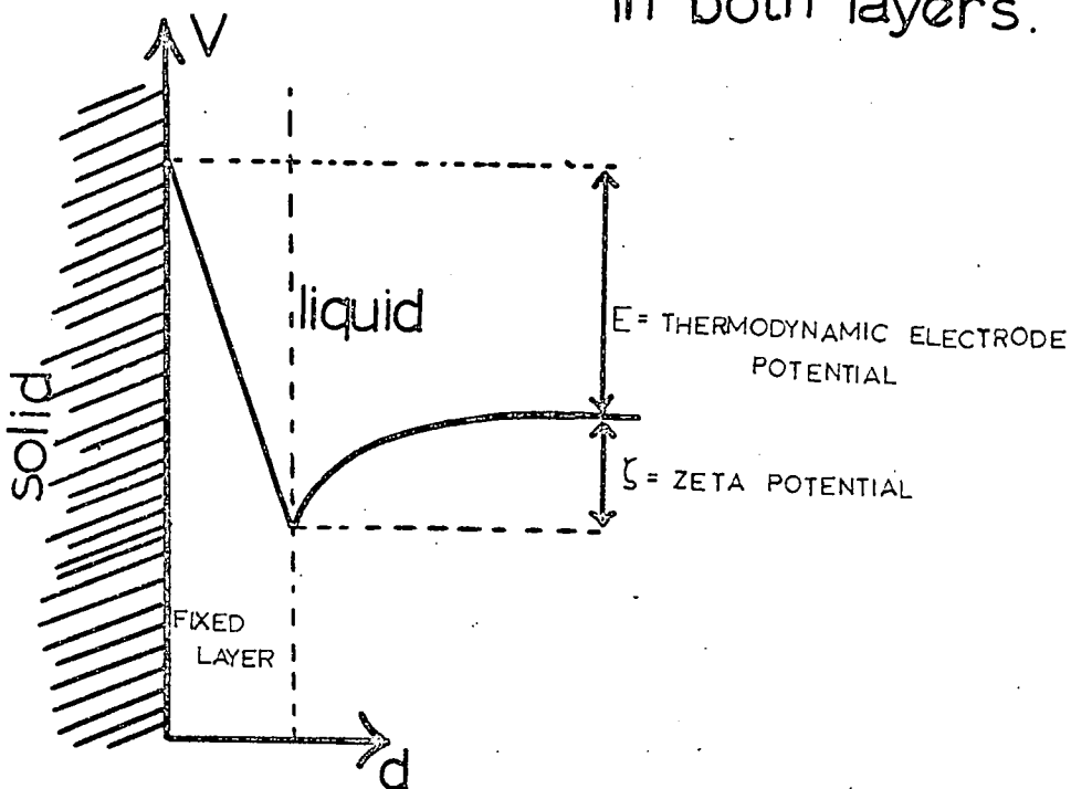
(b) ions of opposite sign in each layer.
