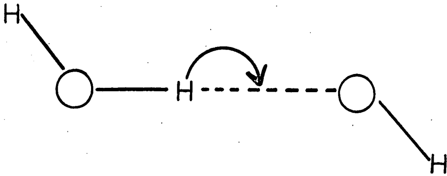
Fig. II.4. the "Proton-jump" mechanism of charge transport in water.
