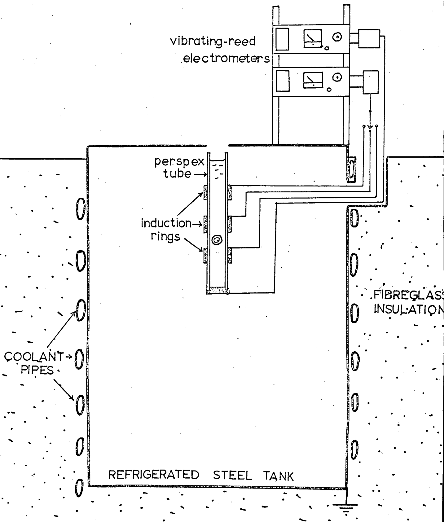
Fig. V.1. APPARATUS FOR DETERMINING THE CHARGE ON ICE-COATED SPHERES, FALLING THROUGH WATER.
