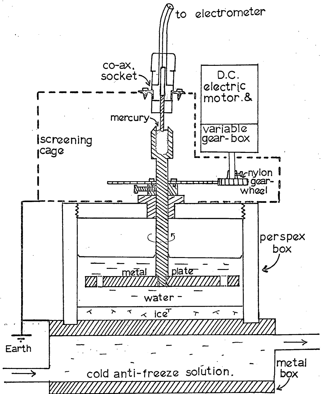
The freezing cell.
