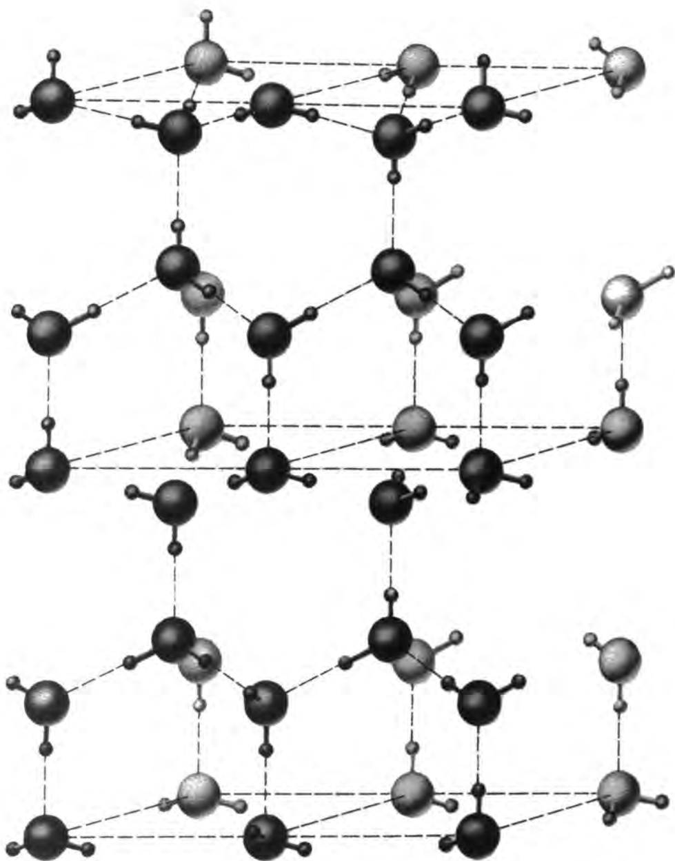
Fig. II.3 The arrangement of molecules in the ice crystal. The orientation of the water molecules as represented in the drawing is arbitrary; there is one proton along each oxygen-oxygen axis, closer to one or the other of the two oxygen atoms. [Linus Pauling, The Nature of the Chemical Bond , Cornell University Press, 1960]
