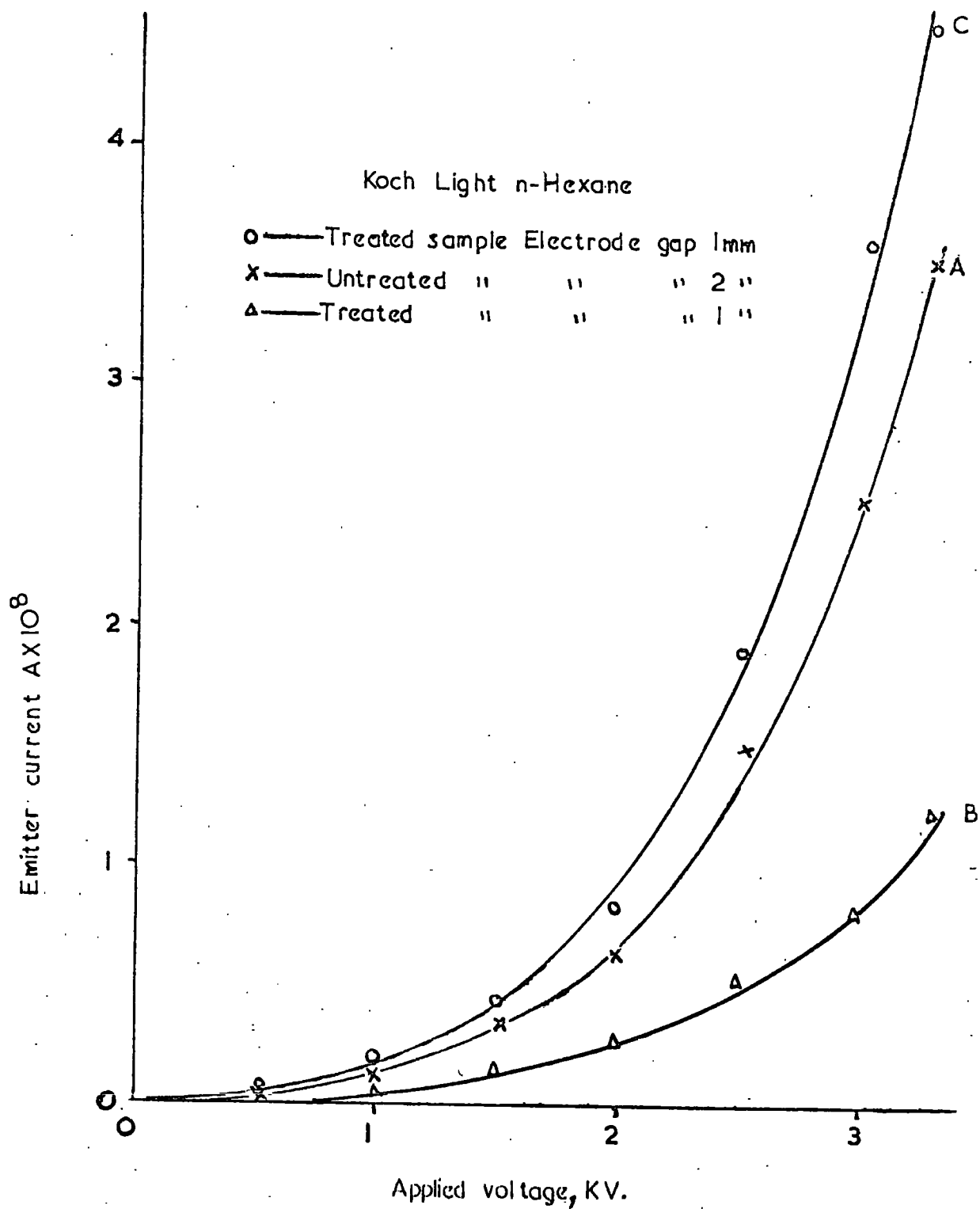
Figure 5.5 Variation of emitter current with applied voltage for an array of six blades in Koch-light n-hexane. Blades are cathode.
