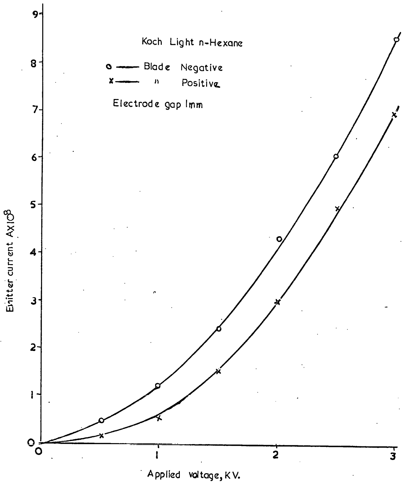
Figure 5.6 Showing the effect of polarity on emitter current from six blades to a plate electrode.
