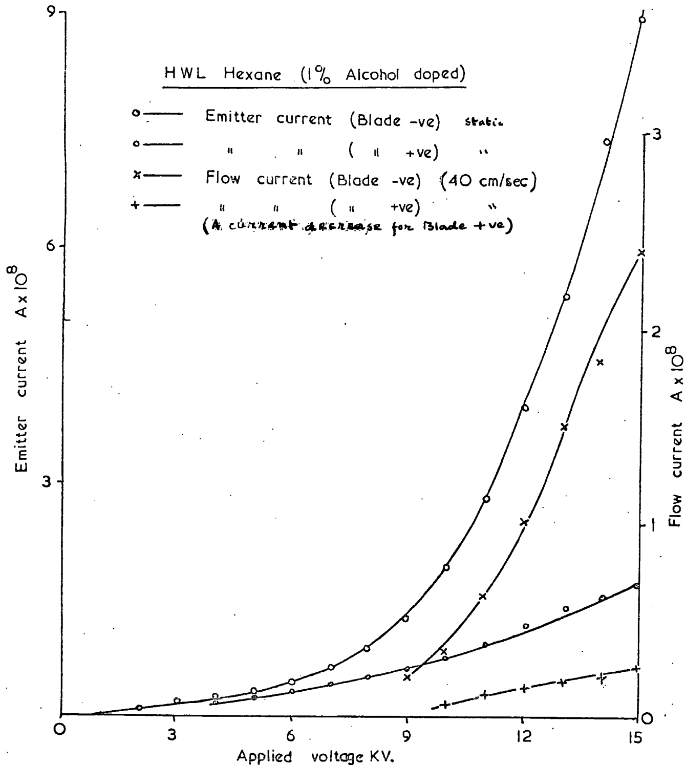
Figure 5.29 Variation of emitter current and flow-current with applied voltages in 1% alcohol doped HWL hexane with Wilkinson blade.
