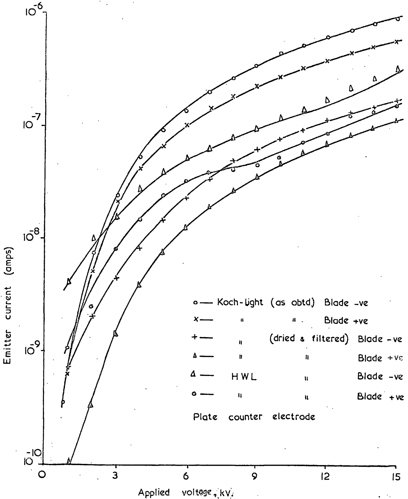
Figure 5.31 Static emitter current characteristics for different grades of hexane with Blue Gillette blade.
