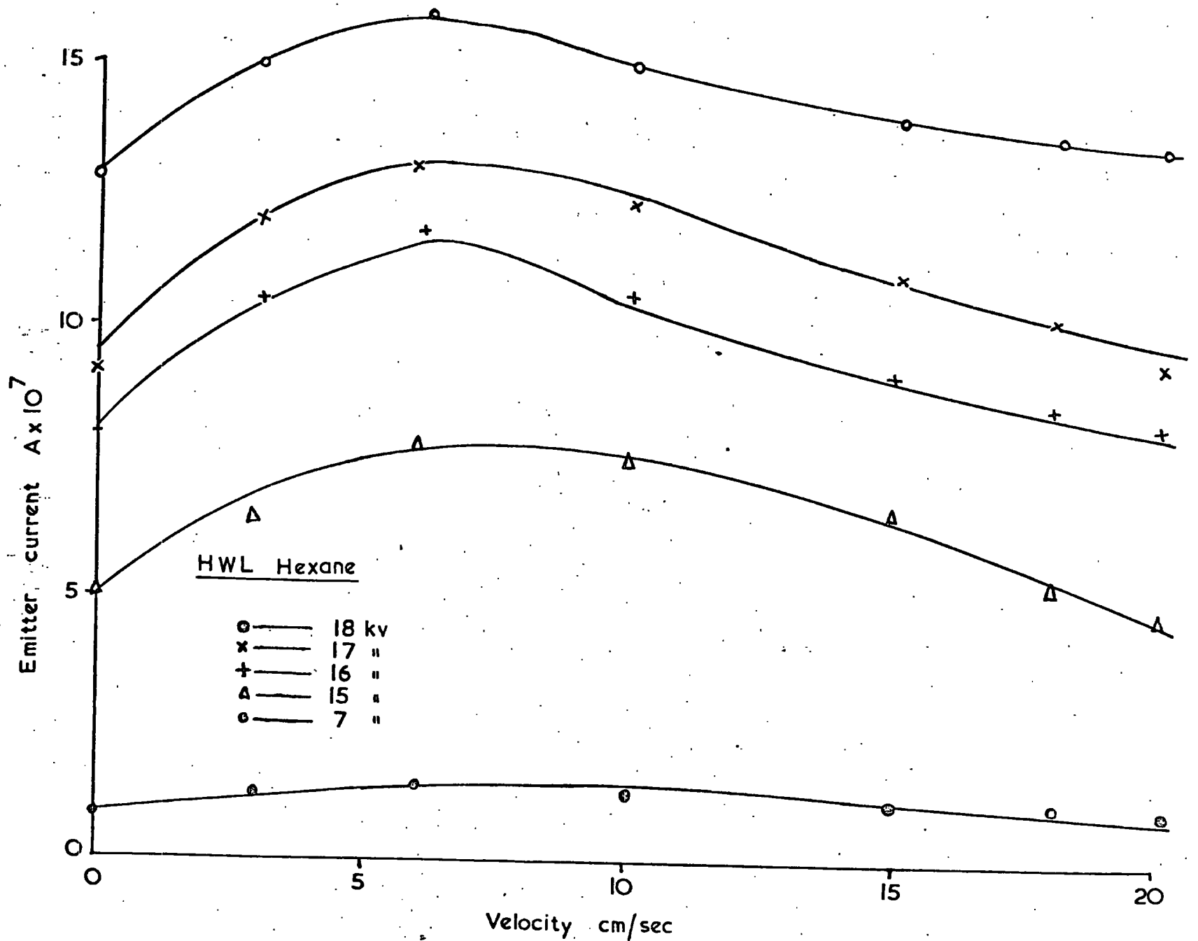
Figure 5.14 Variation of emitter current with liquid velocity in hydrated HWL hexane.
