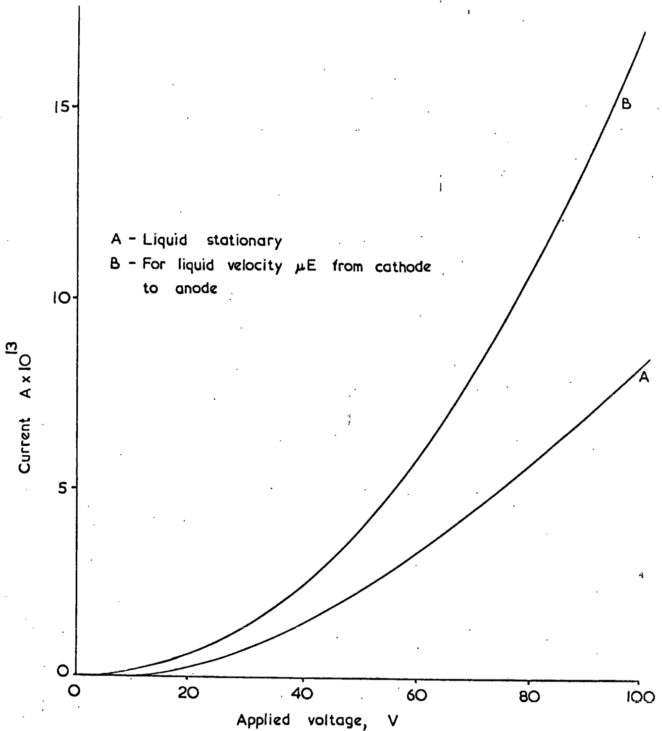
Figure 6.1. Theoretical variation of space charge limited current with applied voltage for stationary and moving liquid.
