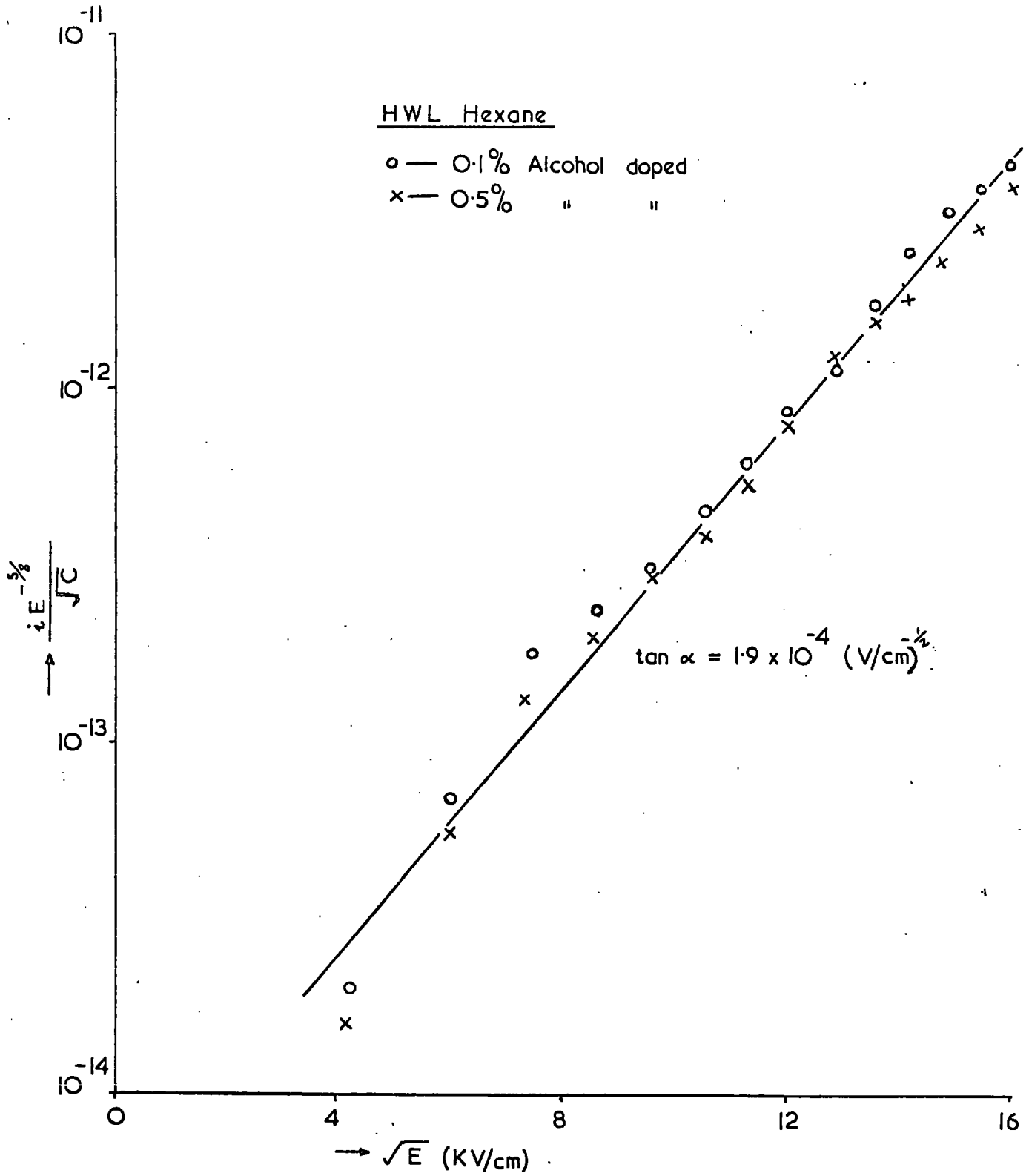
Figure 7.3. Variation of impurity current with applied field in alcohol doped hexane.
