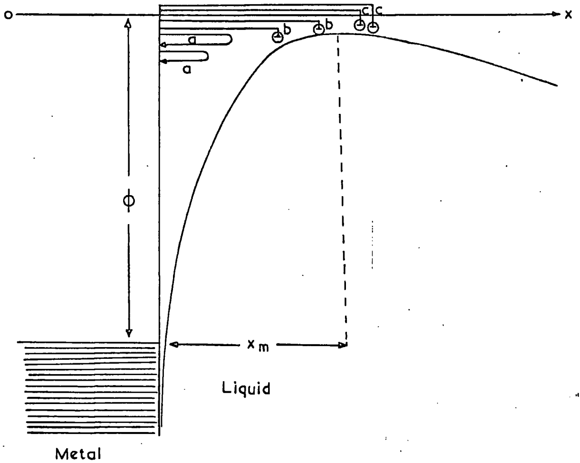
Figure 6.3. The image barrier into a dielectric for low applied field
