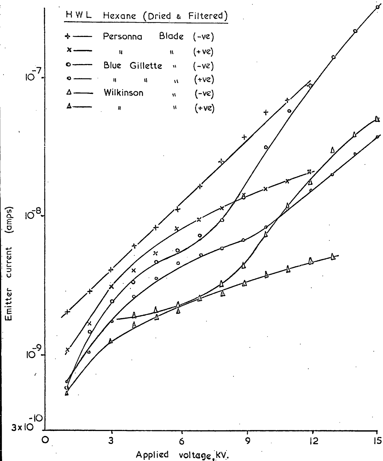
Figure 5.30 Static emitter current characteristics for various blades.
