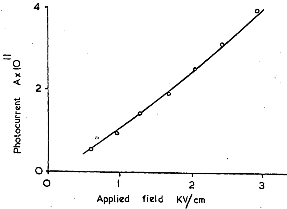
(a) Variation of photocurrent with applied field (Ref. 2)
