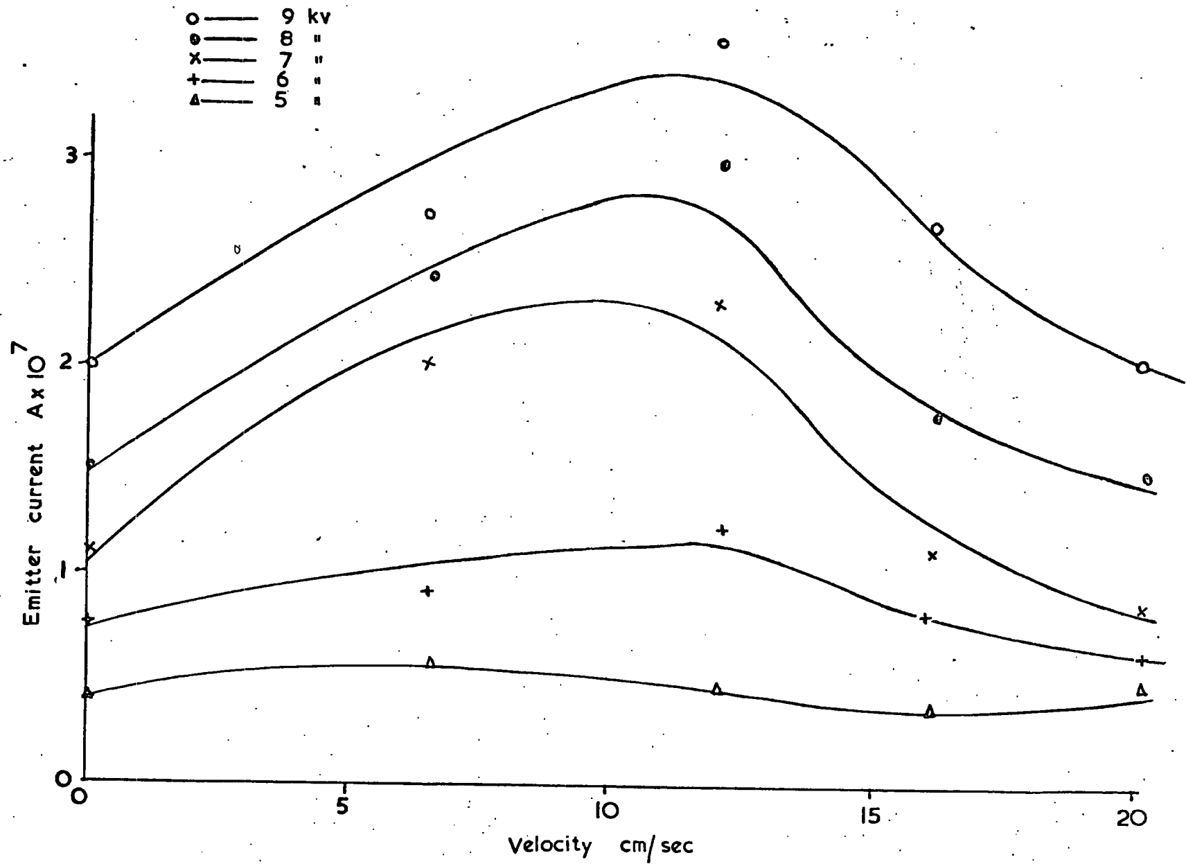
Figure 5.9 Initial results on the variation of emitter current with liquid velocity for different applied voltages.
