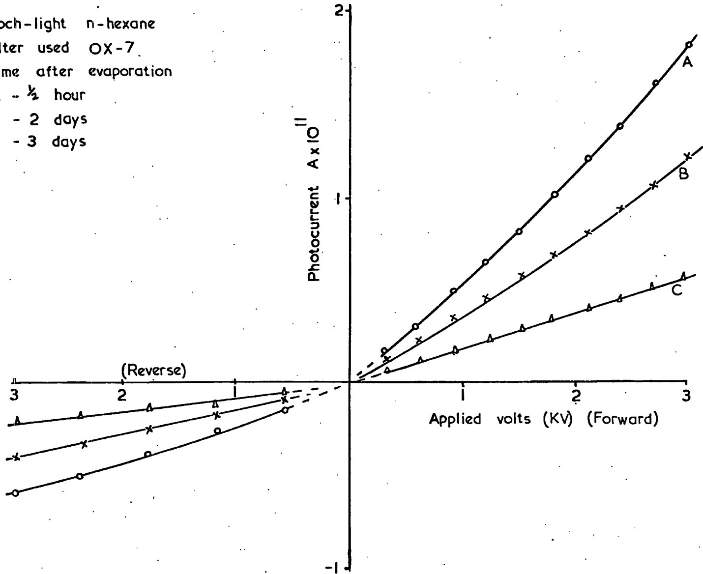
Figure 4.13 Variation of photocurrent with applied voltage
