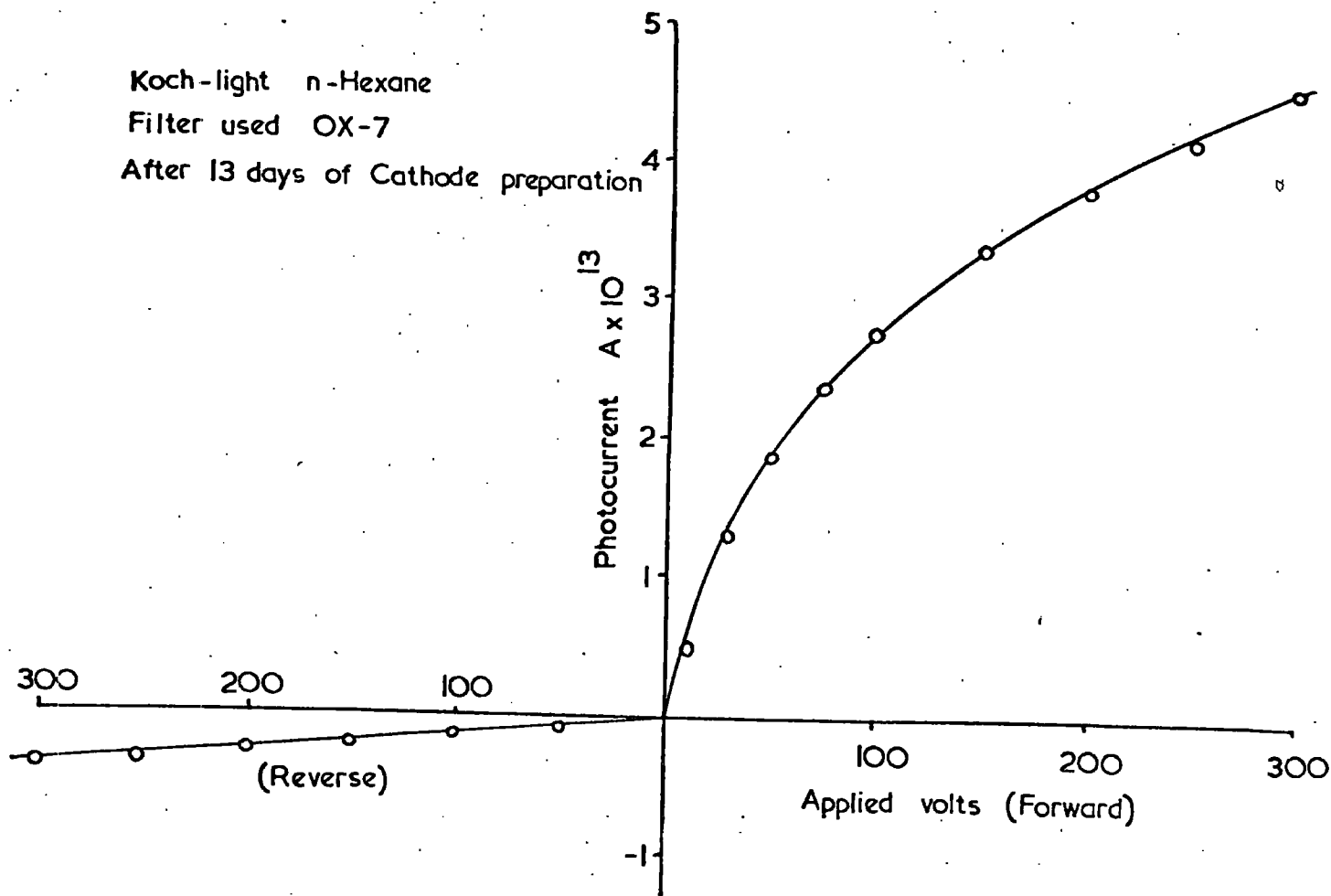
Figure 4.11 Variation of photocurrent with applied voltage
