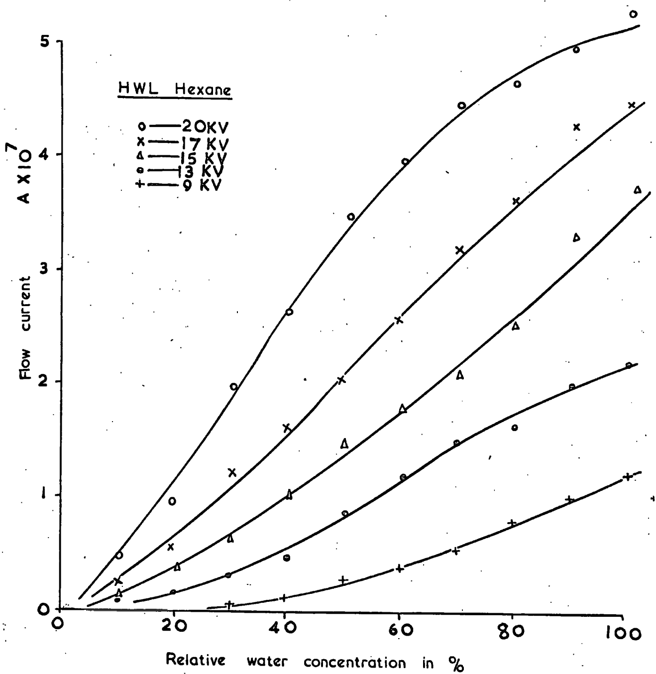
Figure 5.16 Variation of flow current with water content in HWL hexane. The liquid velocity = 10 cm/sec.
