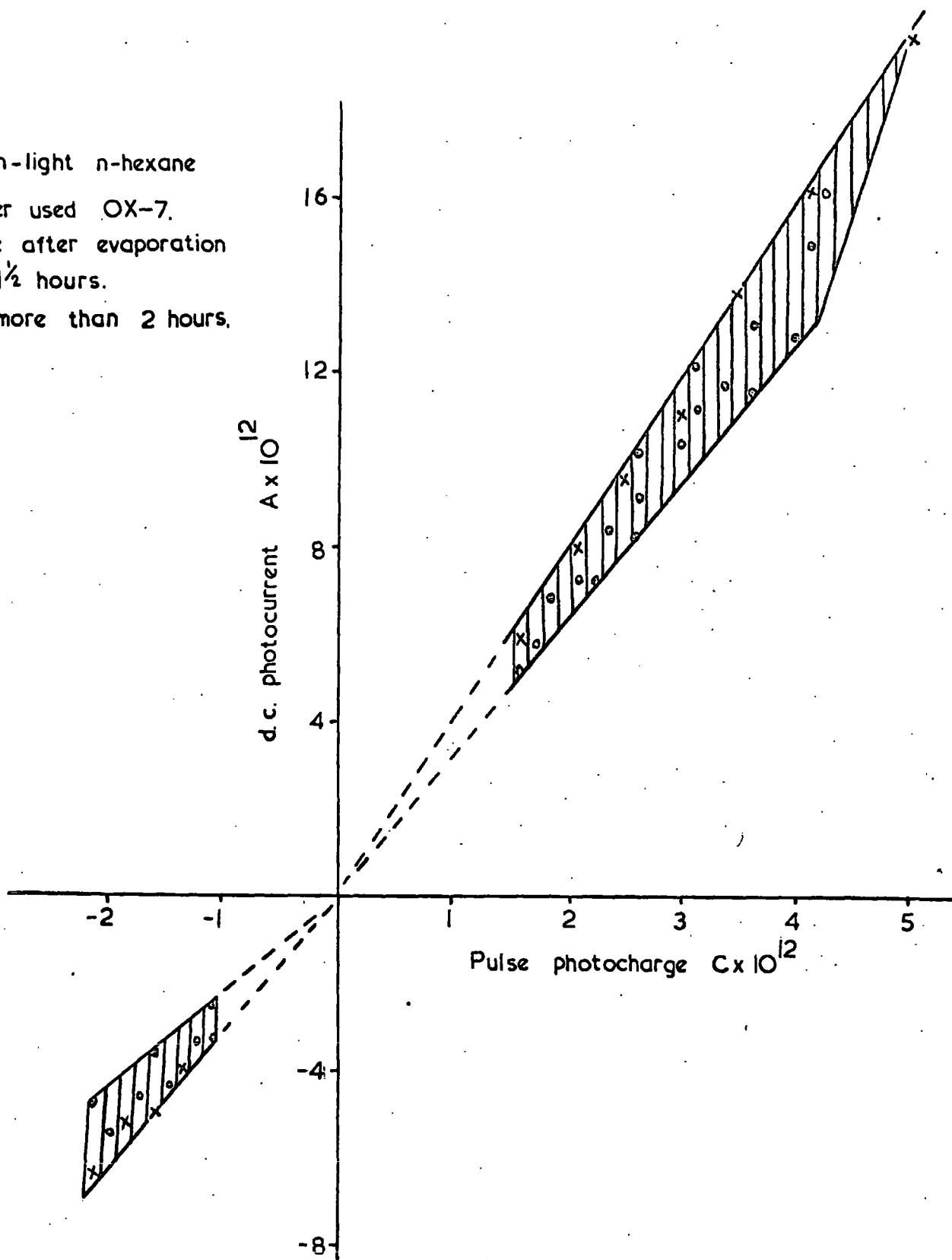
Figure 4.17 Variation of d.c. photocurrent with pulse photocharge. Shaded regions indicate the magnitude of experimental scatter.
