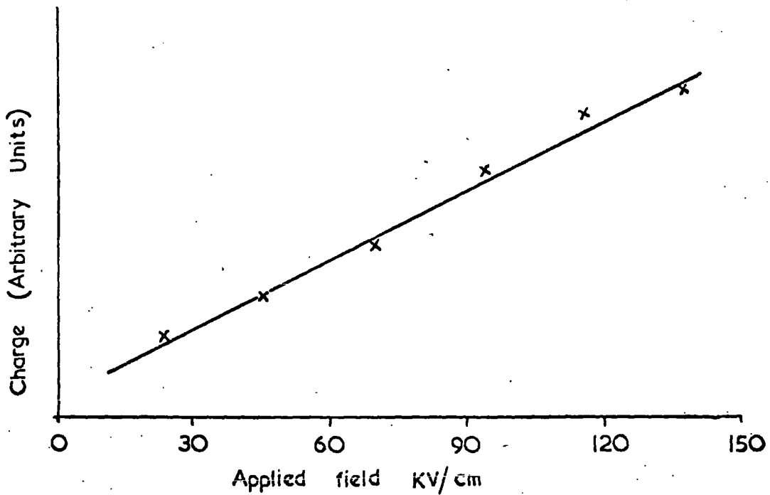
(b) Variation of photocharge with applied field (Ref. 3)
