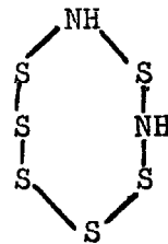
(c) m.p. 130^{\circ}
