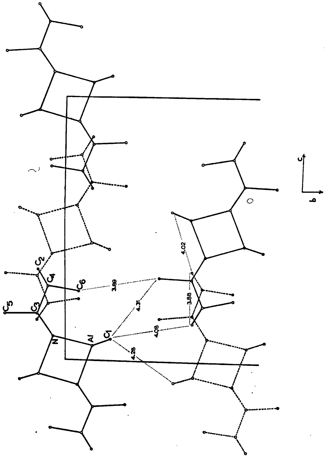
(\text{Bu}^t\text{MeCNAiMe}_2)_2 100 projection
