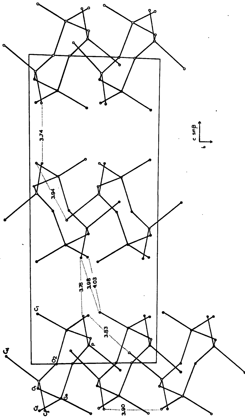
(\text{Me}_2\text{GaO}_2\text{PMe}_2)_2 100 projection
