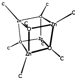
(MeZnOMe)_4 H.M.M. Shearer & C.B. Spencer Durham, 1965
