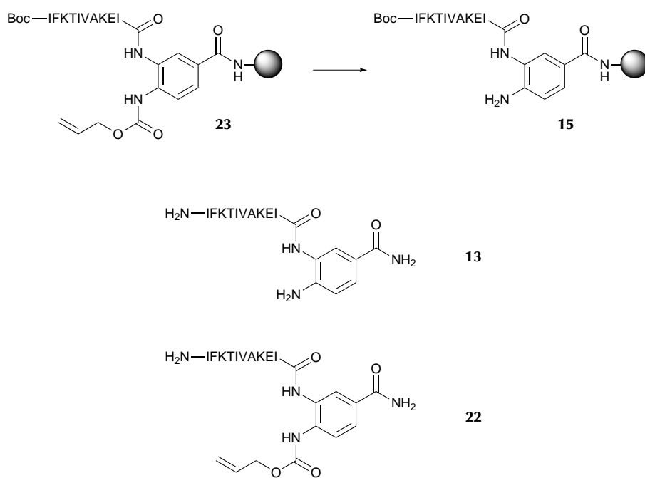
Scheme 3.4: Removal of the Alloc group from the Dbz linker. Reagents and conditions: \text{PhSiH}_3 (20 equiv), \text{Pd}(\text{PPh}_3)_4 (0.35 equiv), DCM, rt, 30 min. Uncyclized products 13 and 22 ( m/z = 1294.7 and 1378.7 respectively - spectrum C , Figure 3.1) observed following TFA cleavage from the resin are also shown.
