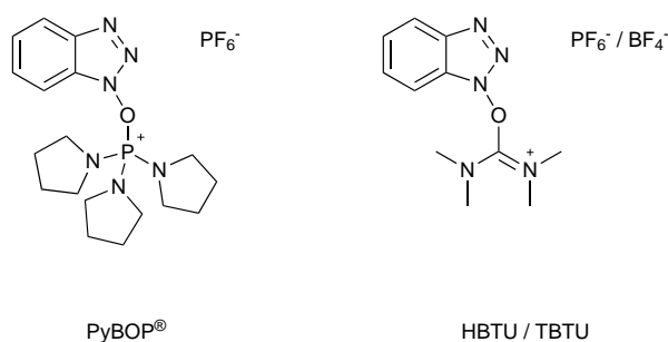
Figure 2.4: The coupling reagents PyBOP ® , HBTU and TBTU. The last two differ only in their counterion, which has no influence on the reactivity. 32
