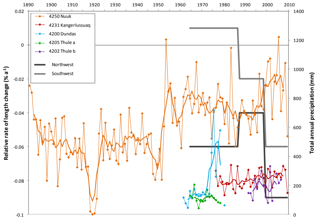
Figure 5.6: Graph showing mean relative rate of glacier length change measured at 4 time steps between 1964 and 2009 (grey lines), and precipitation data (coloured lines), during the twentieth century. Glacier data are based on samples of 33 northwest and 42 southwest glaciers. The solid coloured lines are the 5-year moving averages.
