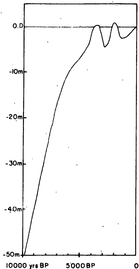
Sea level change in the Fenlands of East Anglia
