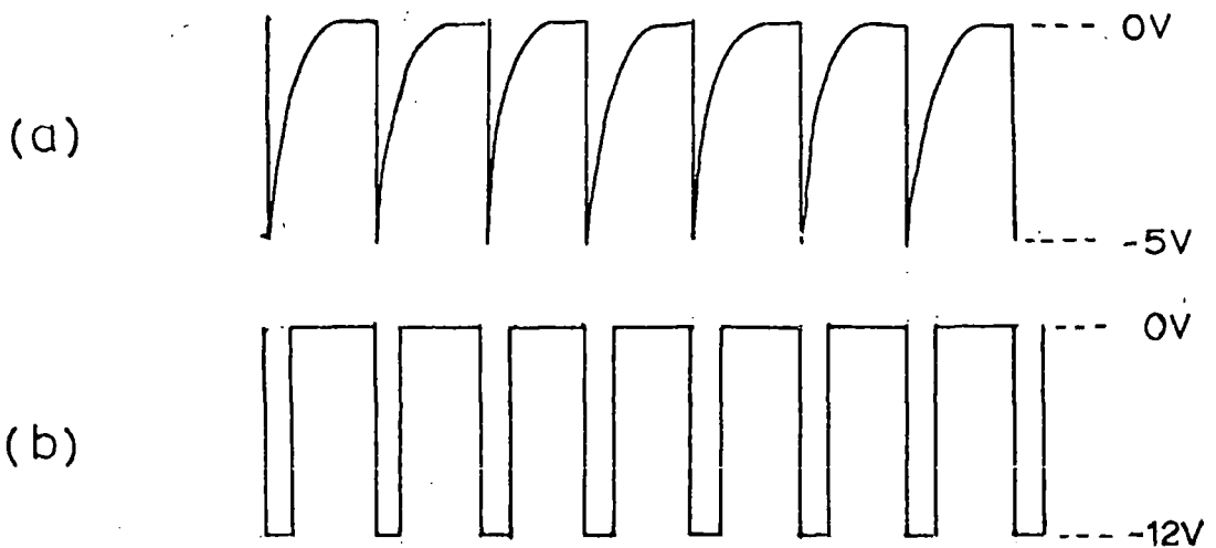
(b) The monostable circuit output
