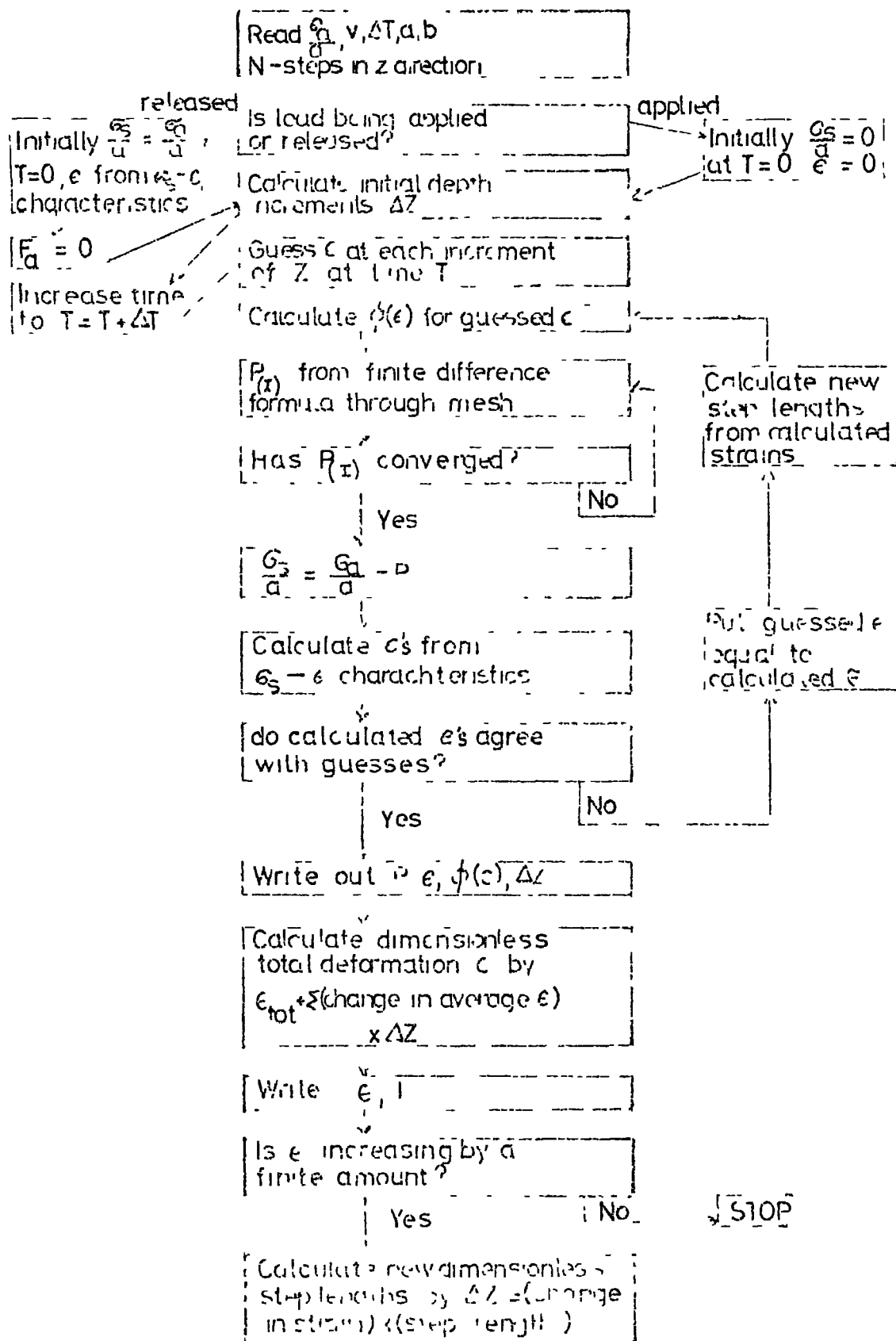
FIG 3 2 FLOW DIAGRAM FOR DIMENSIONLESS AXIAL FLOW PROGRAMME
