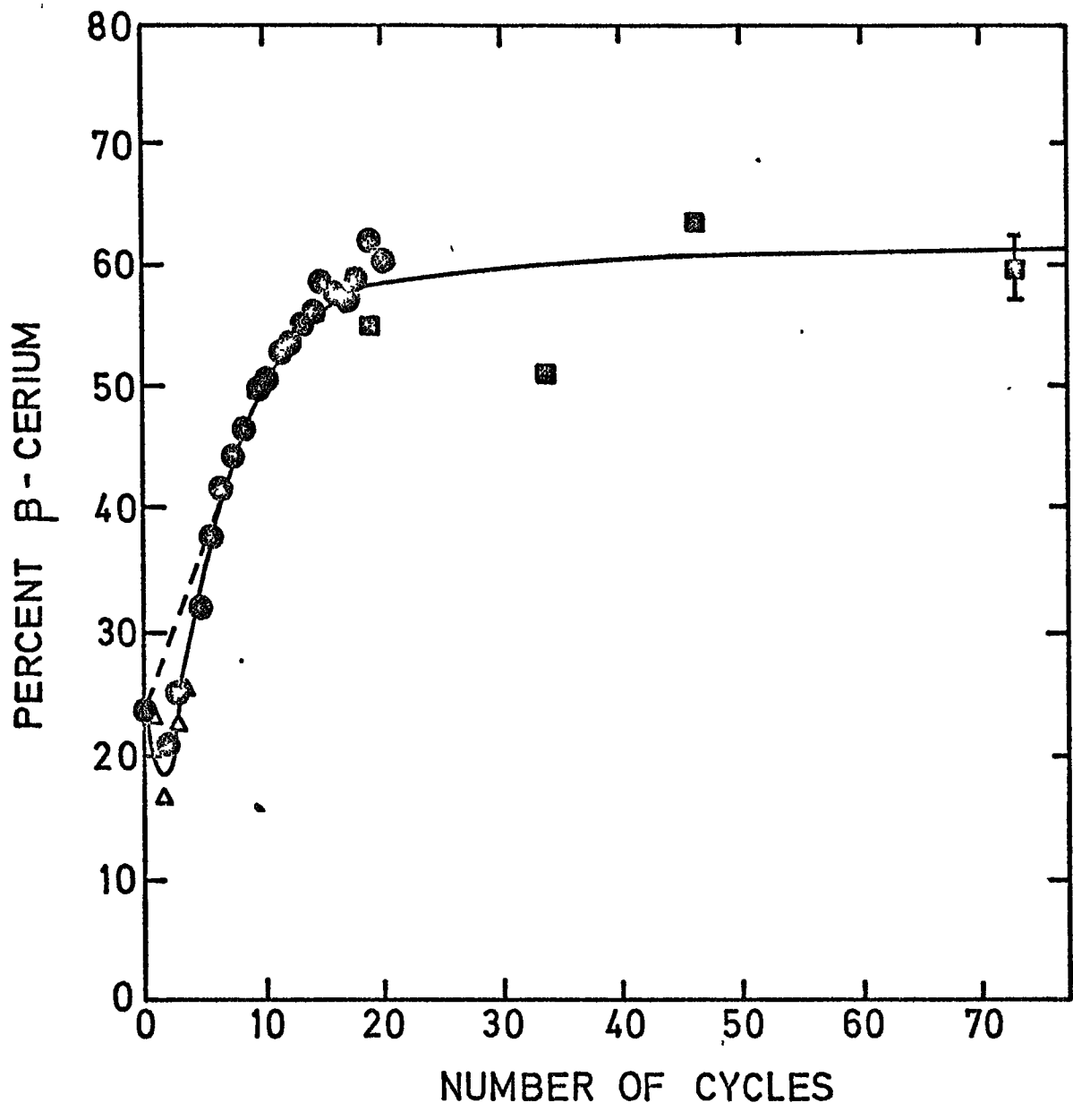
Fig. 3.4: Effect of cycling on the amount of \beta -cerium present in the sample. ● Dilatometric data; \Delta dilatometric data for a second Ce sample from the same manufacturer, ■ X-ray data. [Gschneidner et al. 1962].
