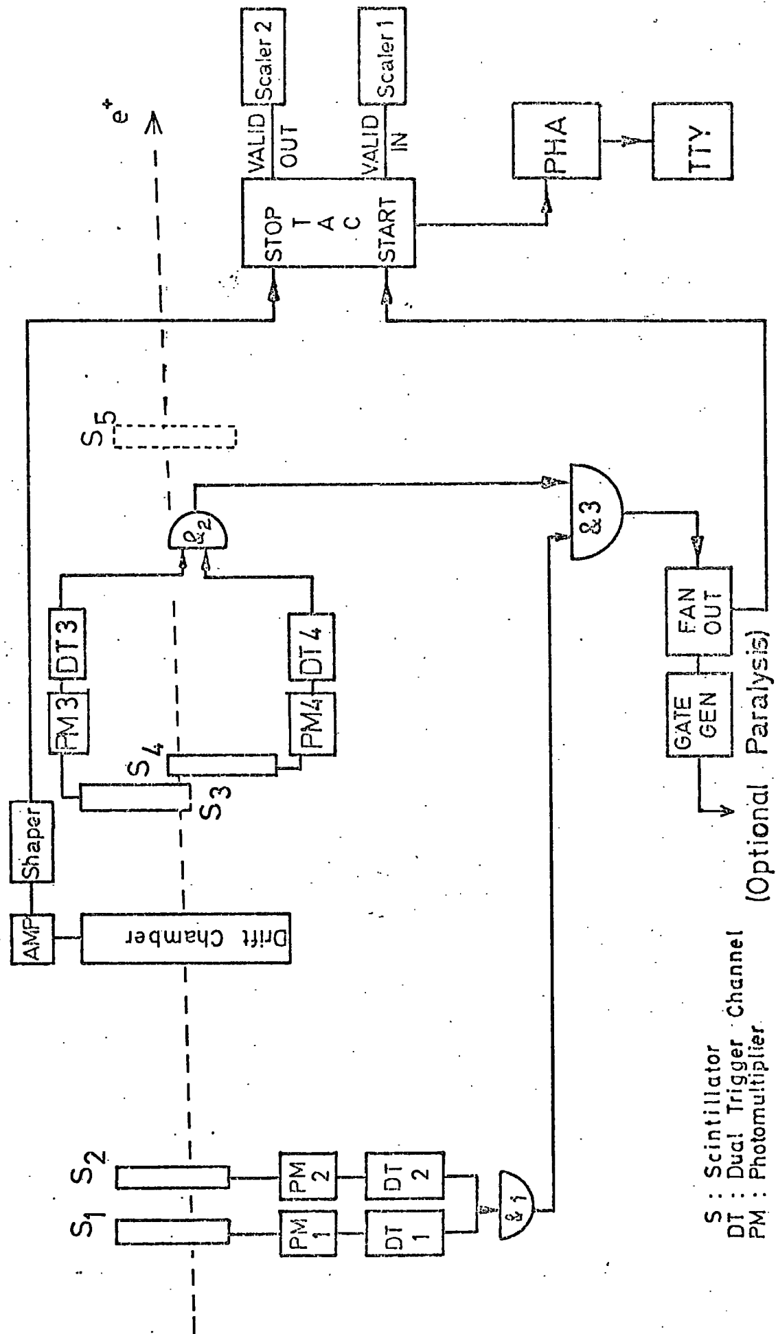
FIG. 5.2: Data Acquisition System for One Chamber (System 1) -
