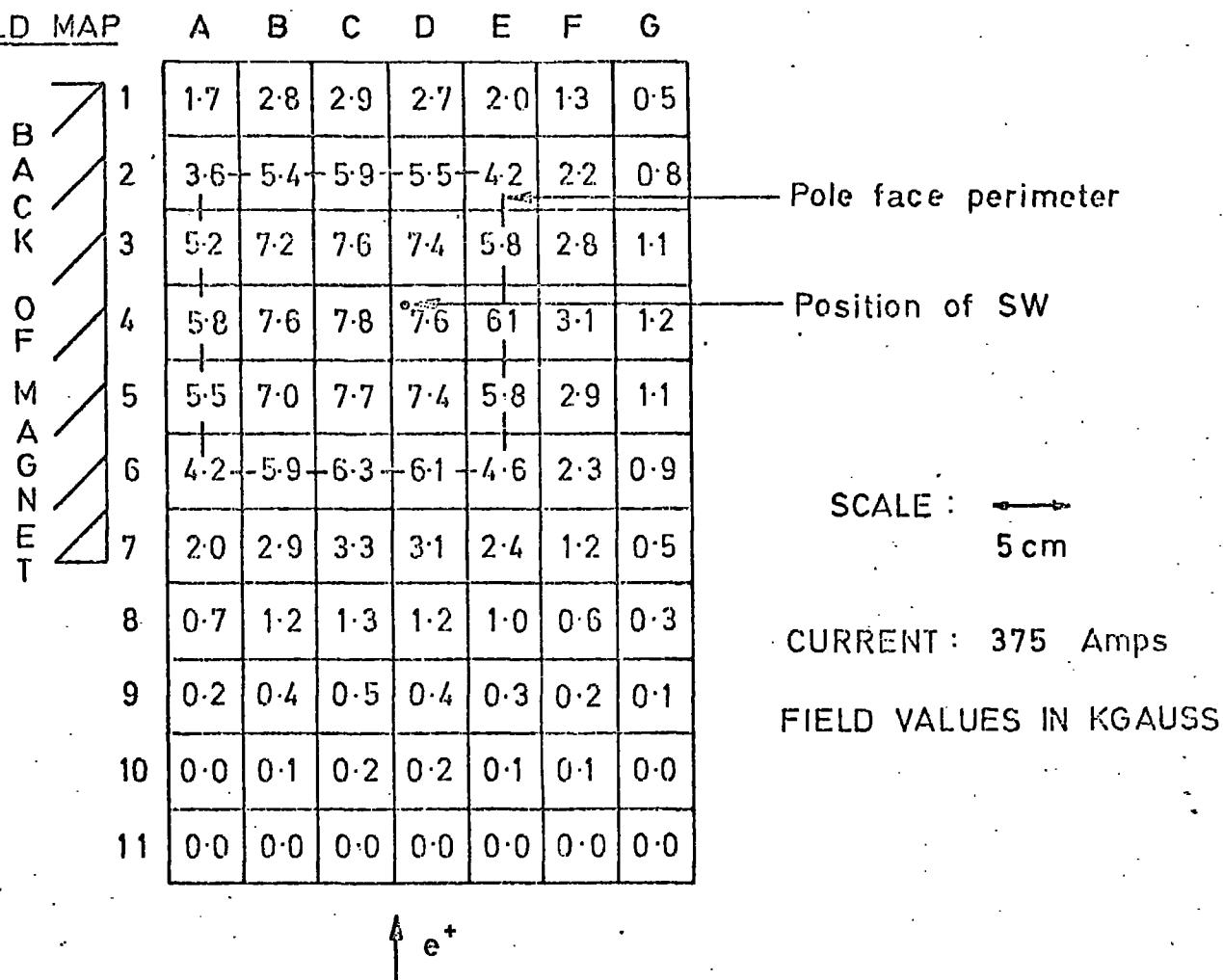
FIG.5.6b MAGNETIC FIELD VS POSITION
