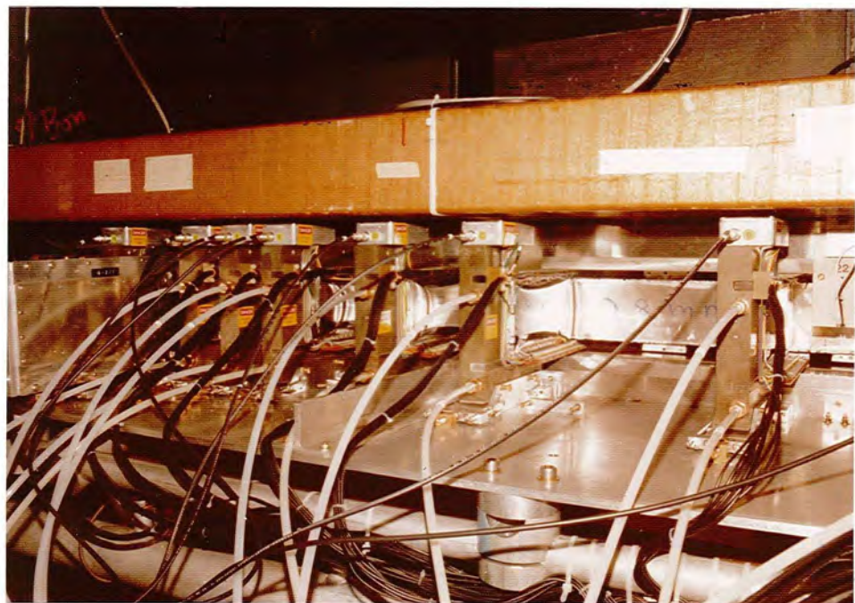
FIG 7.13(b) THE g-2 DRIFT CHAMBERS MOUNTED BETWEEN THE MAGNET POLE PIECES IN THE REGION OF THE THIN-WALLED VACUUM STORAGE TANK
