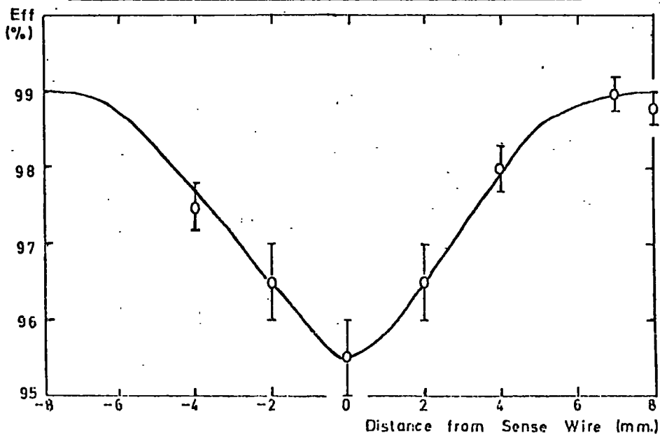
FIG 5.9 EFFICIENCY SCAN ACROSS SENSE WIRE
