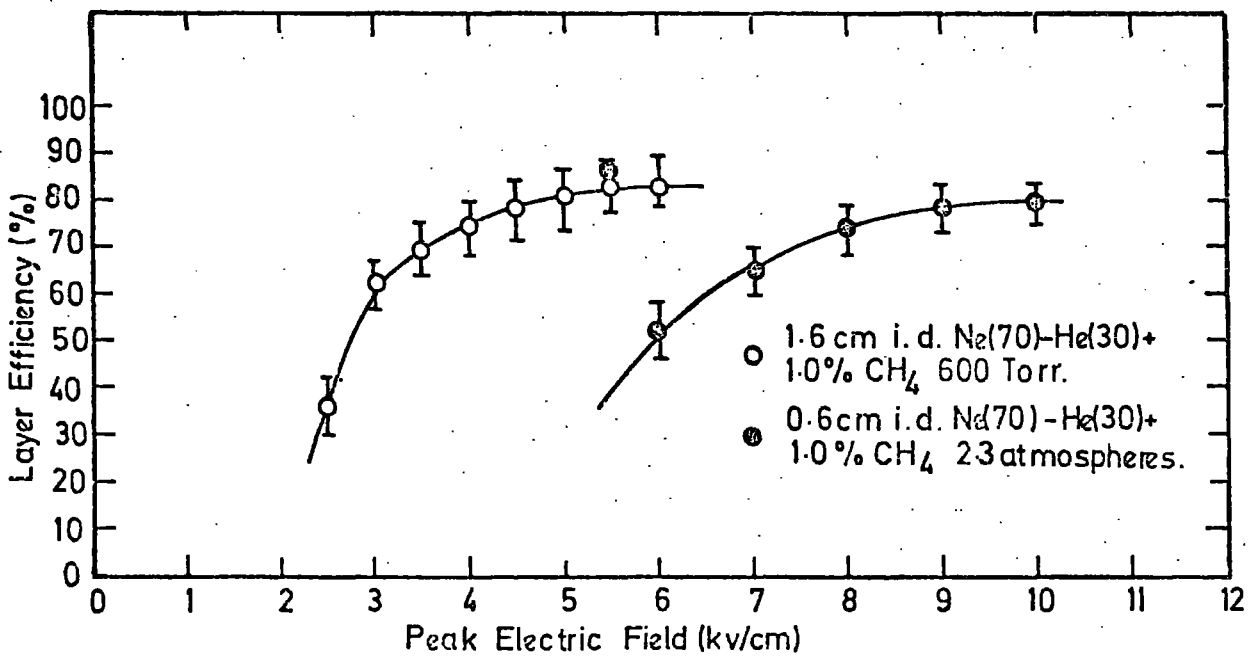
FIG. 5-20 Layer Efficiency versus Field Strength for Ne(70)-He(30)+1.0% CH 4 H.T. RC=2μs
