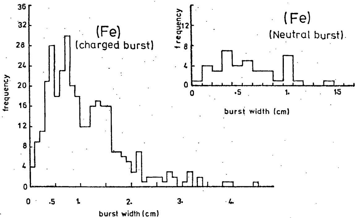
Figure 7.1 The measured burst width distributions obtained below the lead and iron absorber. From 12,057 events selected by the local density trigger where \Delta\epsilon \geq 40 \text{ m}^{-2} . See Table 7.1(a) for further details. For the true burst width, multiply by 20.
