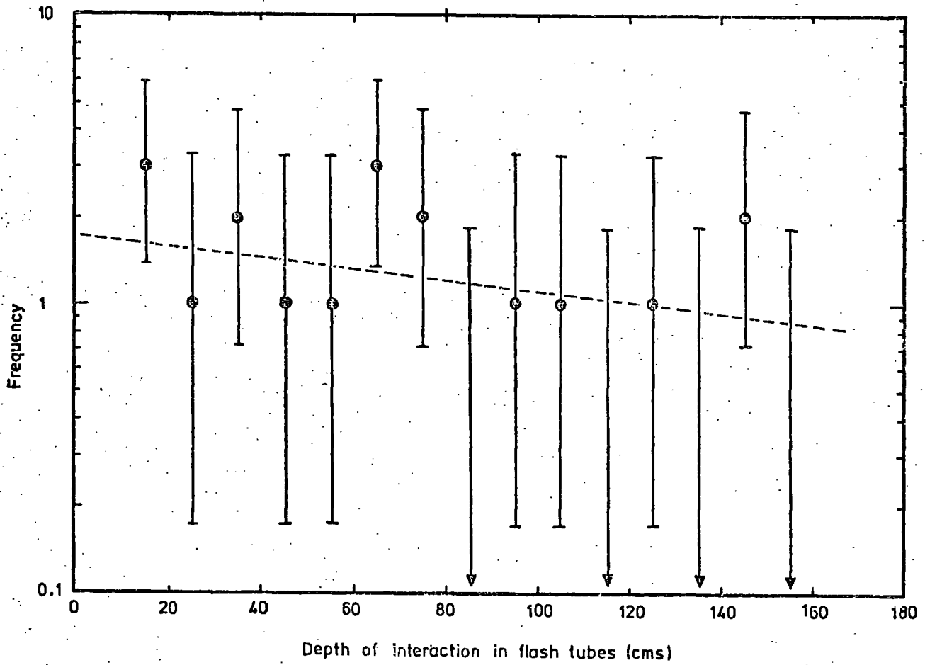
Figure 7.7 The interaction length of neutral particles in the flash tubes. \lambda = 115 \text{ g.cm}^{-2} .
