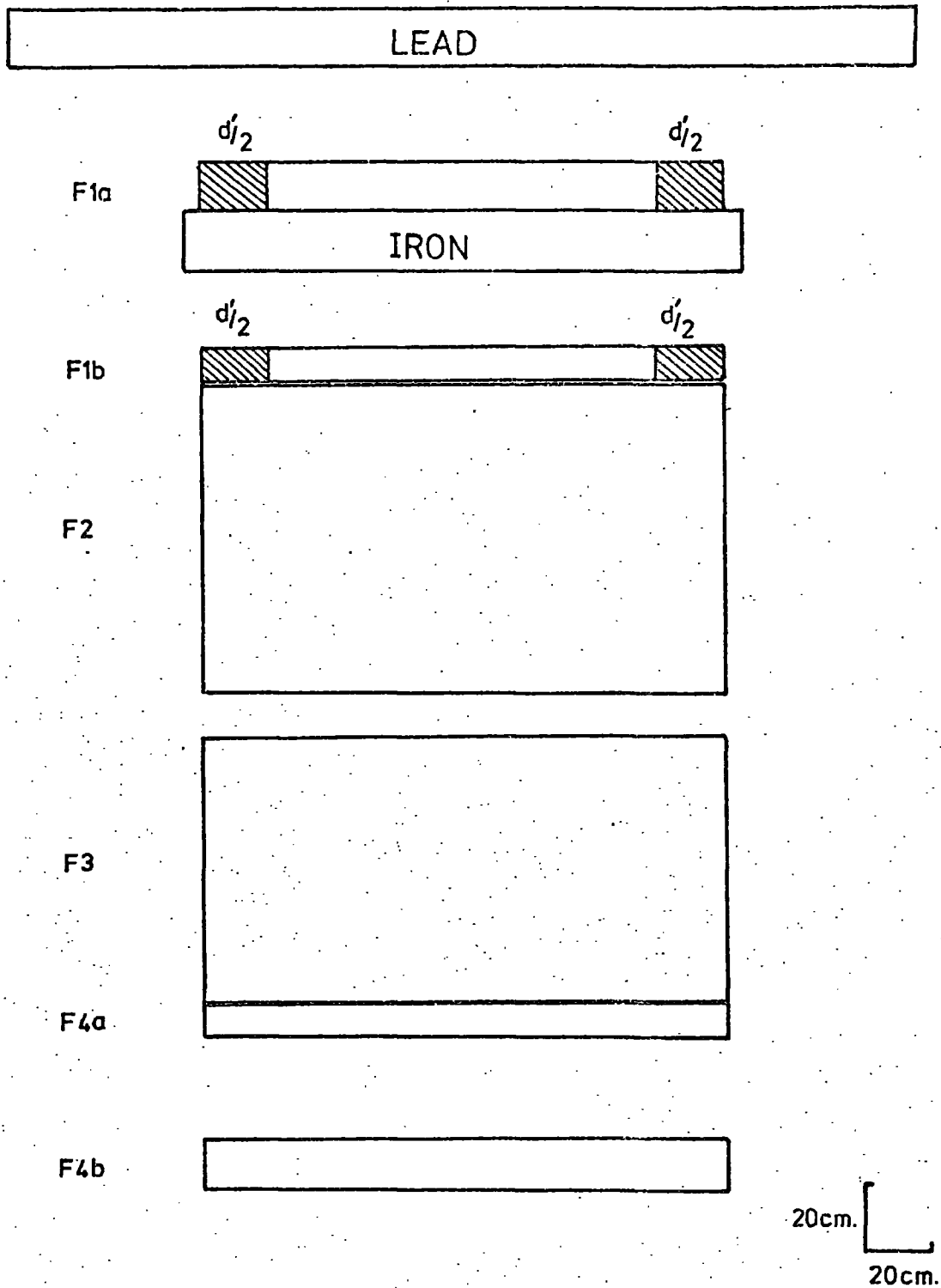
Figure 6.14 Scale diagram of the front of the chamber, showing the restricted acceptance geometry. To be accepted, the core of a burst must lie between, but not in, the shaded areas.
