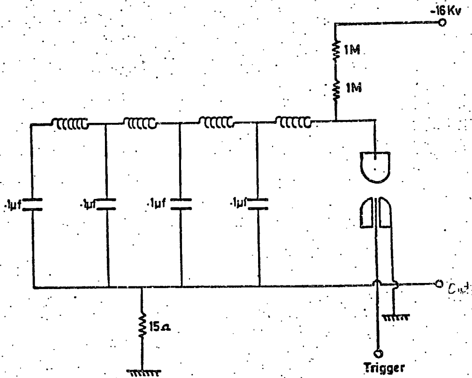
Figure 2.5. Spark gap and delay line
