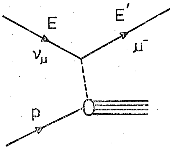
Figure 3.6. Lepton-hadron deep inelastic scattering. (a) represents electron scattering and is an electromagnetic interaction; (b) represents neutrino scattering and occurs via the Fermi(weak) interaction.
