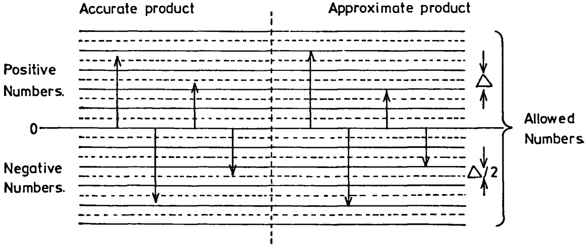
Figure 33 The rounding process
