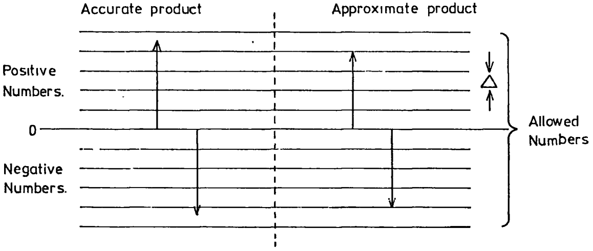
Figure 32 The sign-magnitude truncation process
