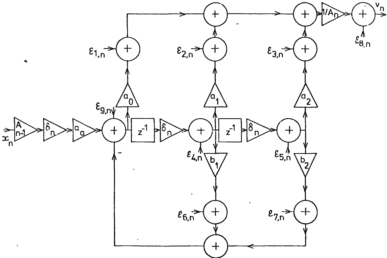
Figure 3.14 An equivalent noise model for a canonic realisation of a second order filter using block-floating-point arithmetic.
