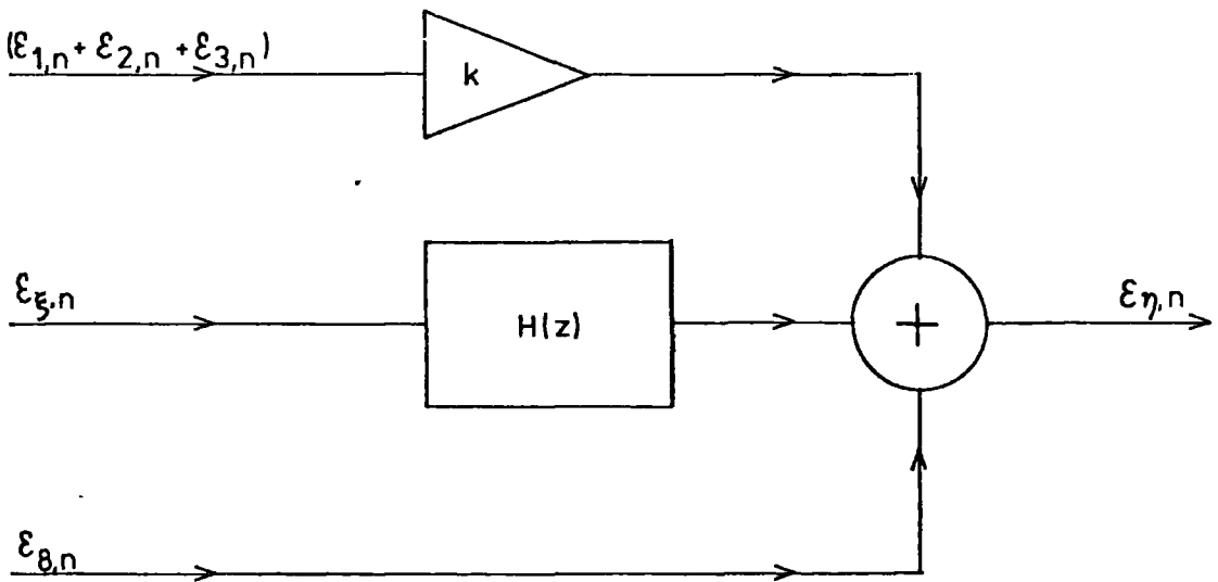
Figure 3.14 An equivalent noise model for a canonic realisation of a second order filter using block-floating-point arithmetic.
