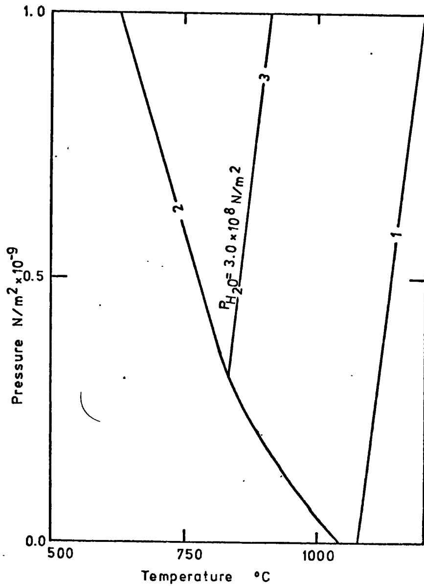
Fig. 2.7 Wet and dry melting curves for basalt (1) Dry basalt (Cohen et al., 1967) (2) Wet basalt (Yoder and Tilley, 1962) (3) Used in this thesis
