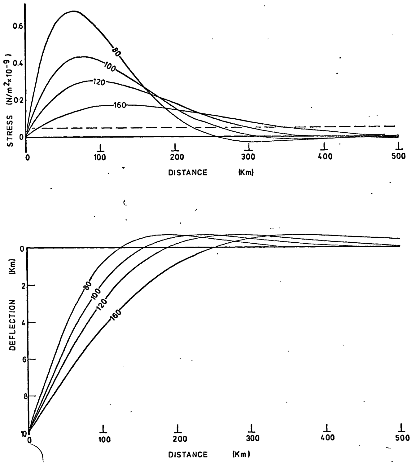
Fig. 5.2 The shape of the deformed plate for various flexural parameters and the stresses induced in the plate 13.5 km from the neutral fibre. If the tensile strength of the crust is 0.5 \times 10^8 \text{ N/m}^2 then failure would occur in the top of the crust at 220 to 350 km from the origin. This is near the top of the deflection for each flexural rigidity.
