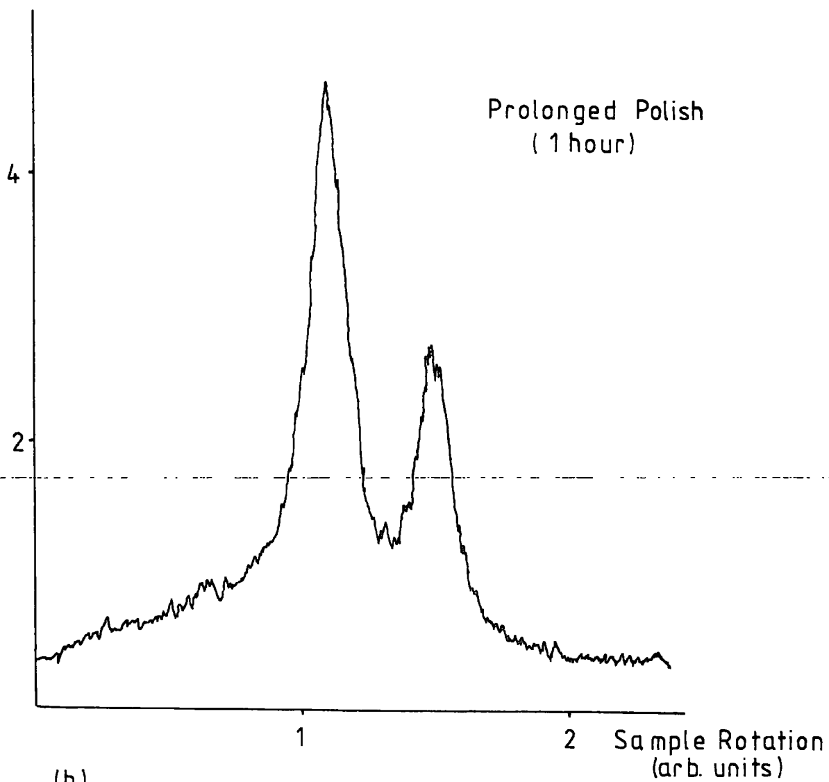
Fig.7.14 Rocking Curves. Effect of Chemical Polishing on Terbium ( 3\bar{1}20 Reflection \text{Cu K}\alpha )
