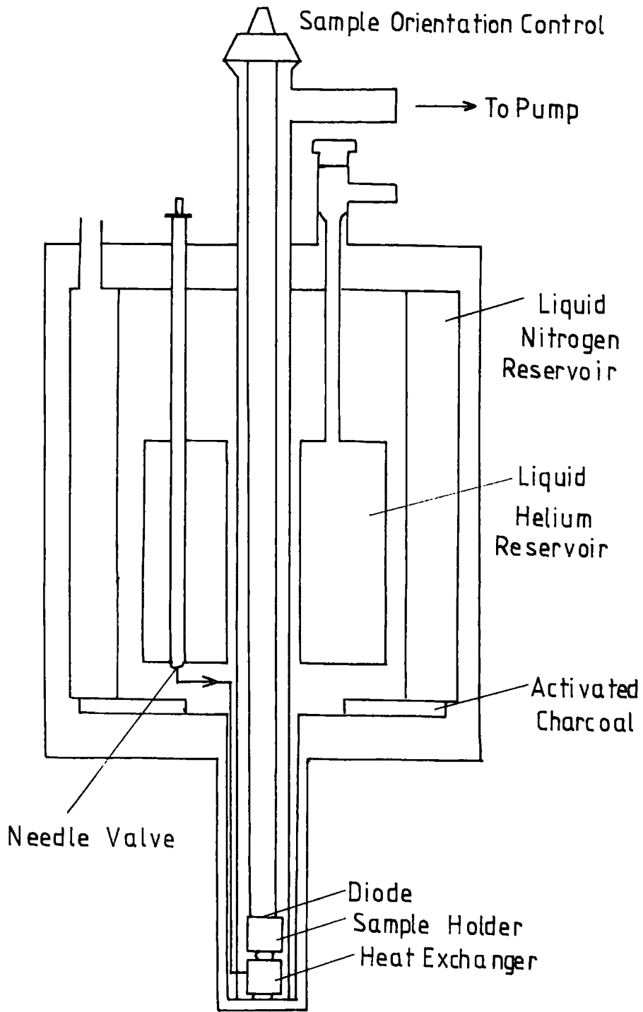
Fig. 2.20 MERIC Cryostat
