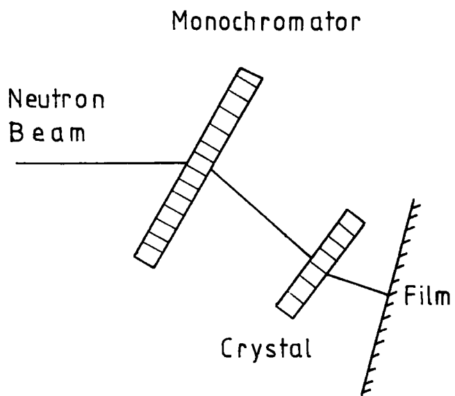
Fig. 5.1 Neutron Topography
