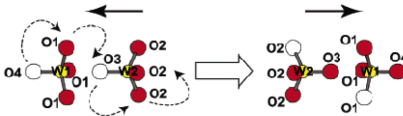
Figure 4-2 Oxygen mobility mechanism responsible for the \alpha to \beta -phase transition in cubic \text{ZrW}_2\text{O}_8 . (5)
