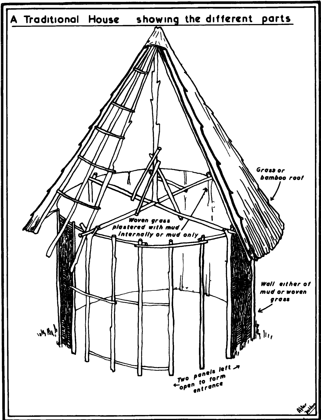
Fig. 9.3. A Traditional Fula Hut Showing the Different Parts.
